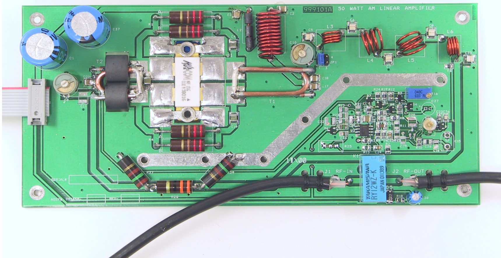
50 watt Amplifier Component Side
