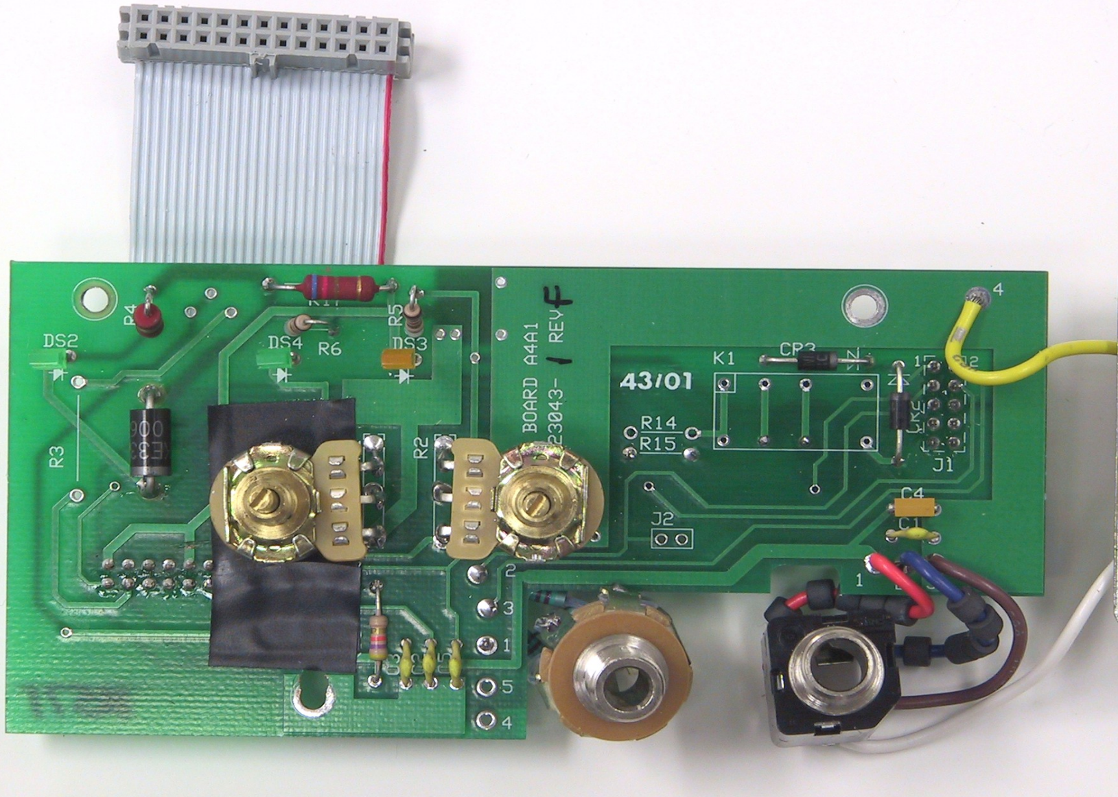
Front Panel
