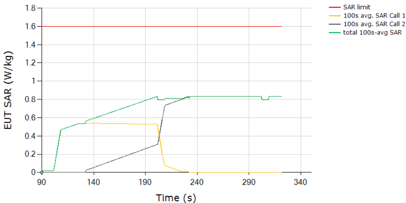
SAR Call Drop Tech: NR5G SUB6, Band 38
