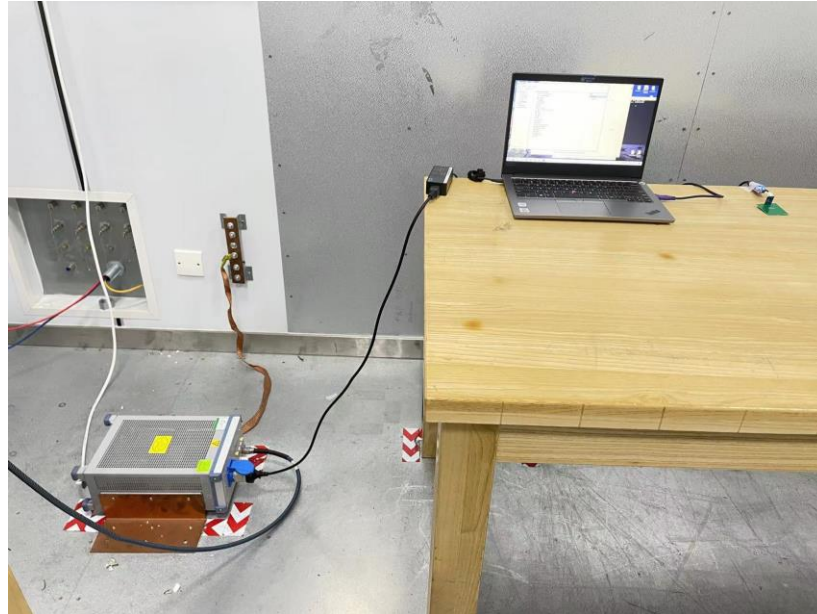
AC POWER LINE CONDUCTED EMISSIONS SETUP
