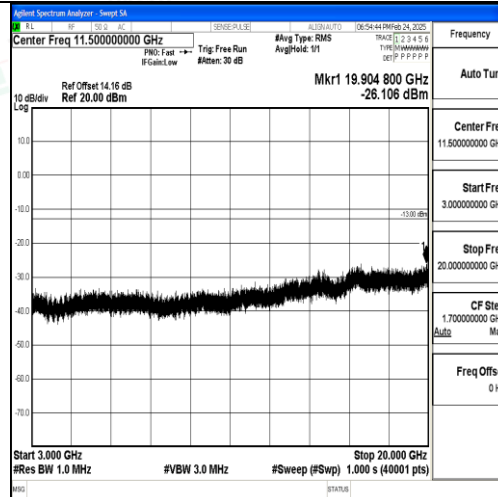
Band2_10MHz_16QAM_18650_1RB#0_3000~20000_3000~20000
