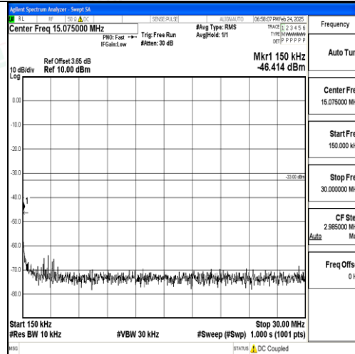
Band2_15MHz_16QAM_18675_1RB#0_0.15~30_0.15~30
