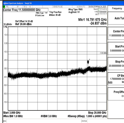
Band2_15MHz_16QAM_18675_1RB#0_3000~20000_3000~20000
