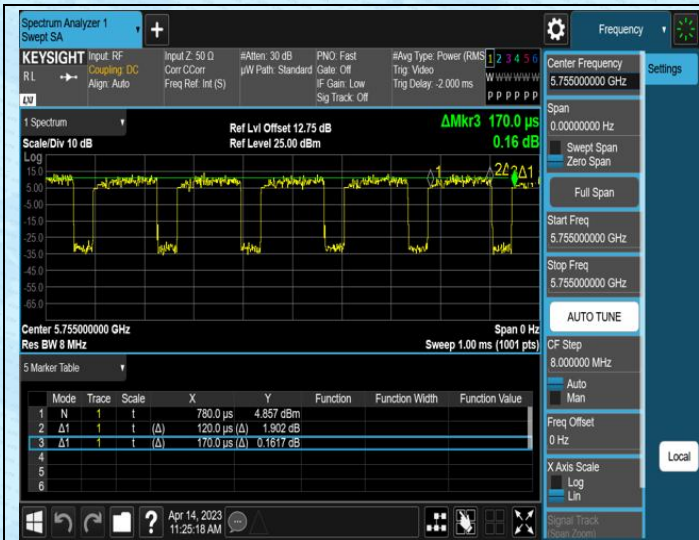
NTNV-11N40SISO-Ant1-5755
