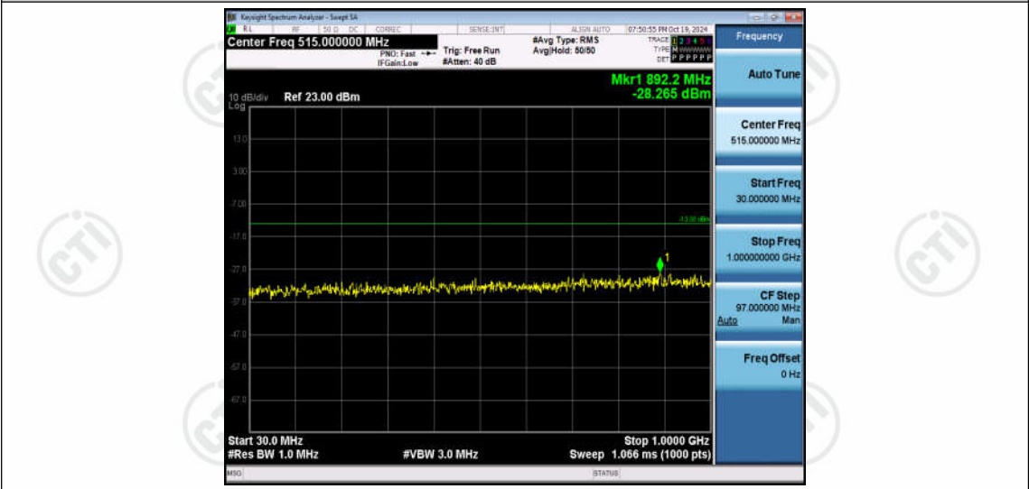
Band66-15MHz-QPSK-132047-1RB#0-Range1:30~1000MHz
