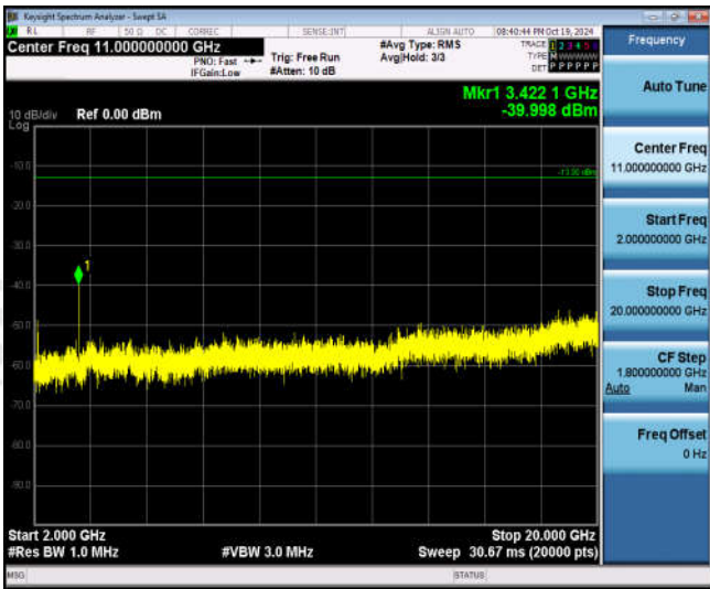
Band66-15MHz-16QAM-132047-1RB#0-Range3:2000~20000MHz
