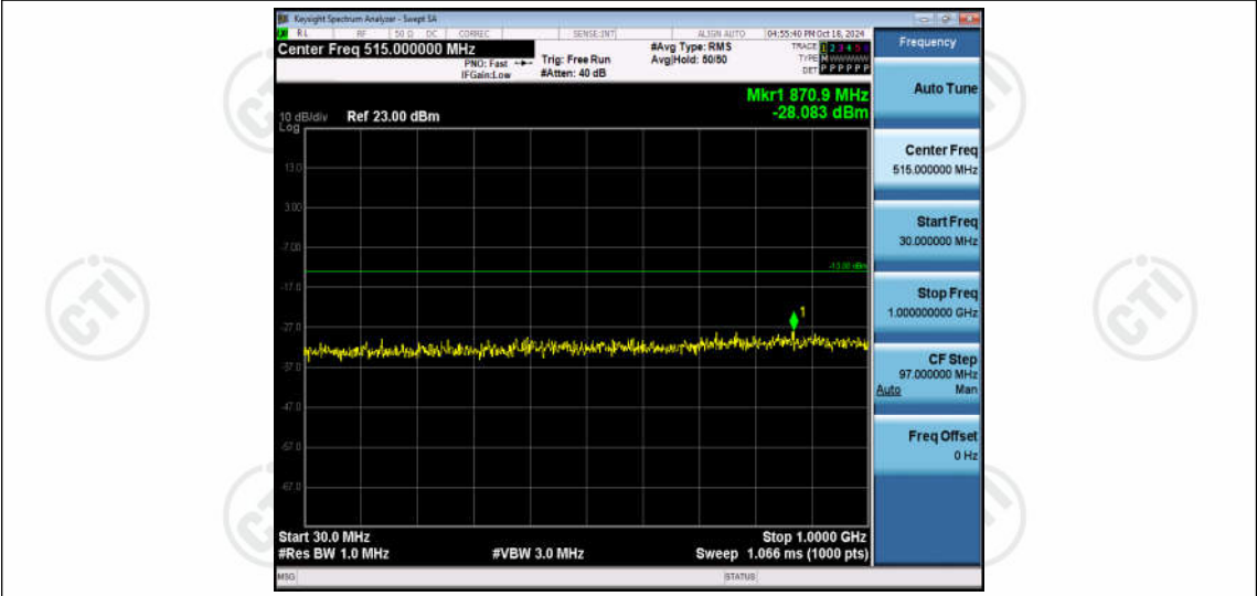
Band66-20MHz-16QAM-132322-1RB#0-Range1:30~1000MHz
