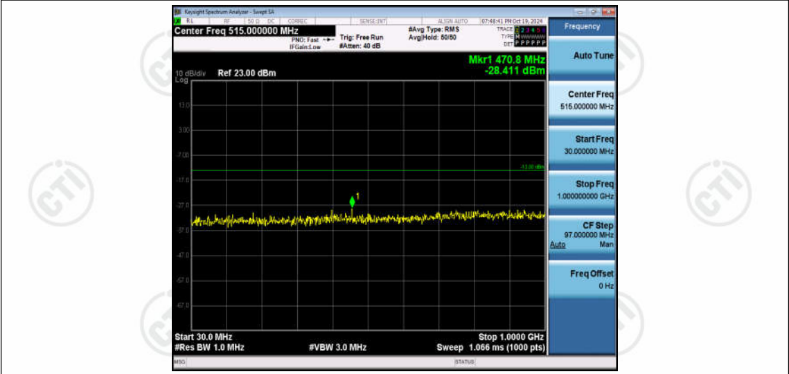
Band66-10MHz-QPSK-132622-1RB#0-Range1:30~1000MHz
