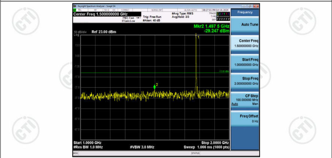
Band66-5MHz-16QAM-132647-1RB#0-Range2:1000~2000MHz
