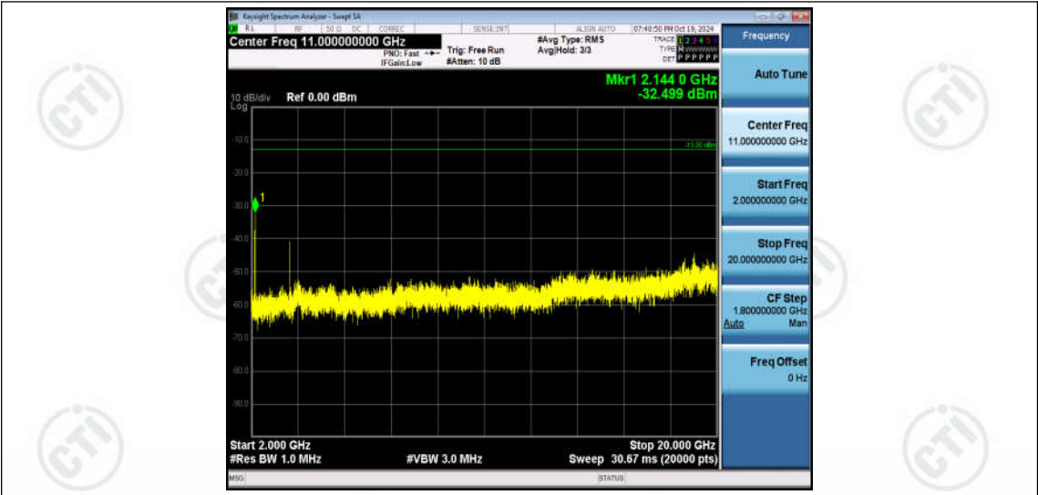
Band66-5MHz-QPSK-132322-1RB#0-Range3:2000~20000MHz
