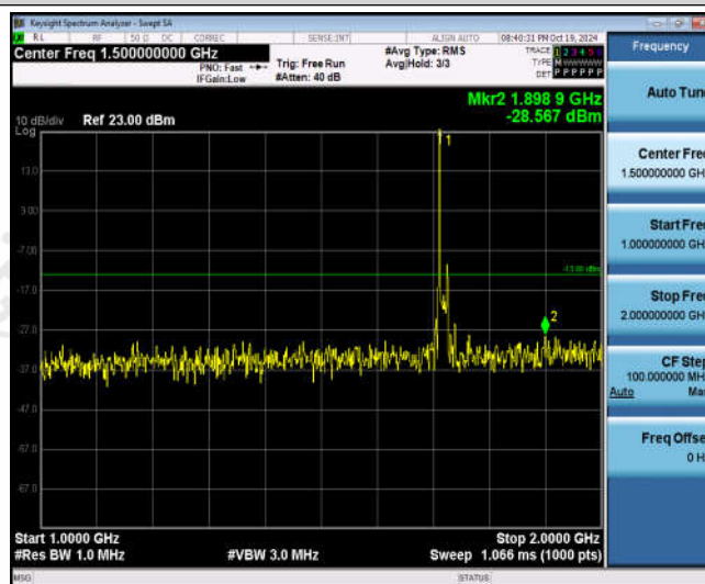
Band66-15MHz-16QAM-132047-1RB#0-Range2:1000~2000MHz
