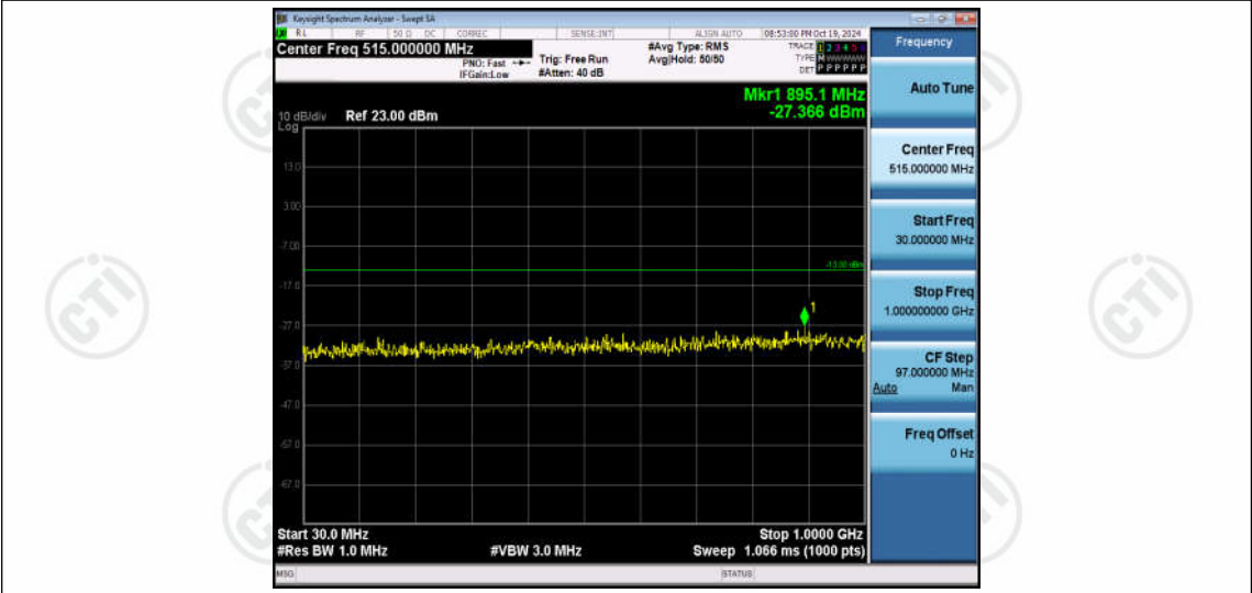
Band66-20MHz-16QAM-132072-1RB#0-Range1:30~1000MHz
