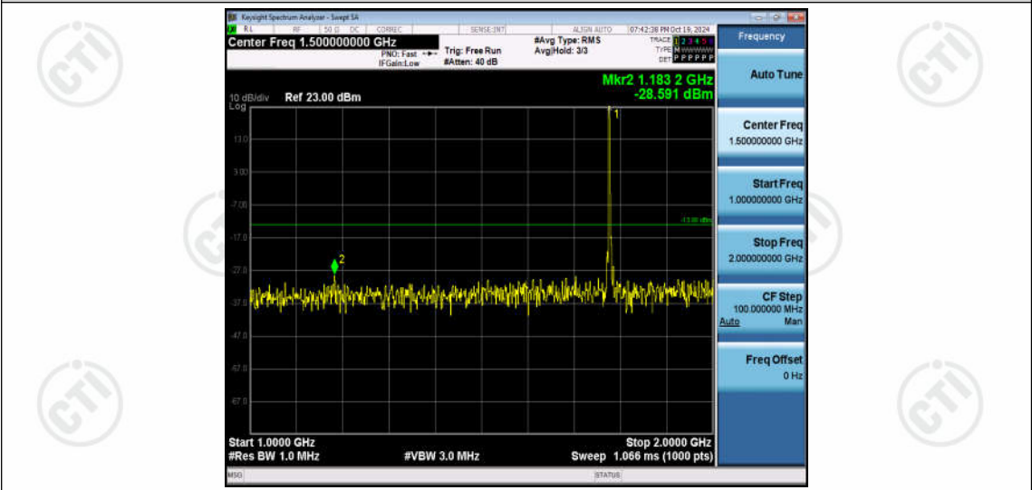
Band66-5MHz-QPSK-132647-1RB#0-Range2:1000~2000MHz
