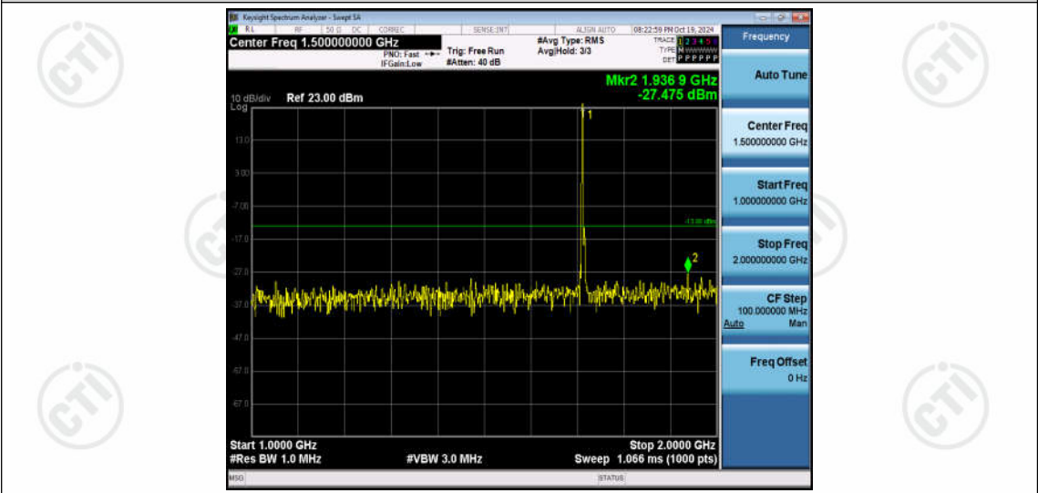
Band66-5MHz-16QAM-131997-1RB#0-Range2:1000~2000MHz
