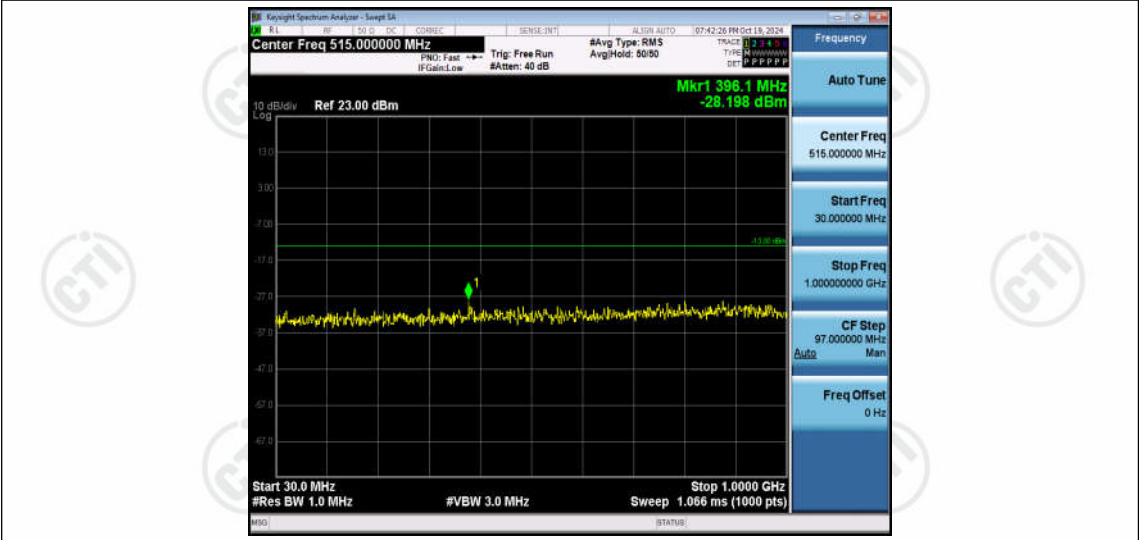
Band66-5MHz-QPSK-132647-1RB#0-Range1:30~1000MHz
