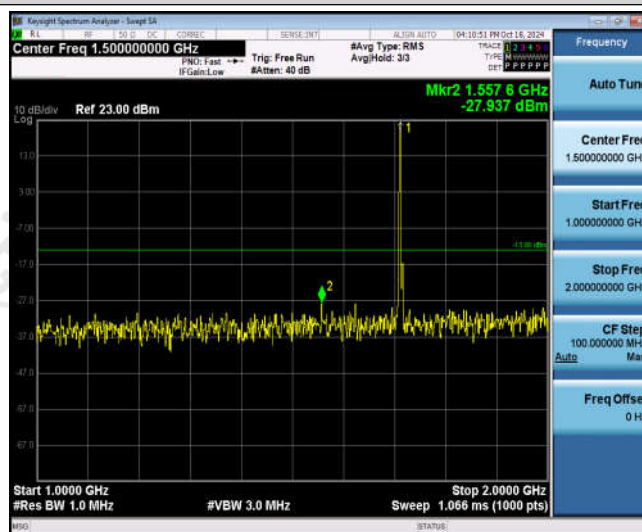
Band66-3MHz-16QAM-131987-1RB#0-Range2:1000~2000MHz
