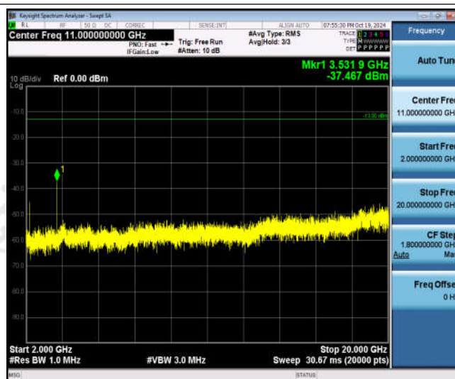
Band66-15MHz-QPSK-132597-1RB#0-Range3:2000~20000MHz
