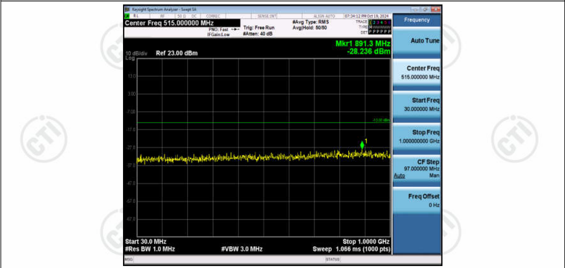
Band66-3MHz-QPSK-132322-1RB#0-Range1:30~1000MHz
