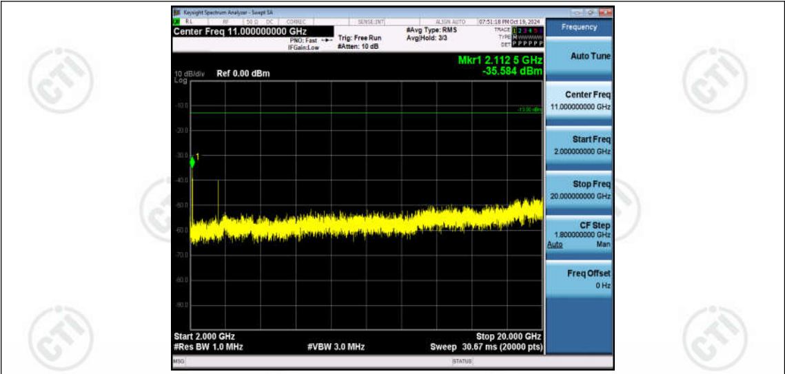
Band66-15MHz-QPSK-132047-1RB#0-Range3:2000~20000MHz
