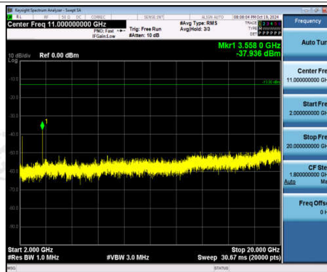
Band66-1.4MHz-16QAM-132665-1RB#0-Range3:2000~20000MHz
