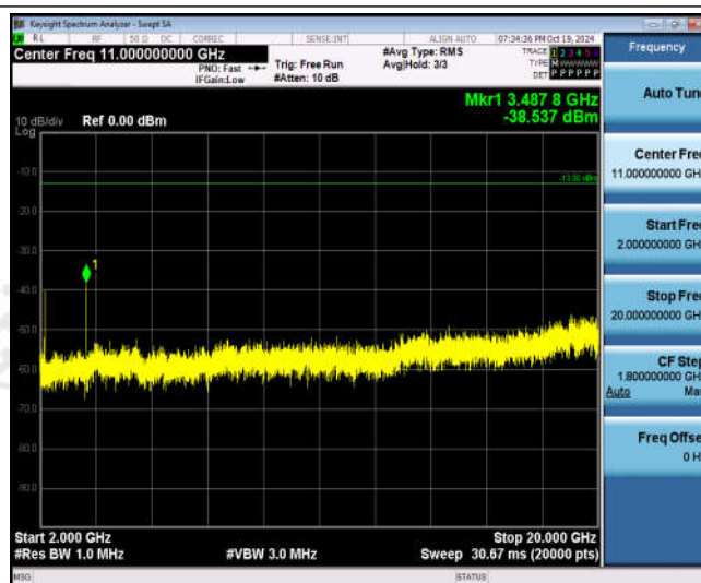
Band66-3MHz-QPSK-132322-1RB#0-Range3:2000~20000MHz
