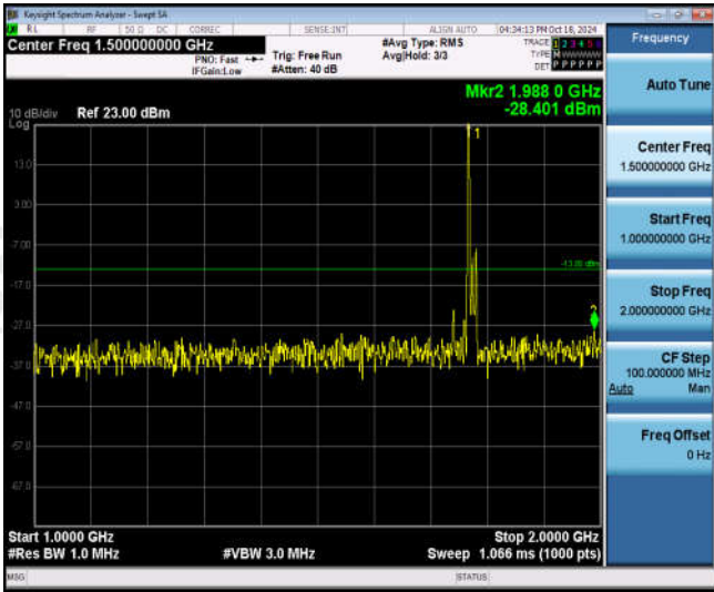
Band66-15MHz-16QAM-132597-1RB#0-Range2:1000~2000MHz
