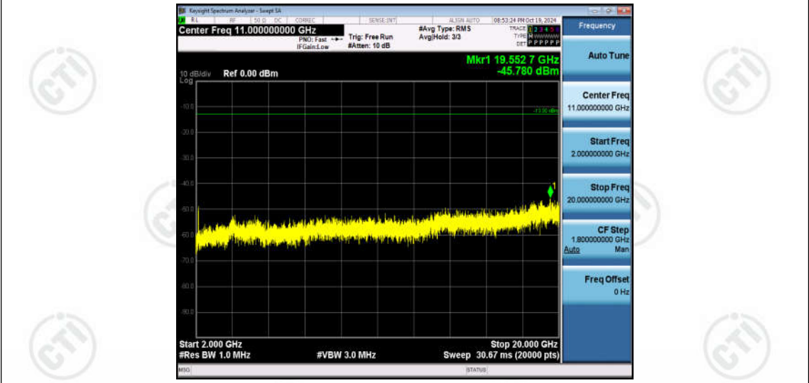
Band66-20MHz-16QAM-132072-1RB#0-Range3:2000~20000MHz
