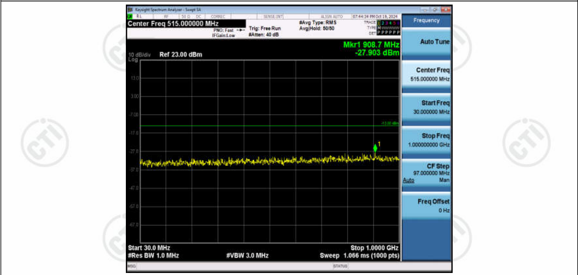
Band66-10MHz-QPSK-132022-1RB#0-Range1:30~1000MHz
