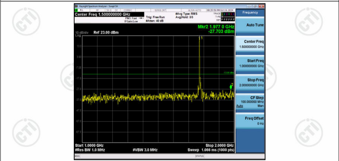
Band66-10MHz-16QAM-132622-1RB#0-Range2:1000~2000MHz
