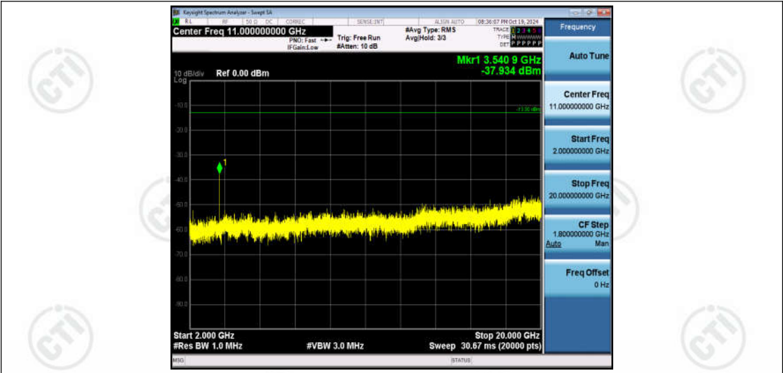
Band66-10MHz-16QAM-132622-1RB#0-Range3:2000~20000MHz
