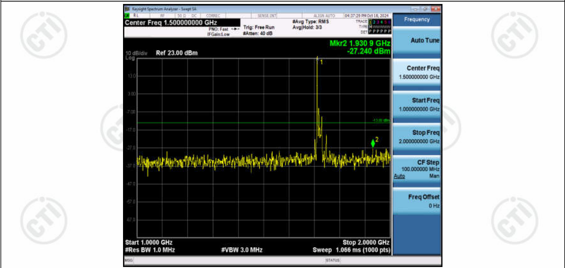
Band66-20MHz-16QAM-132072-1RB#0-Range2:1000~2000MHz
