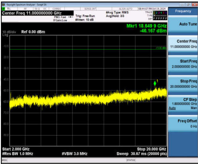
Band66-15MHz-16QAM-132322-1RB#0-Range3:2000~20000MHz
