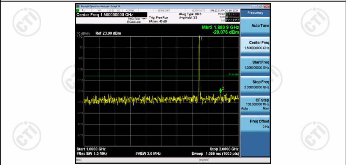
Band66-5MHz-16QAM-132322-1RB#0-Range2: 1000~2000MHz
