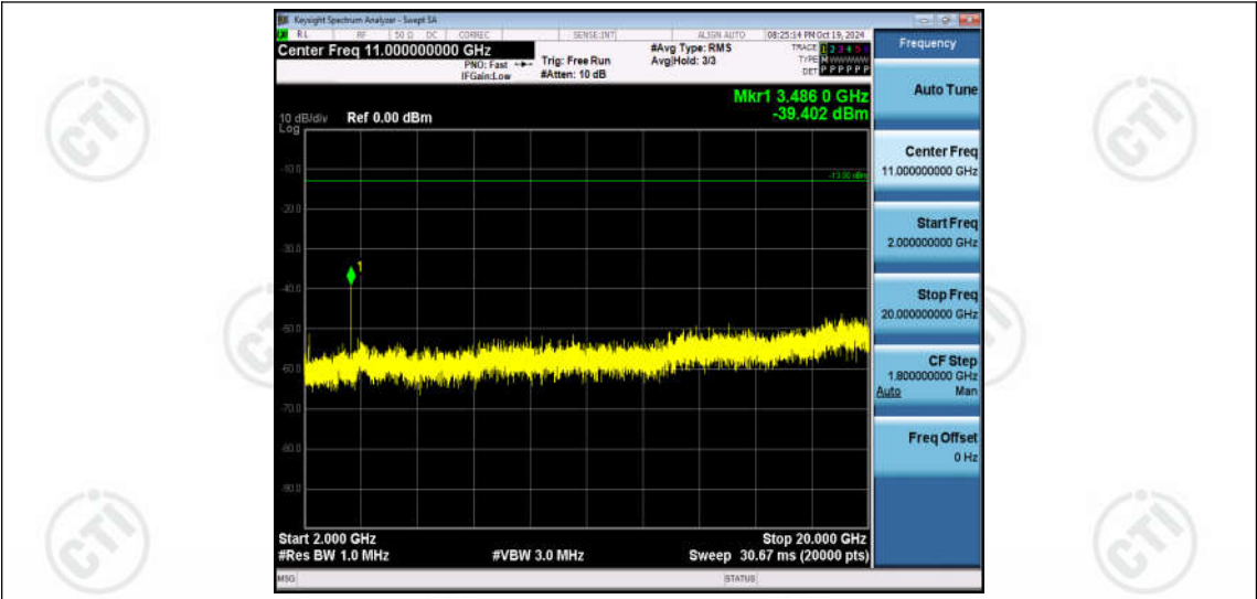
Band66-5MHz-16QAM-132322-1RB#0-Range3:2000~20000MHz
