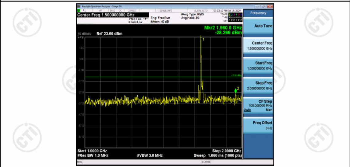
Band66-15MHz-QPSK-132322-1RB#0-Range2:1000~2000MHz
