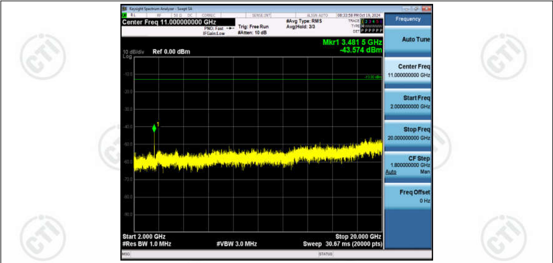
Band66-10MHz-16QAM-132322-1RB#0-Range3:2000~20000MHz
