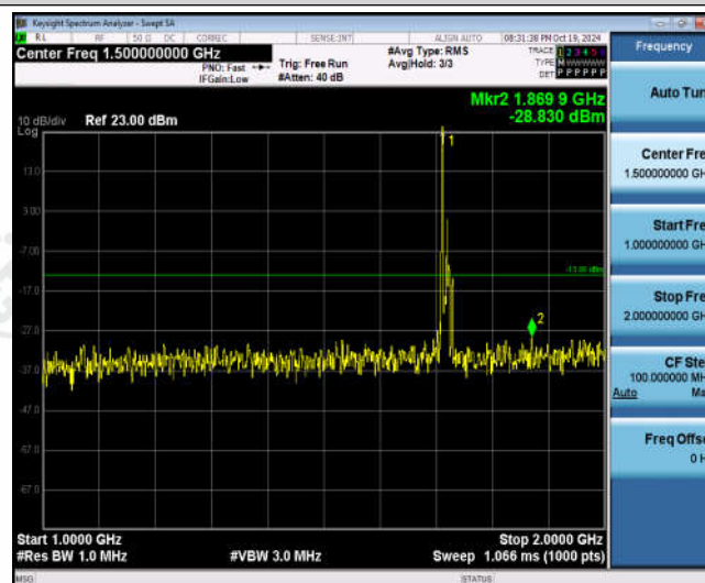
Band66-10MHz-16QAM-132022-1RB#0-Range2:1000~2000MHz
