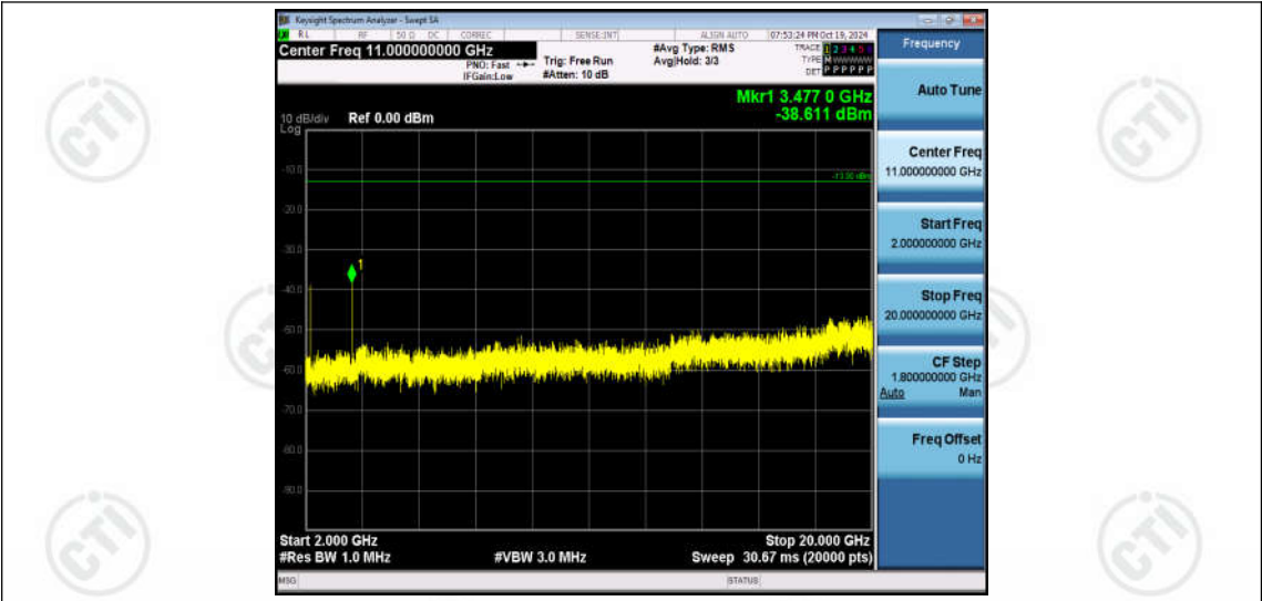
Band66-15MHz-QPSK-132322-1RB#0-Range3:2000~20000MHz
