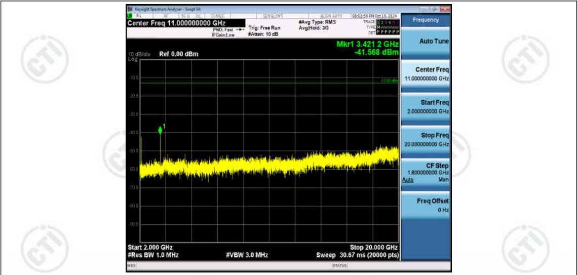
Band66-1.4MHz-16QAM-131979-1RB#0-Range3:2000~20000MHz
