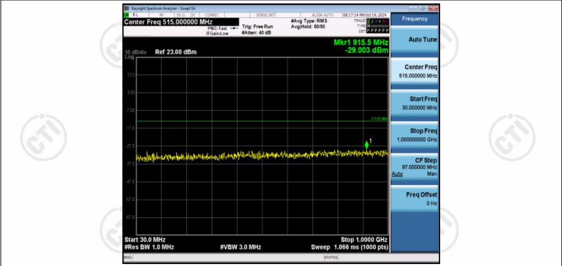
Band66-3MHz-16QAM-132322-1RB#0-Range1:30~1000MHz
