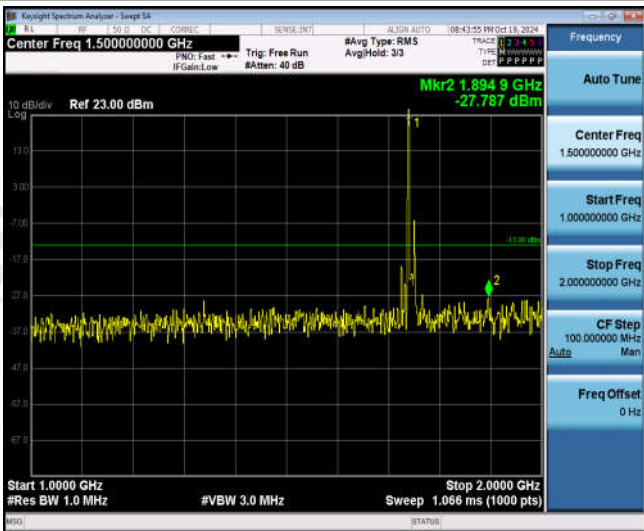
Band66-15MHz-16QAM-132322-1RB#0-Range2:1000~2000MHz
