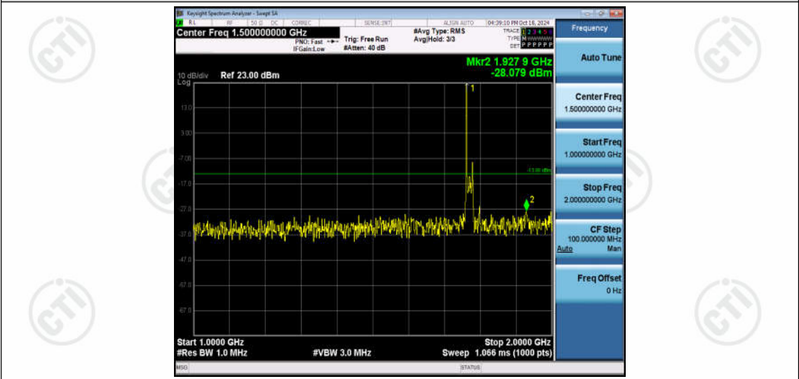
Band66-20MHz-16QAM-132572-1RB#0-Range2:1000~2000MHz
