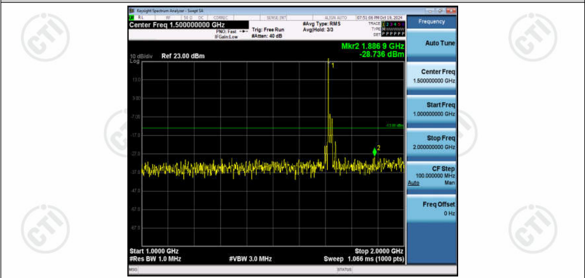
Band66-15MHz-QPSK-132047-1RB#0-Range2:1000~2000MHz
