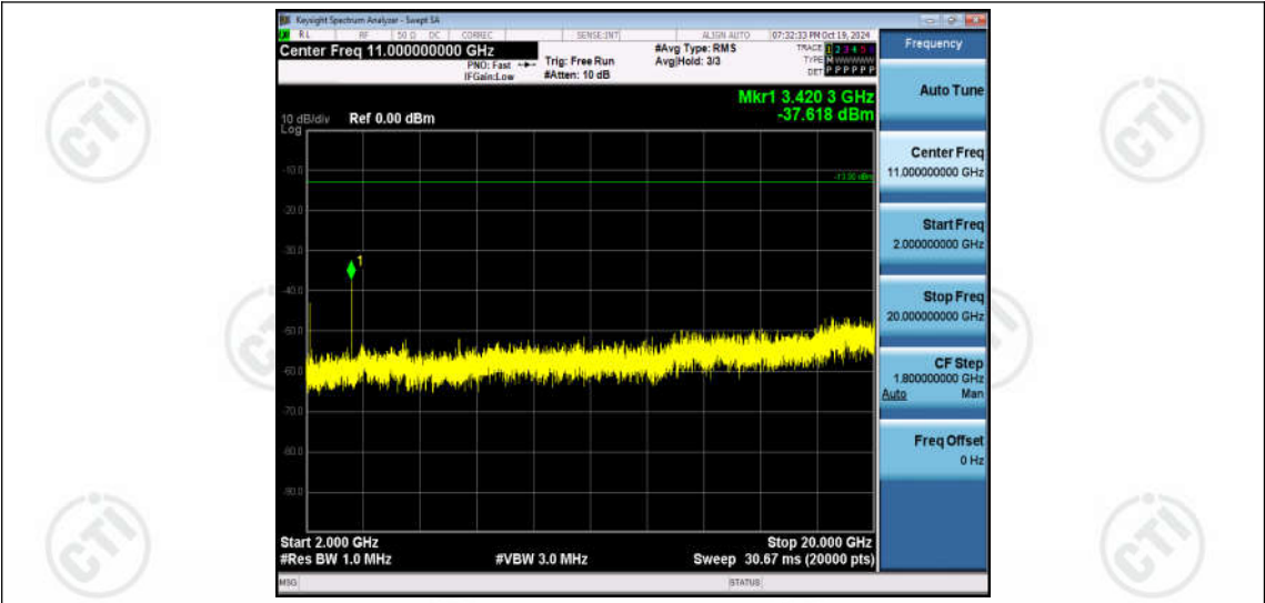
Band66-3MHz-QPSK-131987-1RB#0-Range3:2000~20000MHz
