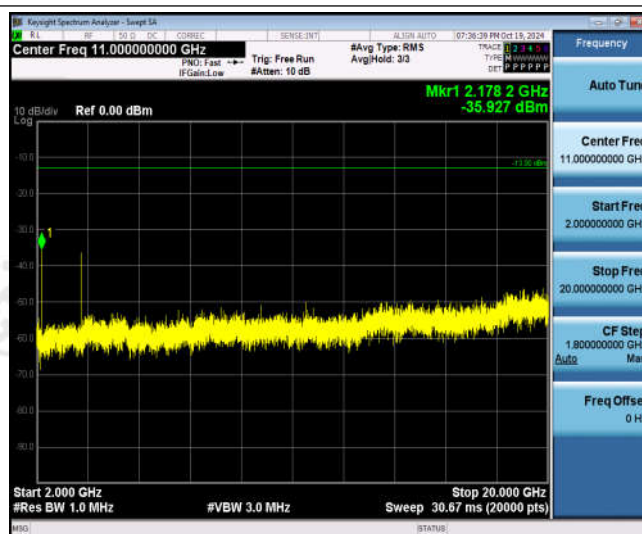
Band66-3MHz-QPSK-132657-1RB#0-Range3:2000~20000MHz
