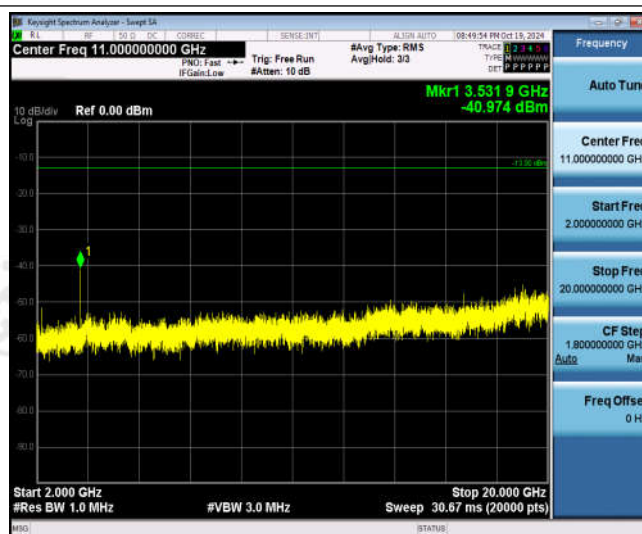
Band66-15MHz-16QAM-132597-1RB#0-Range3:2000~20000MHz
