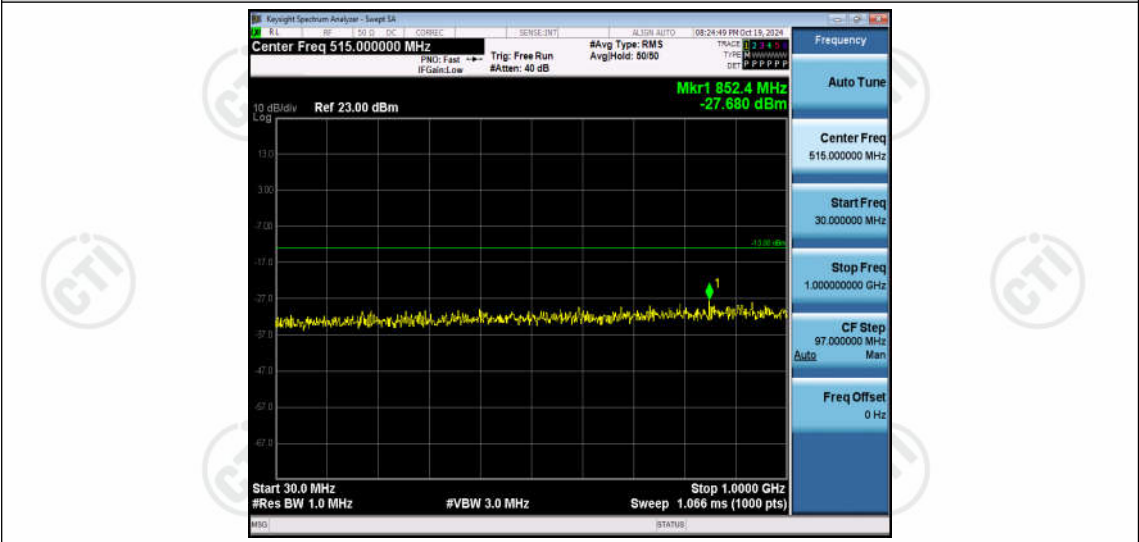
Band66-5MHz-16QAM-132322-1RB#0-Range1:30~1000MHz
