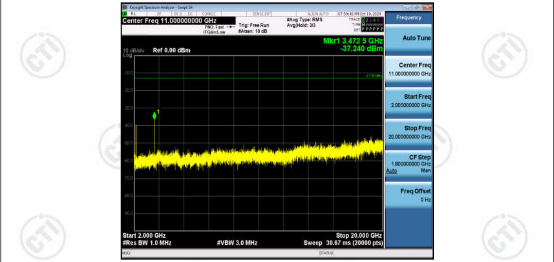
Band66-20MHz-QPSK-132322-1RB#0-Range3:2000~20000MHz
