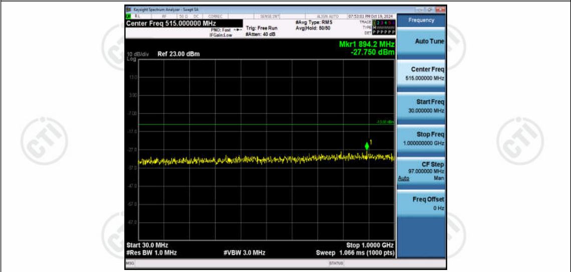
Band66-15MHz-QPSK-132322-1RB#0-Range1:30~1000MHz
