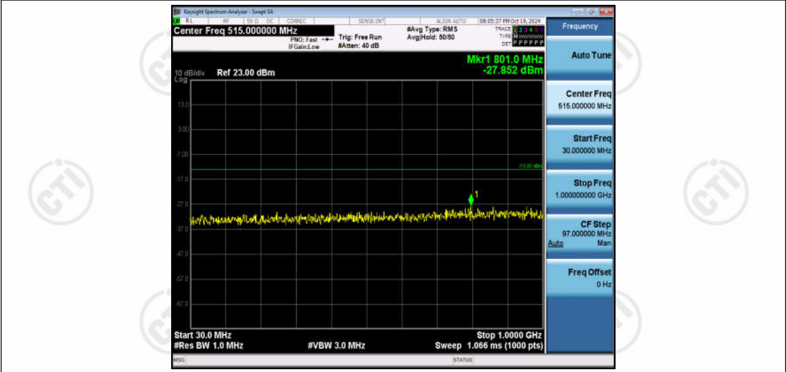
Band66-1.4MHz-16QAM-132322-1RB#0-Range1:30~1000MHz
