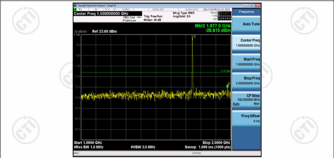
Band66-3MHz-16QAM-132322-1RB#0-Range2: 1000~2000MHz
