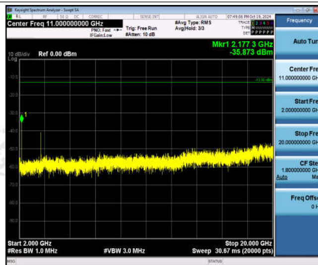
Band66-10MHz-QPSK-132622-1RB#0-Range3:2000~20000MHz
