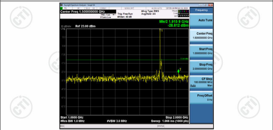
Band66-15MHz-QPSK-132597-1RB#0-Range2:1000~2000MHz
