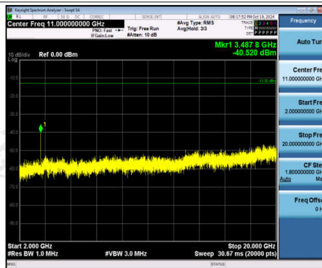
Band66-3MHz-16QAM-132322-1RB#0-Range3:2000~20000MHz
