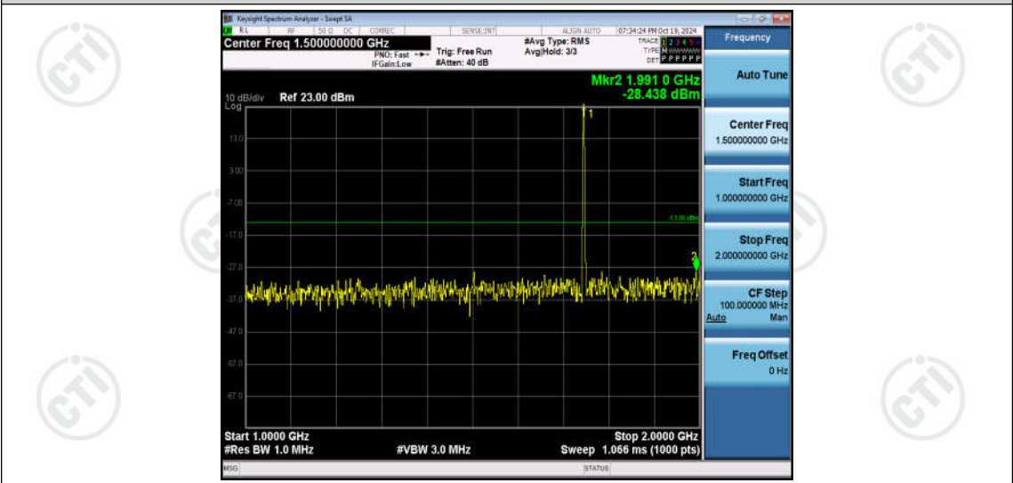
Band66-3MHz-QPSK-132322-1RB#0-Range2:1000~2000MHz
