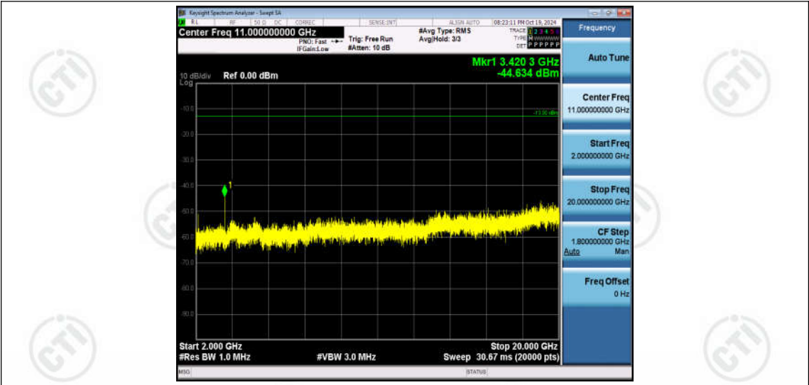
Band66-5MHz-16QAM-131997-1RB#0-Range3:2000~20000MHz
