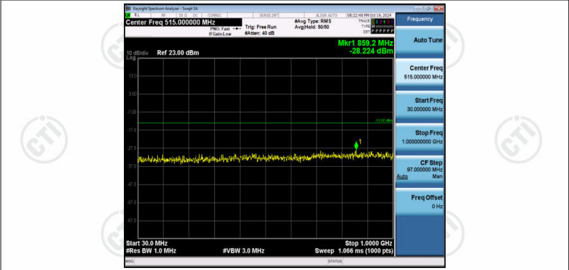
Band66-5MHz-16QAM-131997-1RB#0-Range1:30~1000MHz
