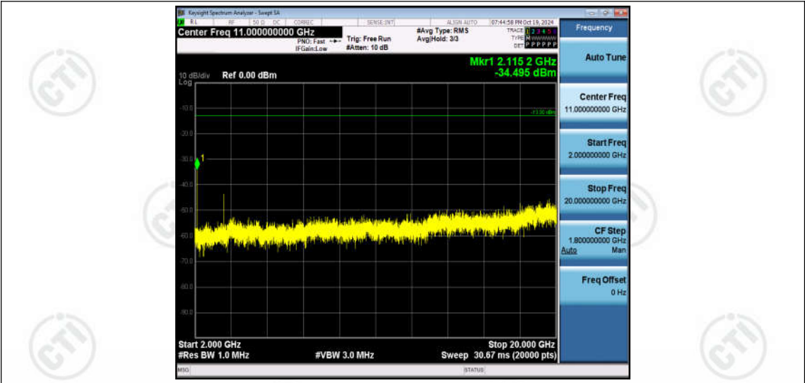
Band66-10MHz-QPSK-132022-1RB#0-Range3:2000~20000MHz
