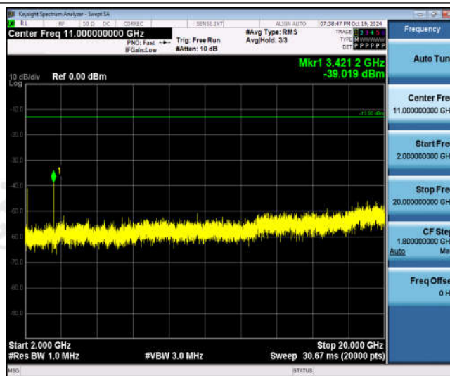
Band66-5MHz-QPSK-131997-1RB#0-Range3:2000~20000MHz
