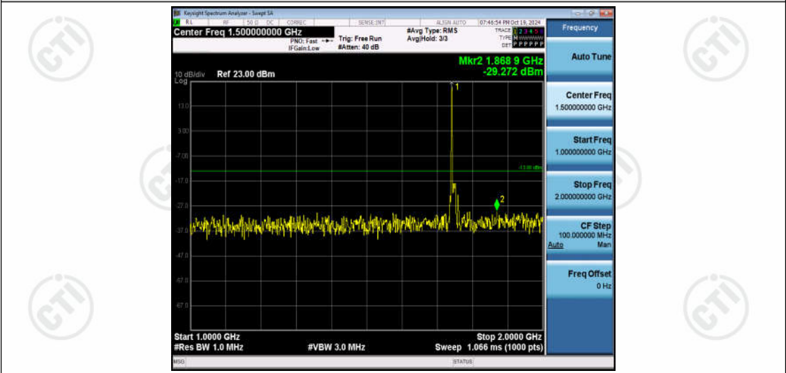
Band66-10MHz-QPSK-132322-1RB#0-Range2:1000~2000MHz
