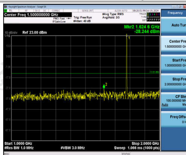
Band66-3MHz-16QAM-132657-1RB#0-Range2:1000~2000MHz
