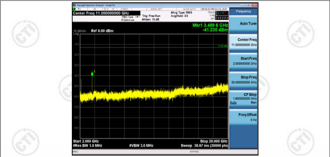
Band66-1.4MHz-16QAM-132322-1RB#0-Range3:2000~20000MHz
