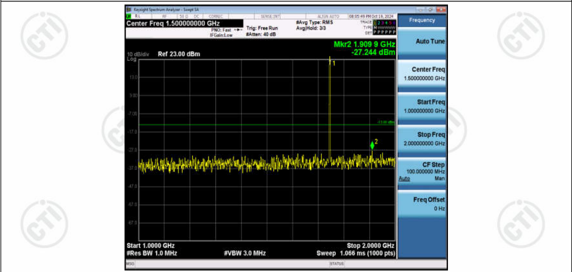
Band66-1.4MHz-16QAM-132322-1RB#0-Range2:1000~2000MHz
