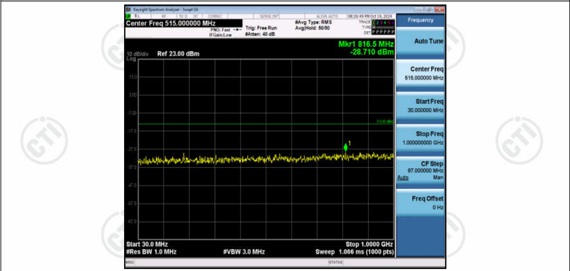
Band66-5MHz-16QAM-132647-1RB#0-Range1:30~1000MHz
