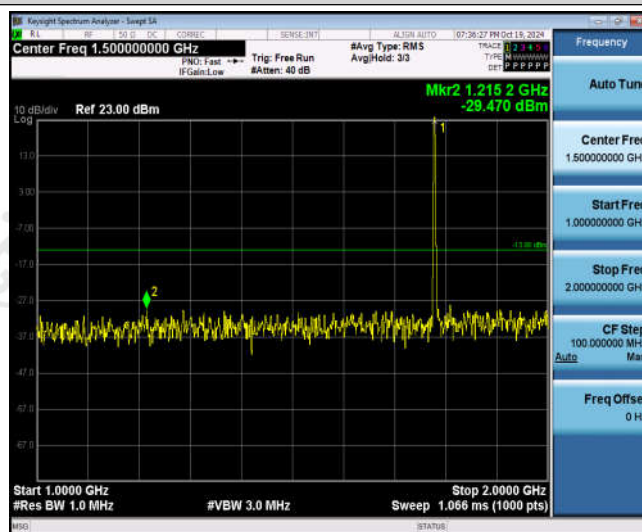
Band66-3MHz-QPSK-132657-1RB#0-Range2:1000~2000MHz
