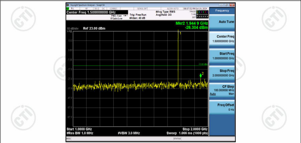
Band66-1.4MHz-16QAM-132665-1RB#0-Range2:1000~2000MHz
