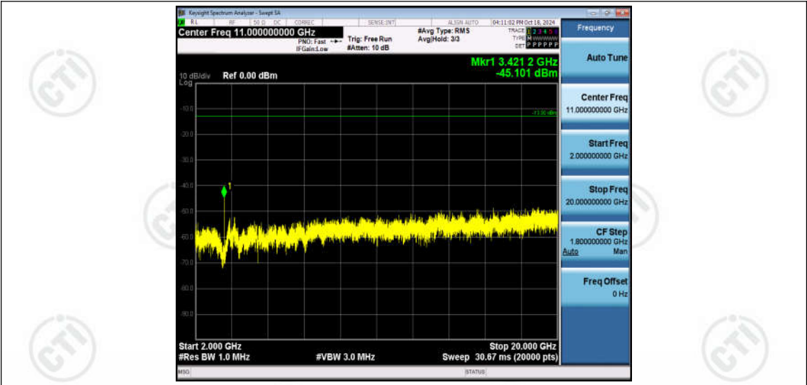
Band66-3MHz-16QAM-131987-1RB#0-Range3:2000~20000MHz
