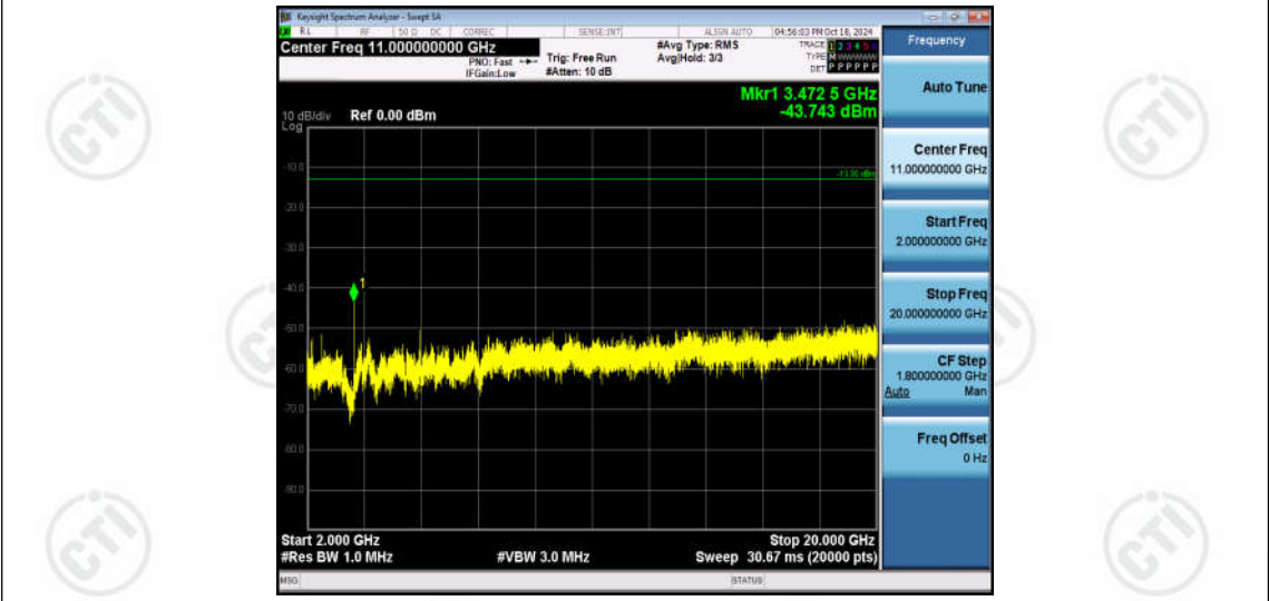
Band66-20MHz-16QAM-132322-1RB#0-Range3:2000~20000MHz
