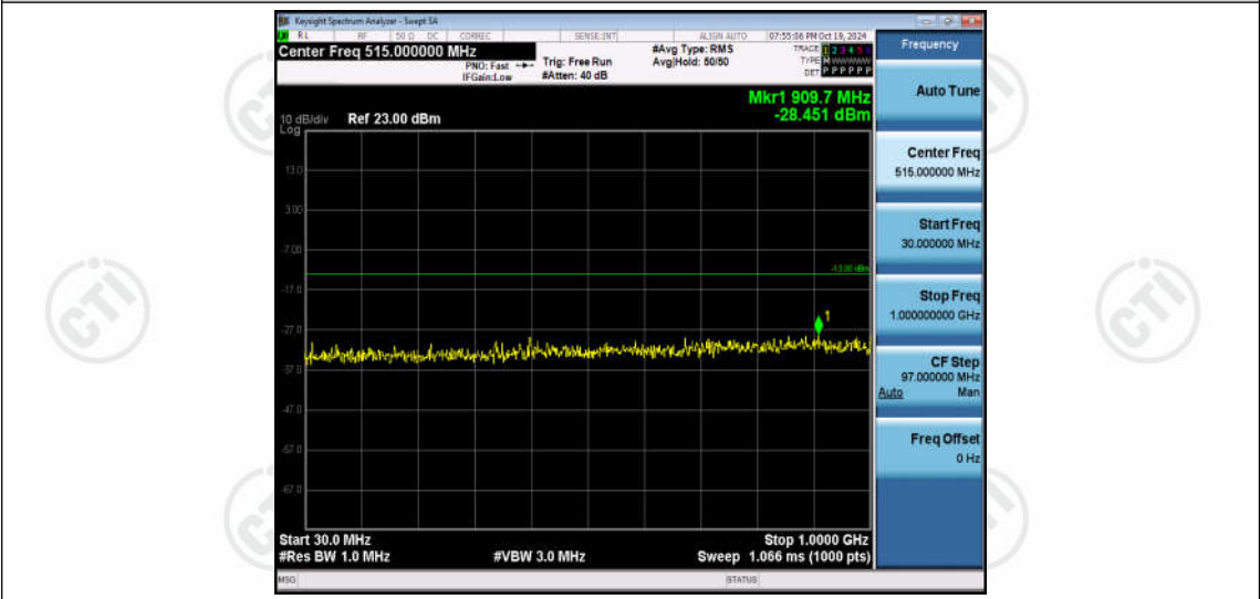
Band66-15MHz-QPSK-132597-1RB#0-Range1:30~1000MHz
