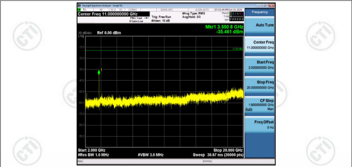
Band66-5MHz-QPSK-132647-1RB#0-Range3:2000~20000MHz
