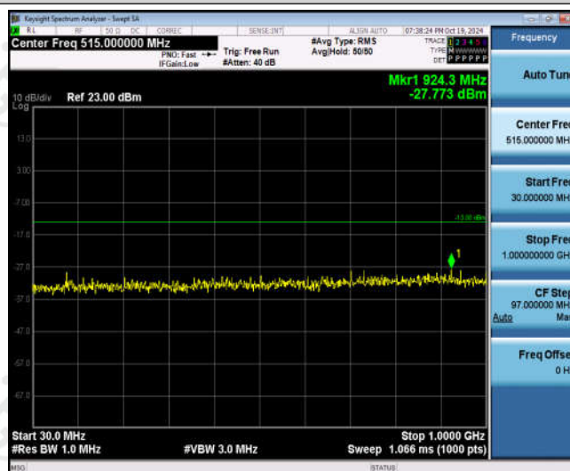
Band66-5MHz-QPSK-131997-1RB#0-Range1:30~1000MHz
