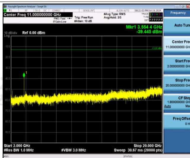
Band66-3MHz-16QAM-132657-1RB#0-Range3:2000~20000MHz
