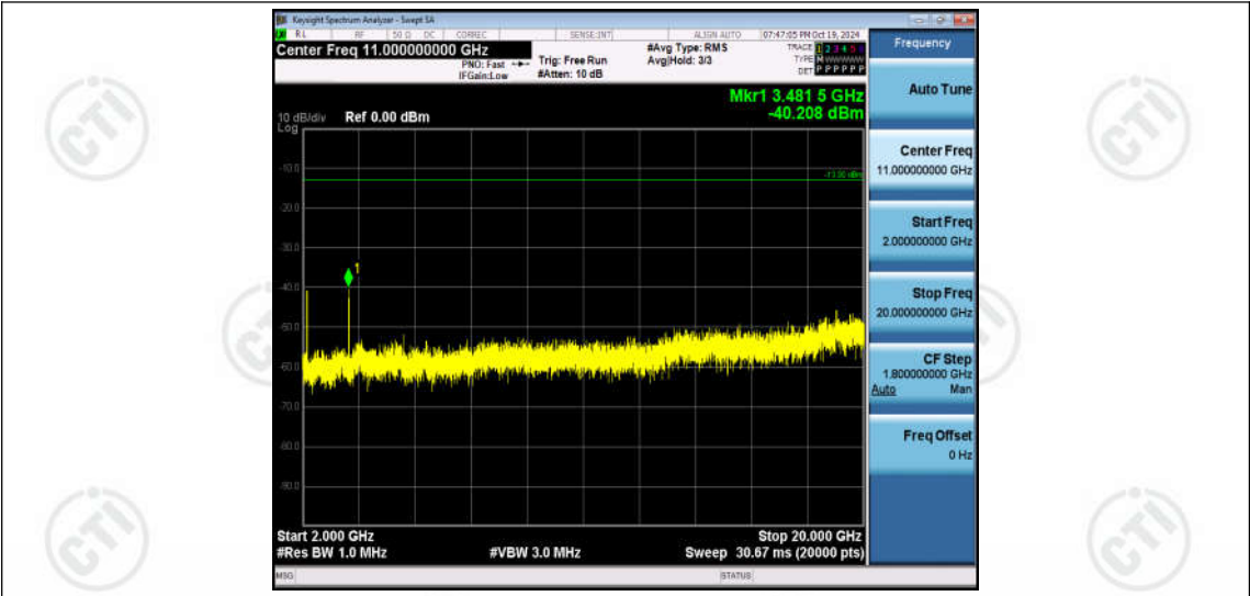
Band66-10MHz-QPSK-132322-1RB#0-Range3:2000~20000MHz
