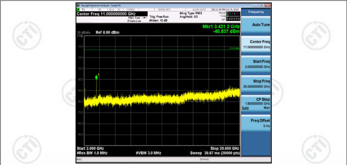
Band66-10MHz-16QAM-132022-1RB#0-Range3:2000~20000MHz
