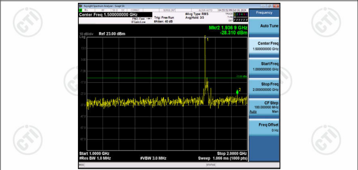
Band66-20MHz-16QAM-132322-1RB#0-Range2:1000~2000MHz
