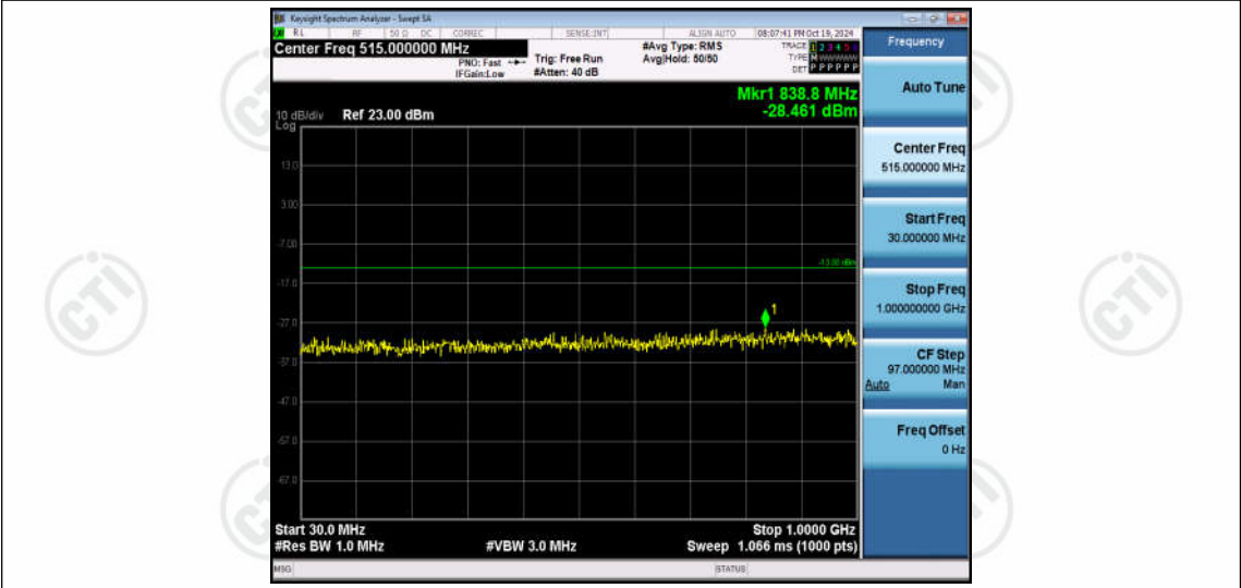
Band66-1.4MHz-16QAM-132665-1RB#0-Range1:30~1000MHz
