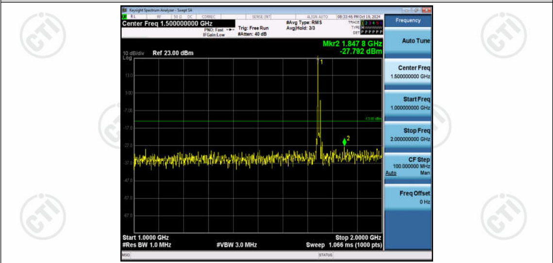
Band66-10MHz-16QAM-132322-1RB#0-Range2:1000~2000MHz
