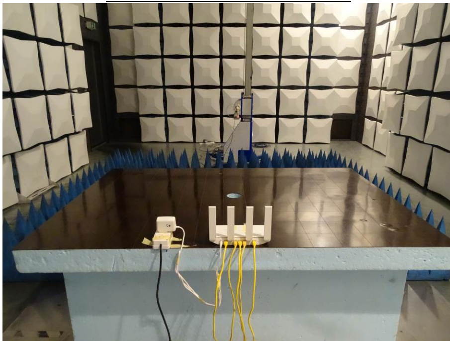
Radiated Disturbance (18GHz-26.5GHz)
