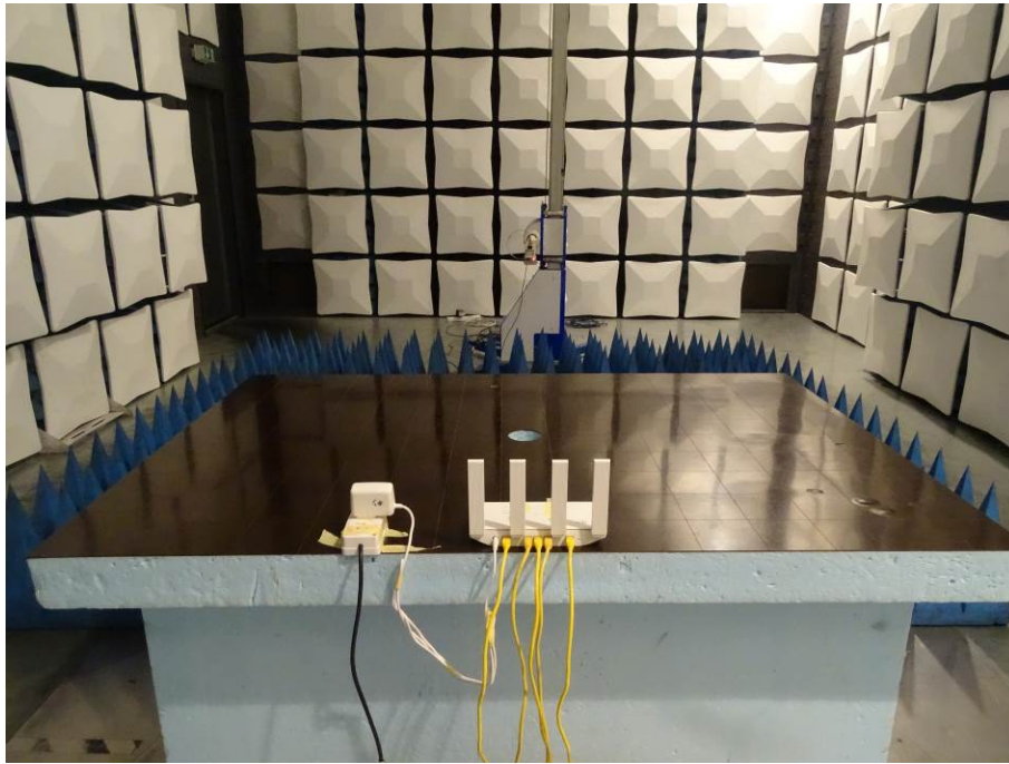
Radiated Disturbance (26.5GHz-40GHz)
