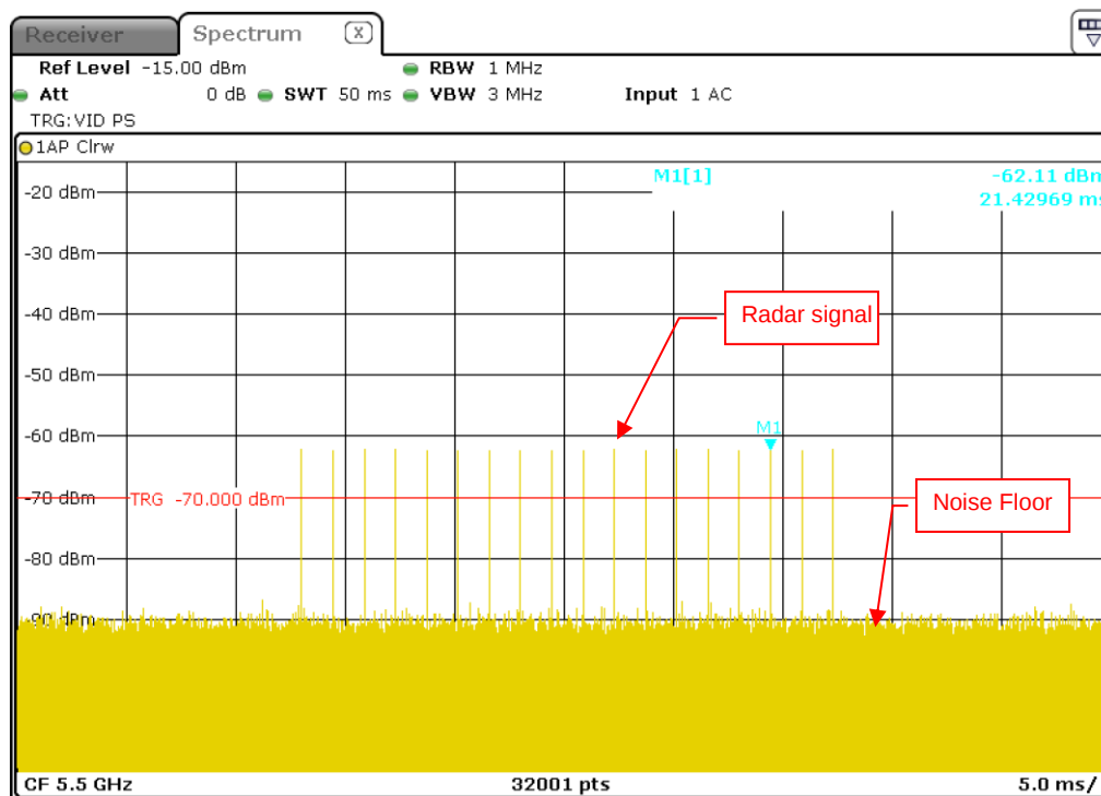
Radar Signal 0
