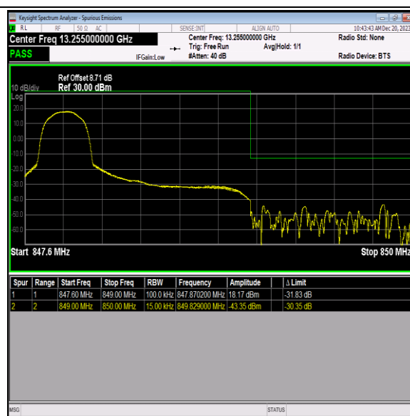
Band5_1.4MHz_16QAM_20643_1RB#0
