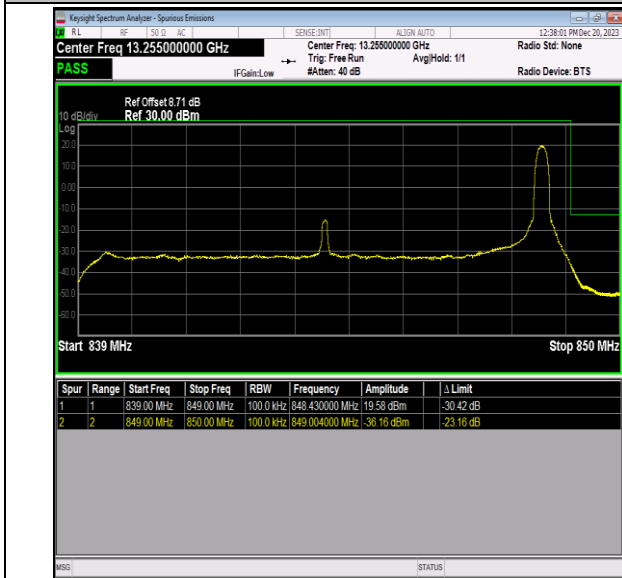
Band5_10MHz_QPSK_20600_1RB#49
