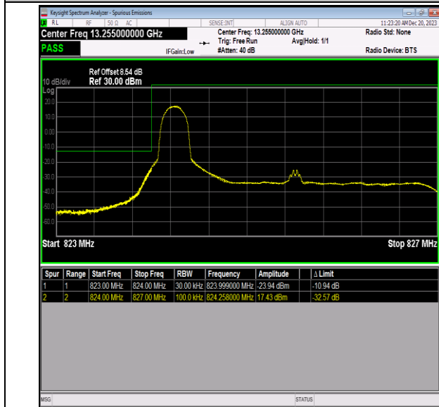
Band5_3MHz_64QAM_20415_1RB#0
