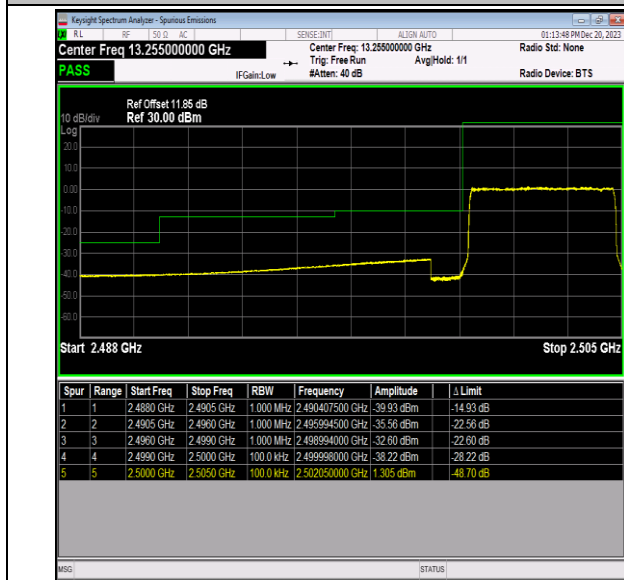
Band7_5MHz_64QAM_20775_25RB#0
