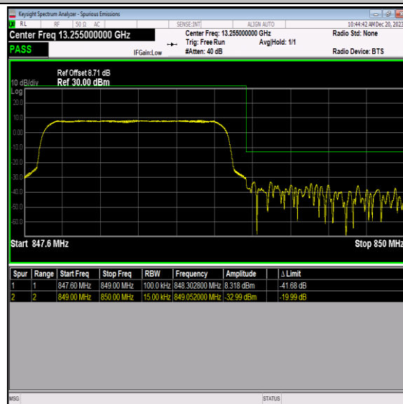
Band5_1.4MHz_16QAM_20643_6RB#0
