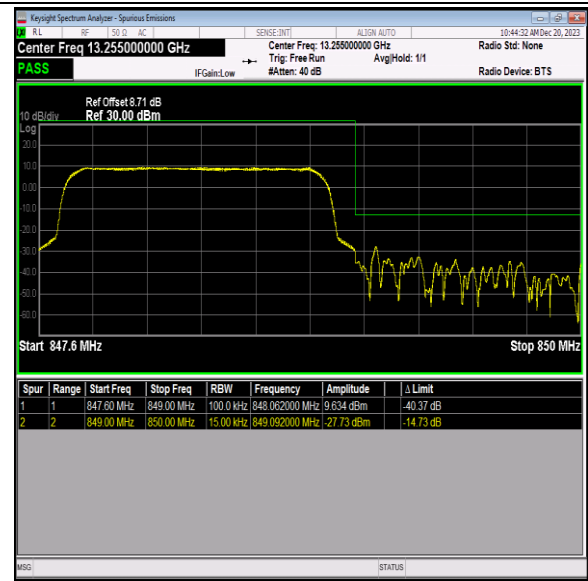
Band5_1.4MHz_QPSK_20643_6RB#0
