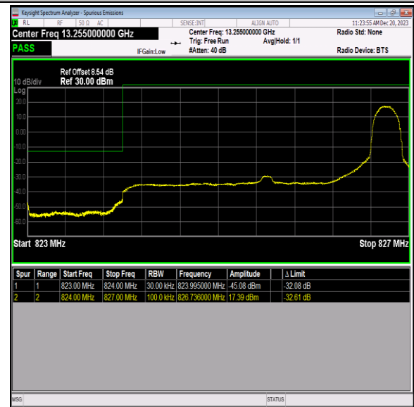
Band5_3MHz_64QAM_20415_1RB#14
