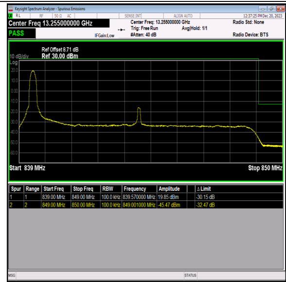
Band5_10MHz_QPSK_20600_1RB#0
