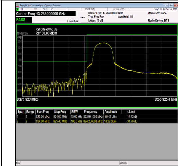
Band5_1.4MHz_16QAM_20407_1RB#0
