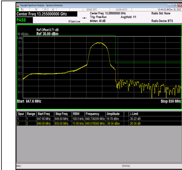
Band5_1.4MHz_QPSK_20643_1RB#5
