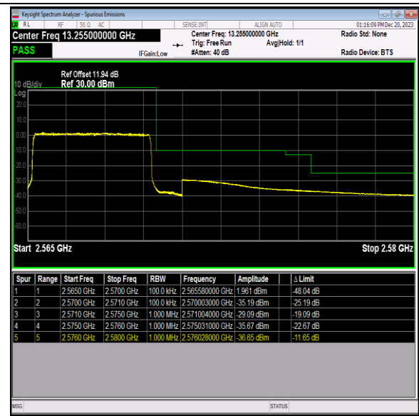
Band7_5MHz_64QAM_21425_25RB#0
