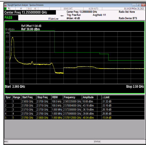
Band7_5MHz_16QAM_21425_1RB#0
