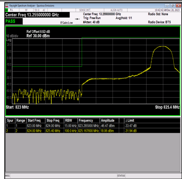
Band5_1.4MHz_16QAM_20407_1RB#5
