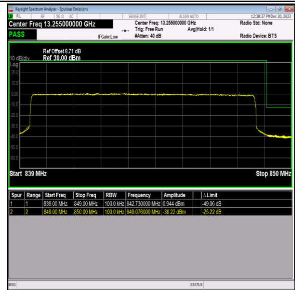
Band5_10MHz_QPSK_20600_50RB#0
