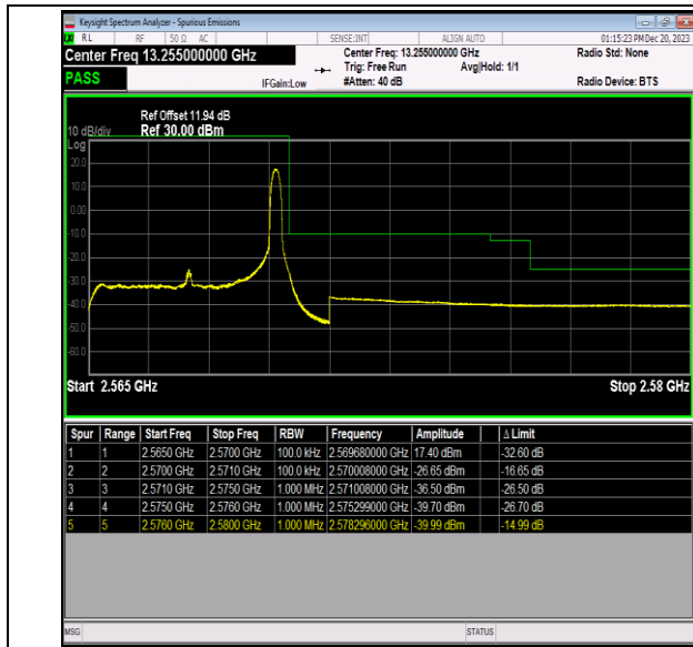
Band7_5MHz_64QAM_21425_1RB#24
