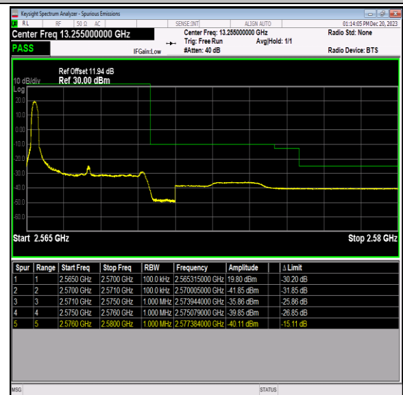
Band7_5MHz_QPSK_21425_1RB#0
