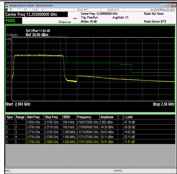
Band7_5MHz_16QAM_21425_25RB#0
