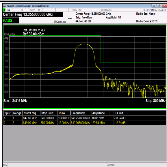
Band5_1.4MHz_16QAM_20643_1RB#5
