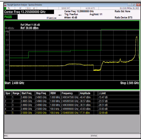
Band7_5MHz_64QAM_20775_1RB#24
