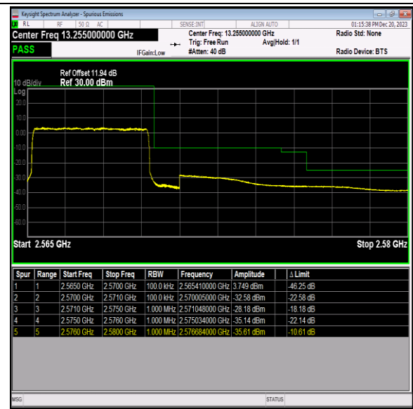
Band7_5MHz_QPSK_21425_25RB#0
