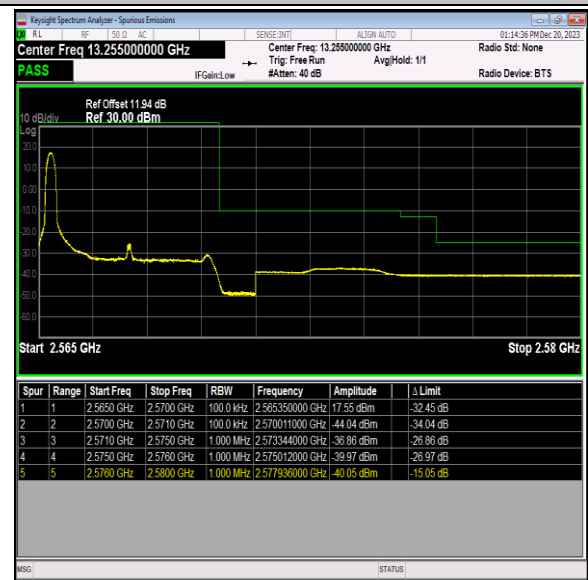
Band7_5MHz_64QAM_21425_1RB#0
