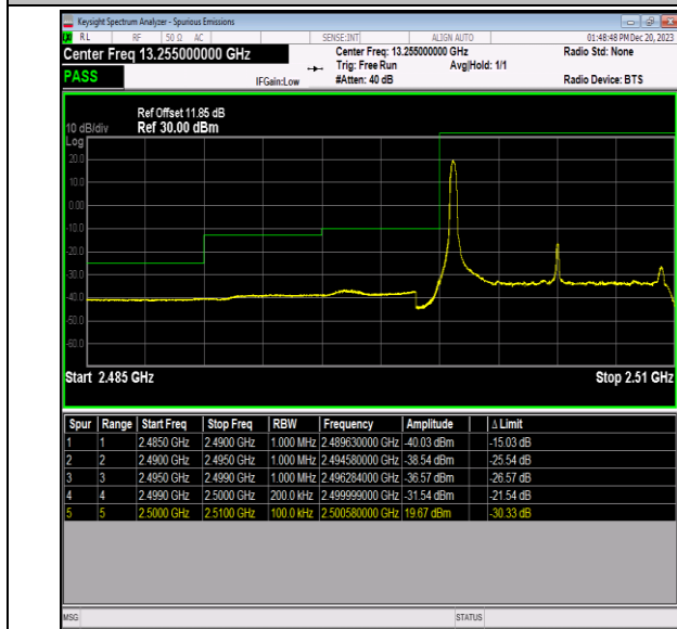
Band7_10MHz_QPSK_20800_1RB#0
