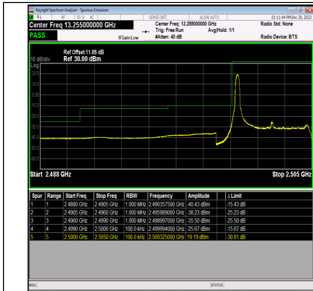
Band7_5MHz_QPSK_20775_1RB#0
