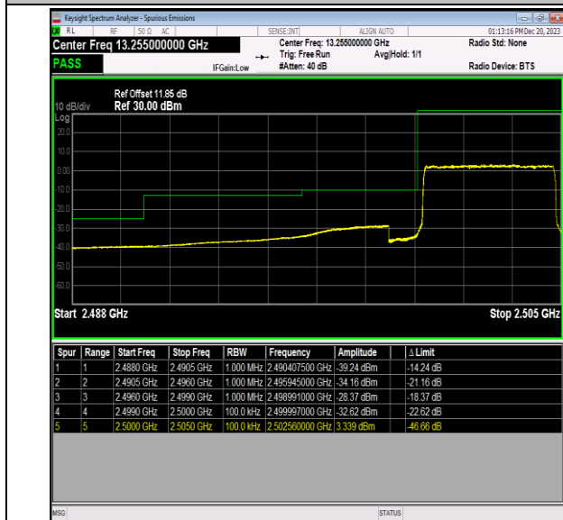
Band7_5MHz_QPSK_20775_25RB#0
