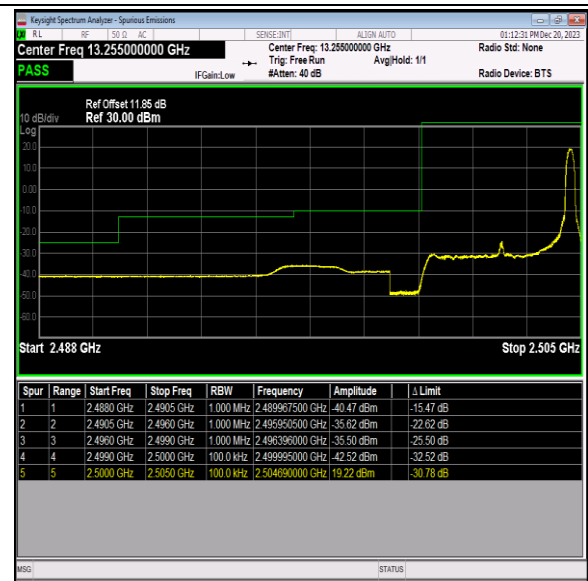
Band7_5MHz_QPSK_20775_1RB#24
