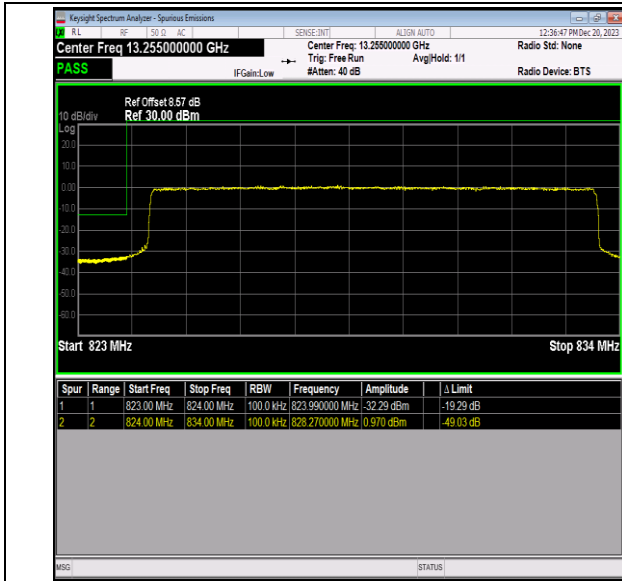
Band5_10MHz_QPSK_20450_50RB#0
