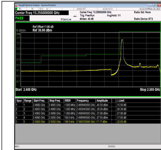
Band7_5MHz_64QAM_20775_1RB#0
