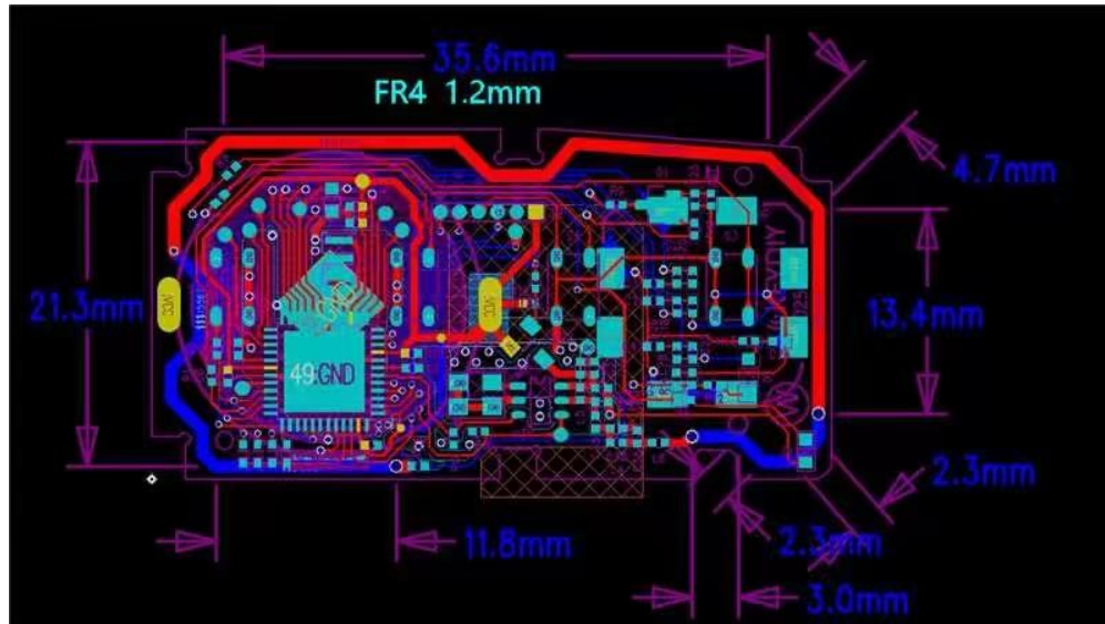
Antenna size diagram
