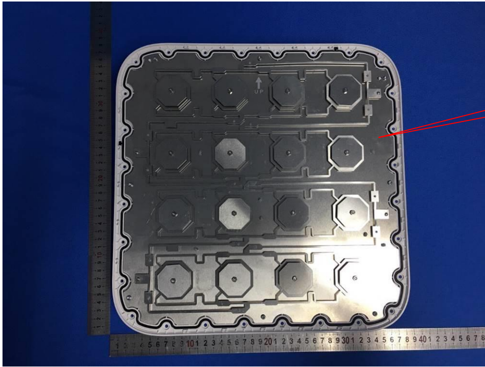
Antenna Panel
