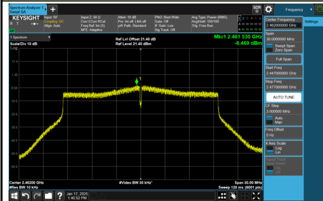
Channel 11 (2462MHz)
