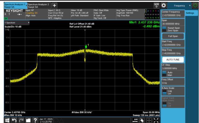
Channel 06 (2437MHz)
