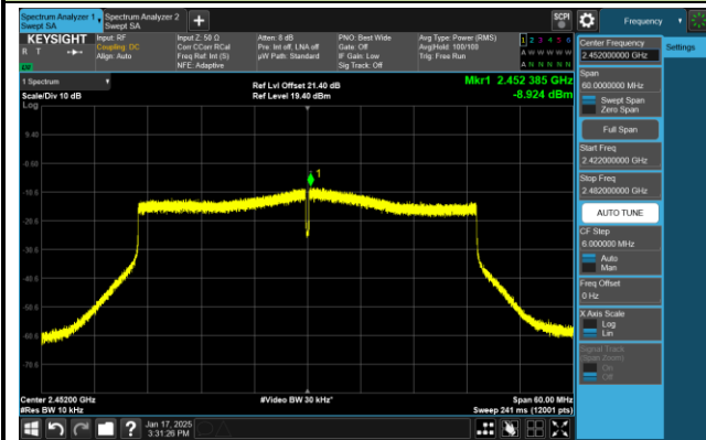
Channel 09 (2452MHz)
