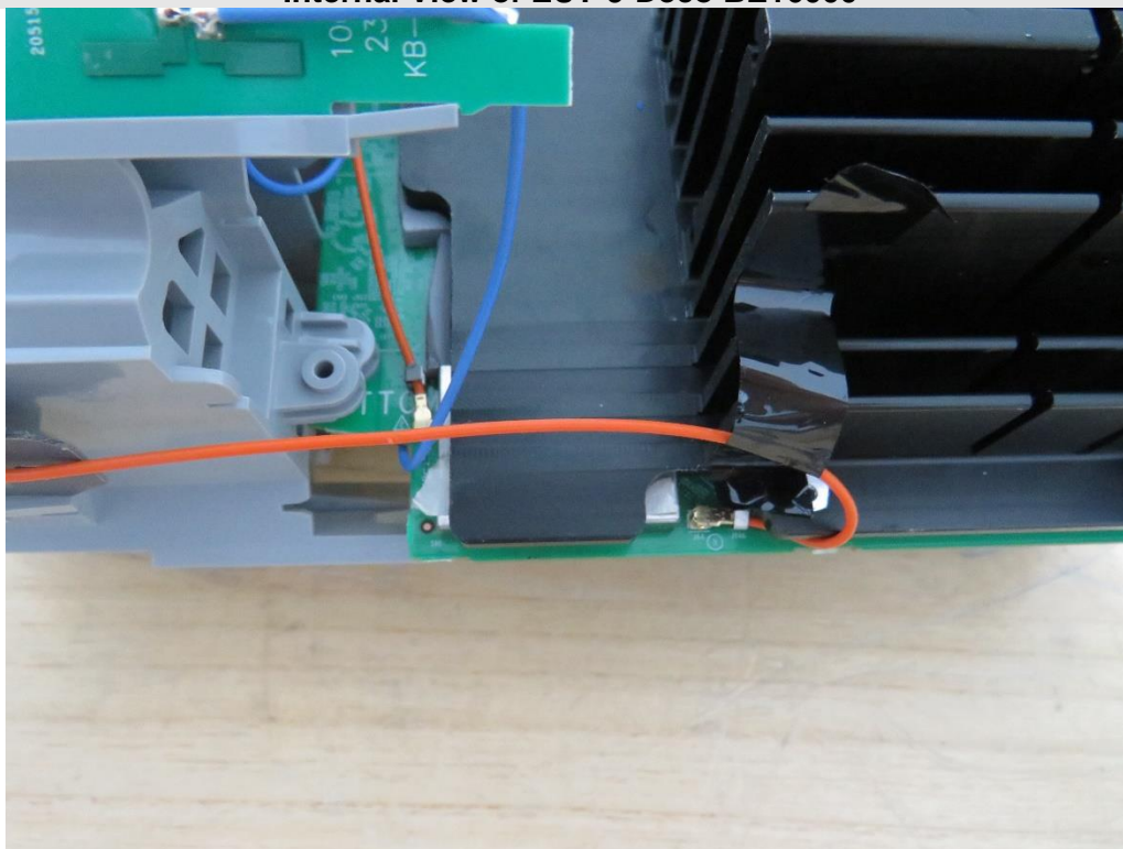
Internal View of EUT-9-Deco BE16000
