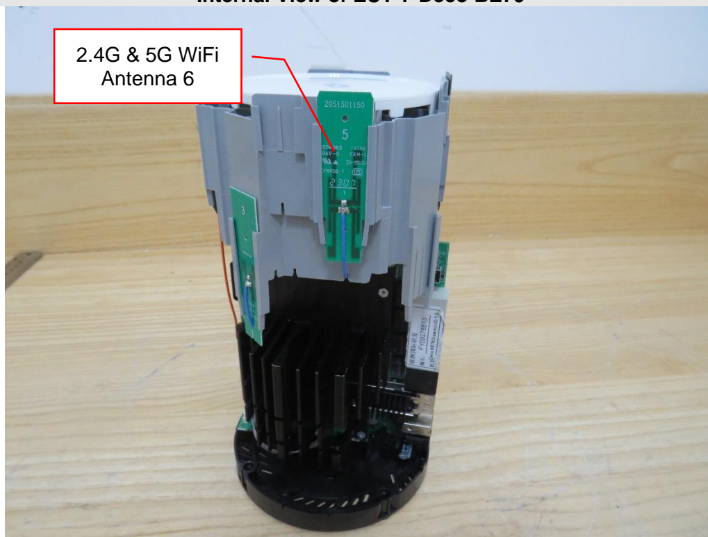
Internal View of EUT-8-Deco BE79
