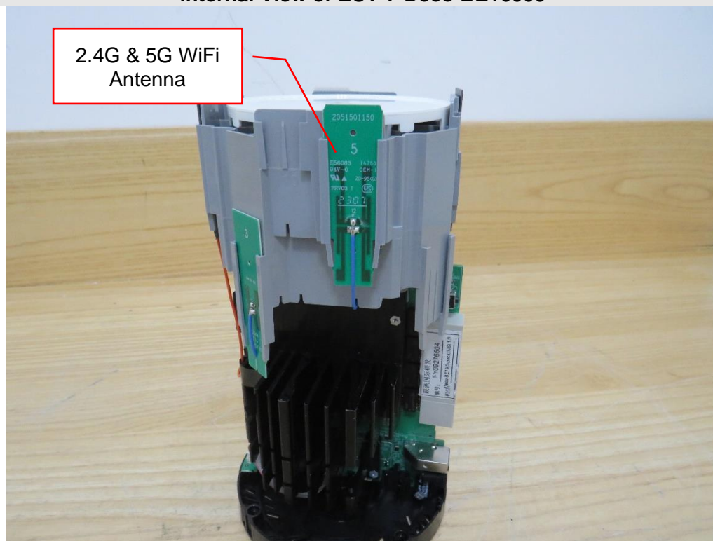
Internal View of EUT-7-Deco BE16000
