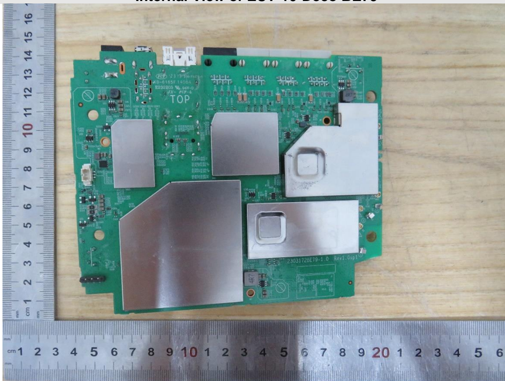
Internal View of EUT-10-Deco BE79
