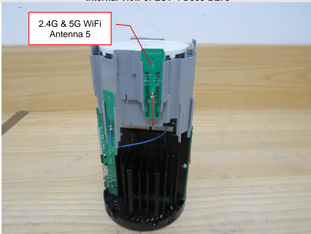
Internal View of EUT-4-Deco BE79
