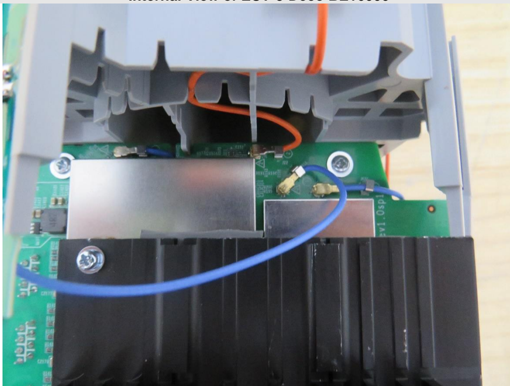
Internal View of EUT-8-Deco BE16000
