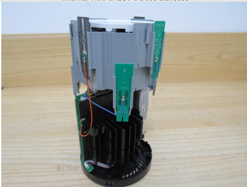
Internal View of EUT-6-Deco BE16000
