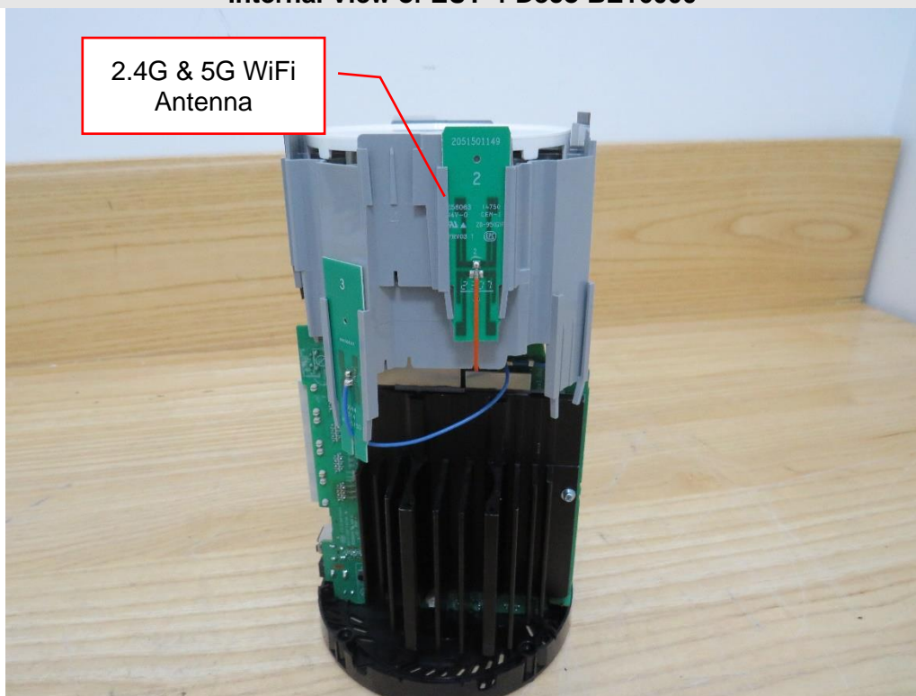
Internal View of EUT-5-Deco BE16000
