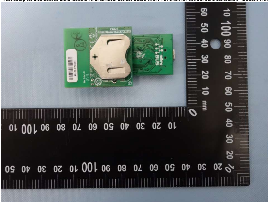
Test setup for 2nd Source BOM Module ATSAMR30M sensor board with FTDI Click for control communication - Bottom View
