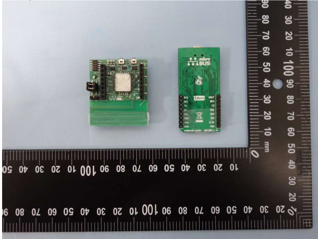
2nd Source BOM Module ATSAMR30M Sensor Board - Top view
