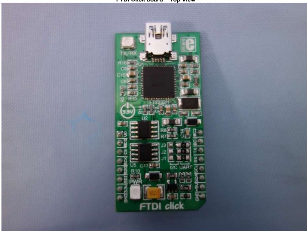
FTDI Click board – Top View
