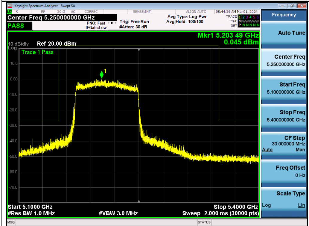
Test_Graph_802.11ax80_ANT1_5210_MCS0_Frequency Band 3
