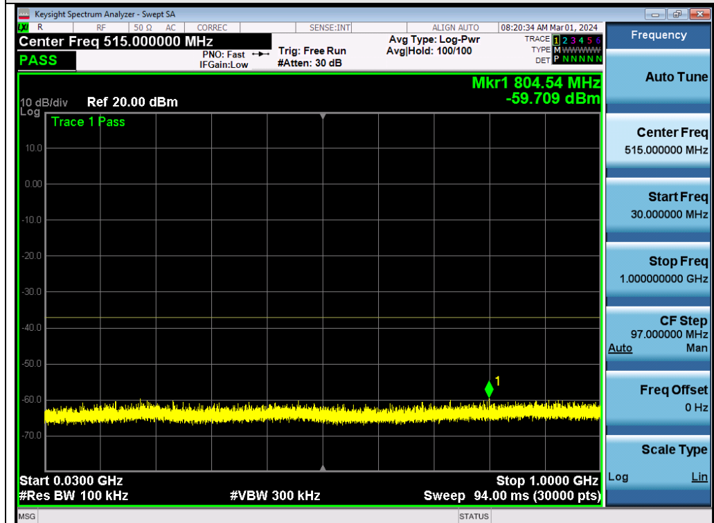
Test_Graph_802.11a_ANT1_5240_6Mbps_Frequency Band 1
