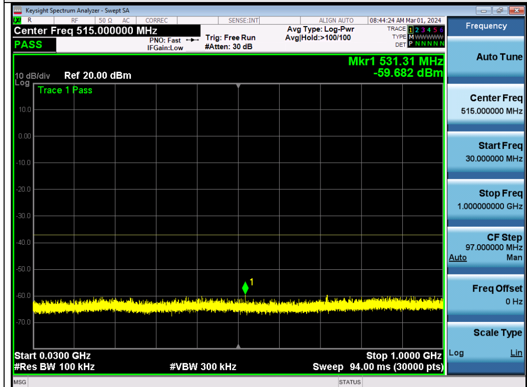
Test_Graph_802.11ax80_ANT1_5210_MCS0_Frequency Band 1
