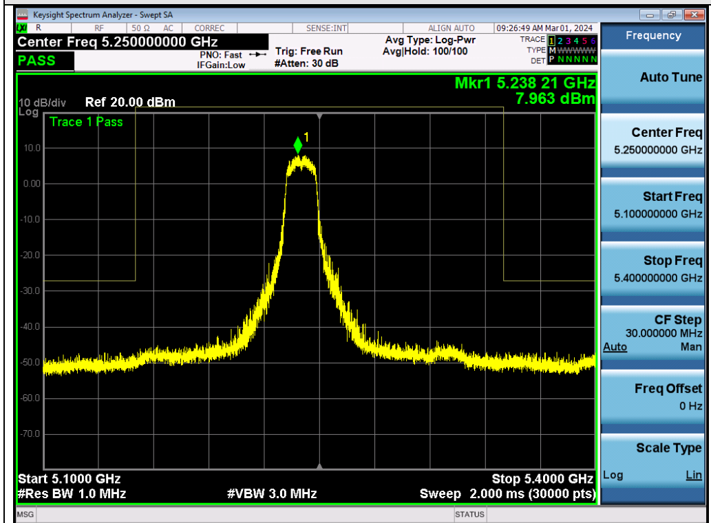
Test_Graph_802.11a_ANT2_5240_6Mbps_Frequency Band 3
