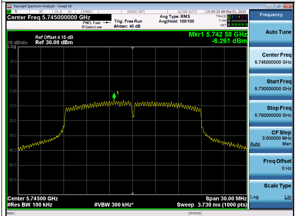
Test_Graph_802.11n20_ANT2_5745_MCS0_PSD
