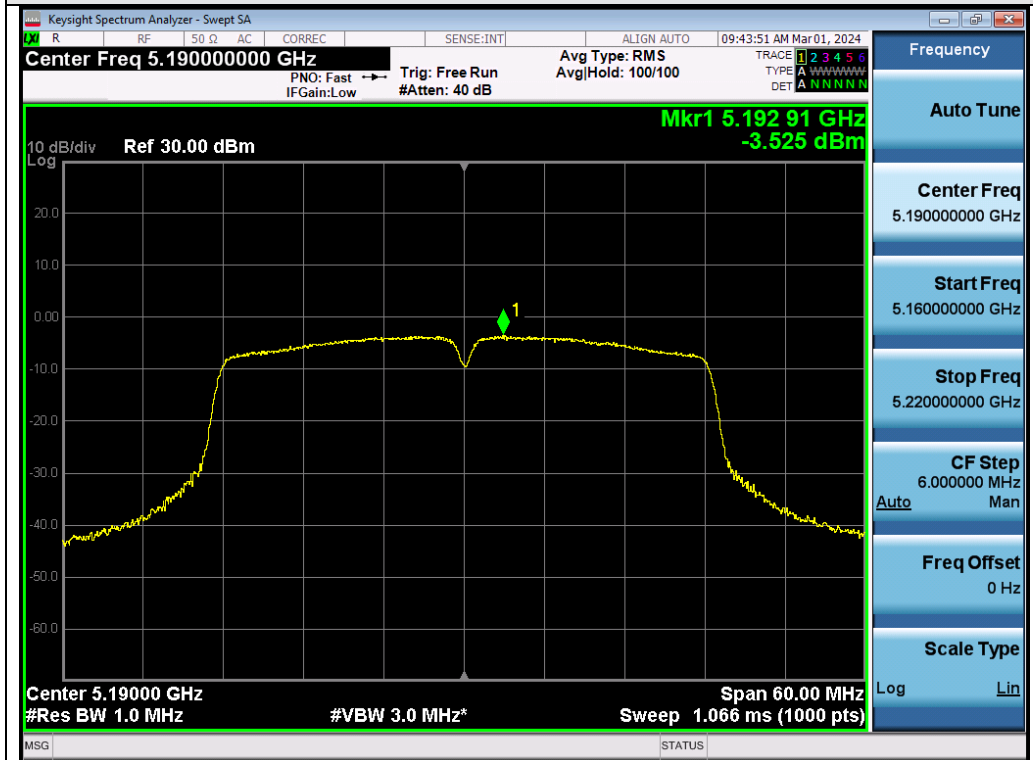
Test_Graph_802.11ac40_ANT2_5190_MCS9_PSD
