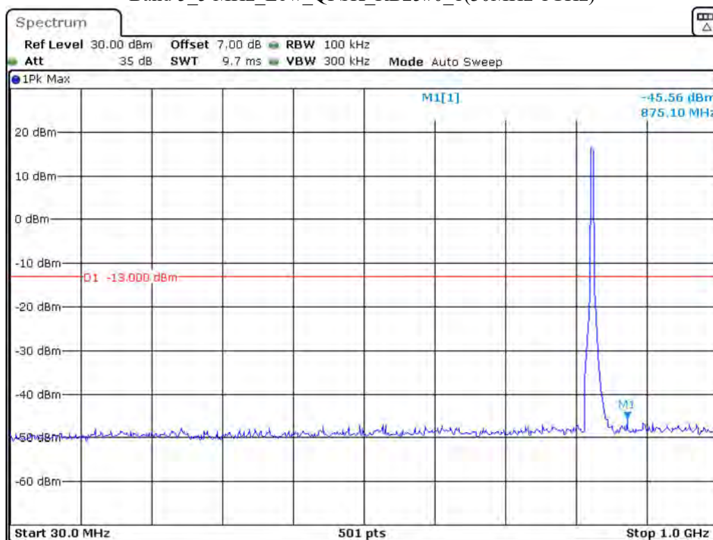
Band 5 5 MHz Low QPSK RB25#0 1(30MHz-1GHz)
