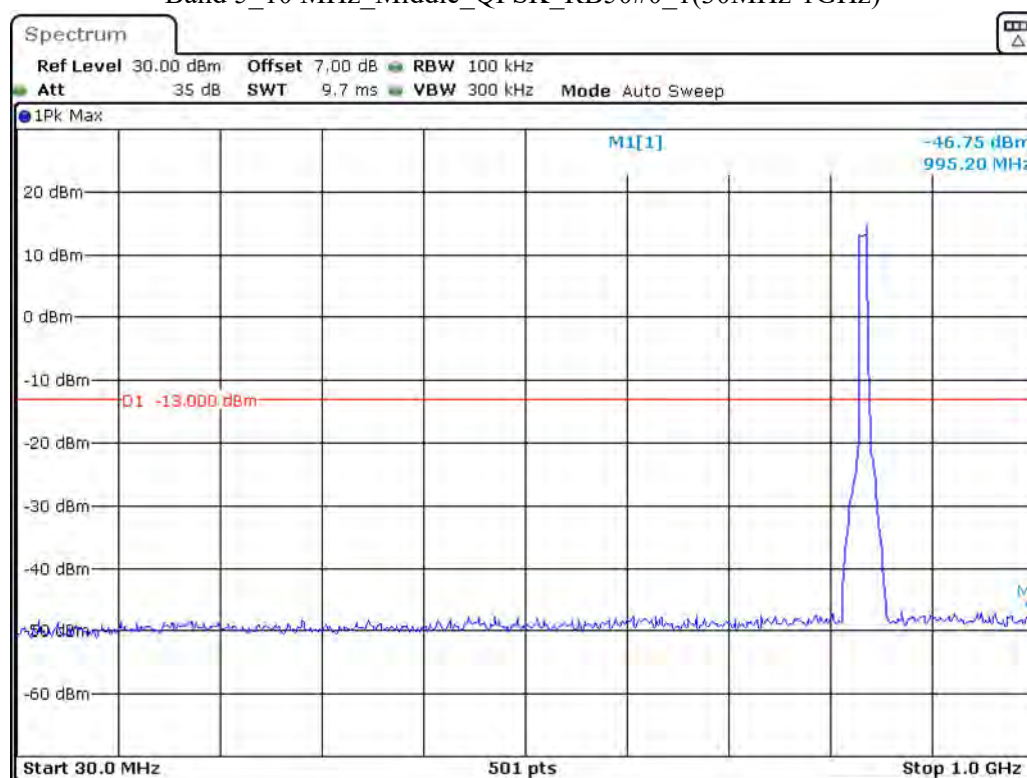
Band 5 10 MHz Middle QPSK RB50#0 1(30MHz-1GHz)
