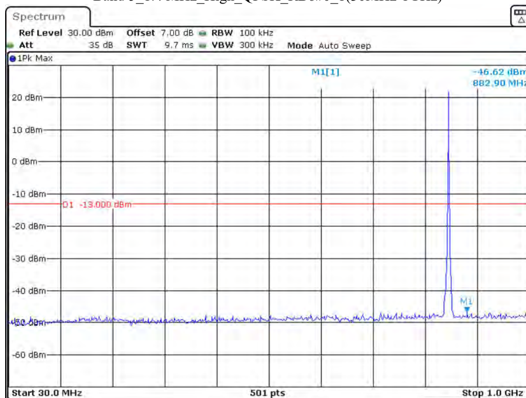
Band 5_1.4 MHz_High_QPSK_RB6#0_1(30MHz-1GHz)
