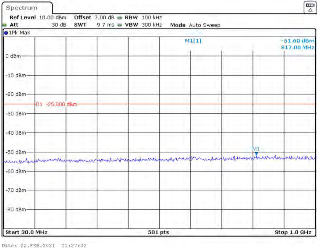
Band 41_15 MHz_Low_QPSK_RB75#0_1(30MHz-1GHz)
