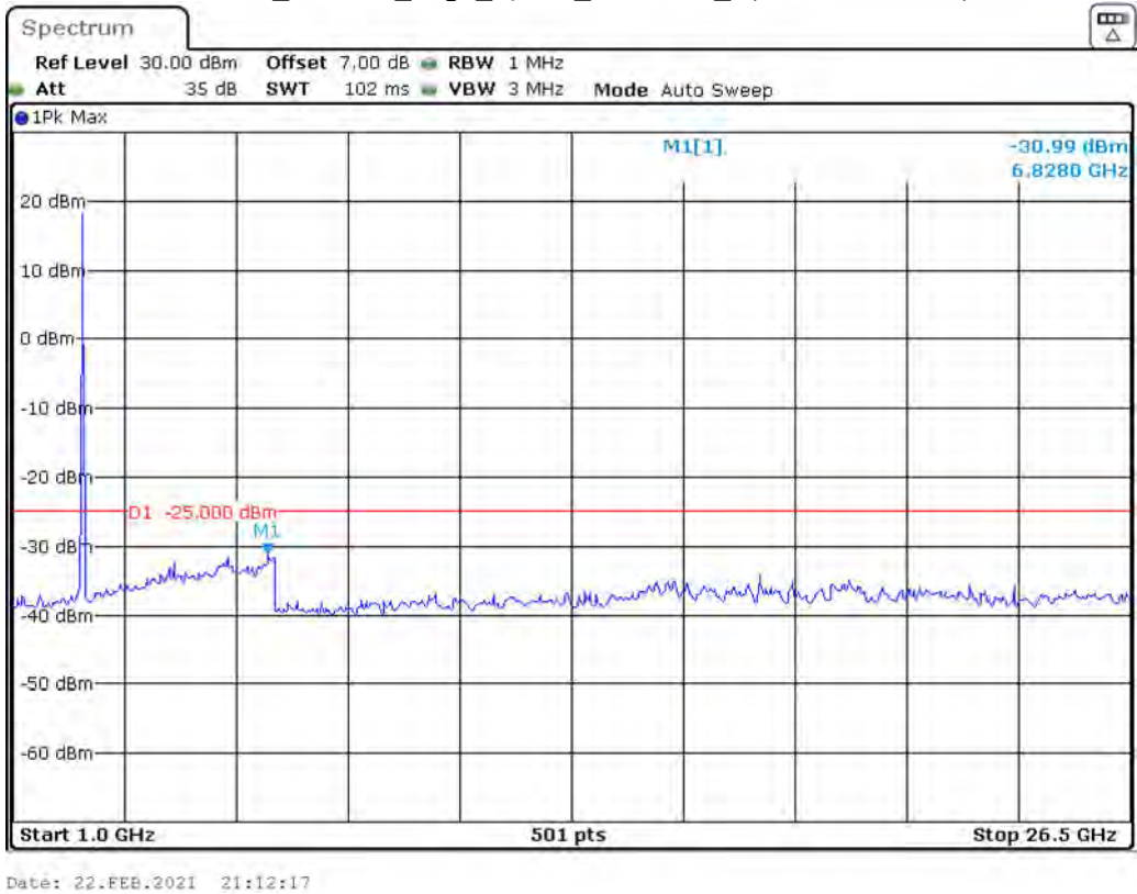
Band 38_20 MHz_High_QPSK_RB100#0_2(1GHz-26.5GHz)
