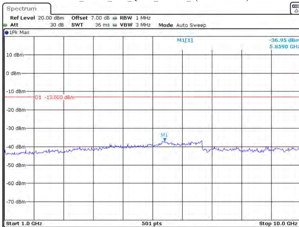
Band 5 5 MHz Low QPSK RB25#0 2(1GHz-10GHz)
