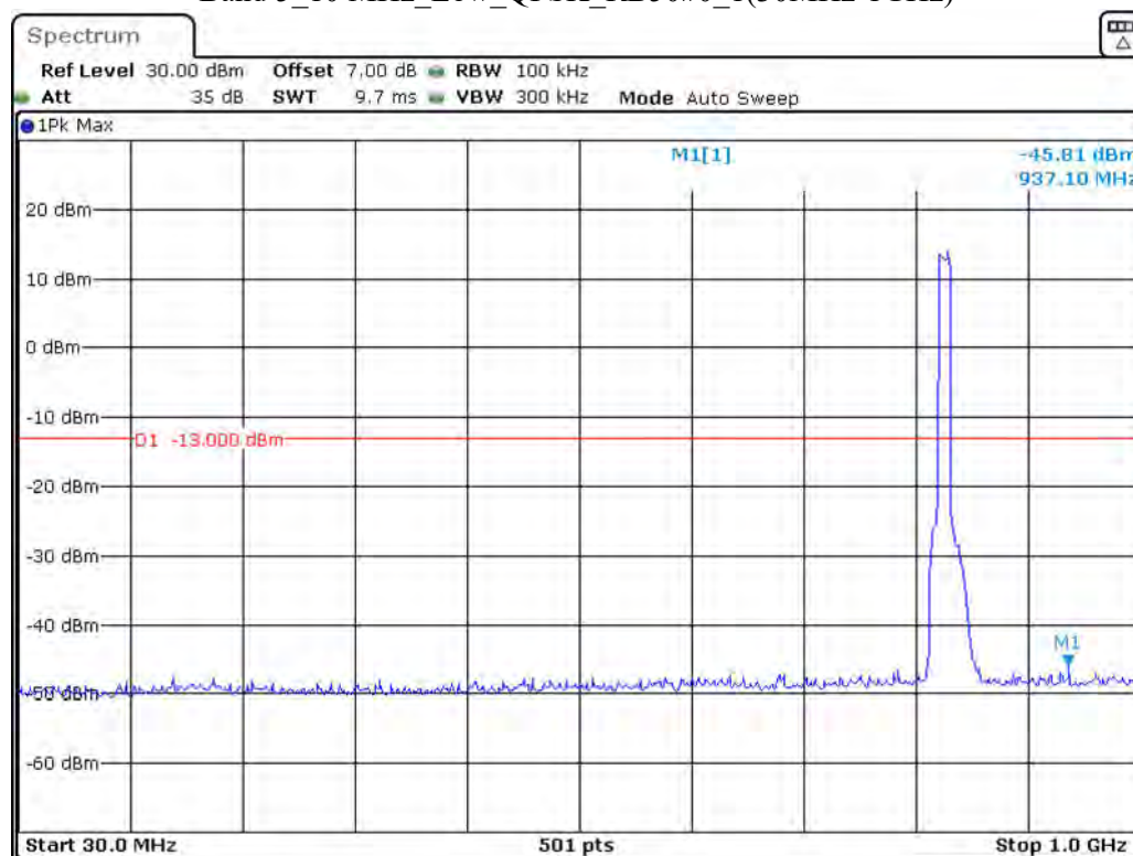
Band 5_10 MHz_Low_QPSK_RB50#0_1(30MHz-1GHz)
