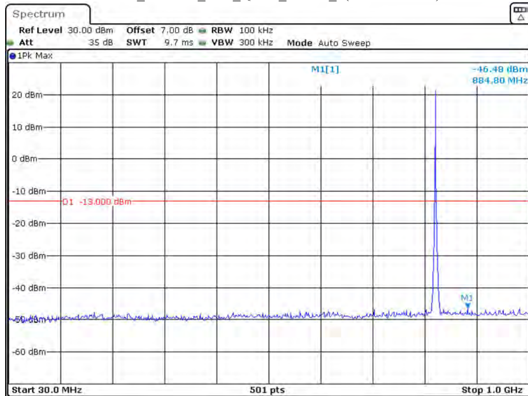
Band 5_1.4 MHz_Low_QPSK_RB6#0_1(30MHz-1GHz)
