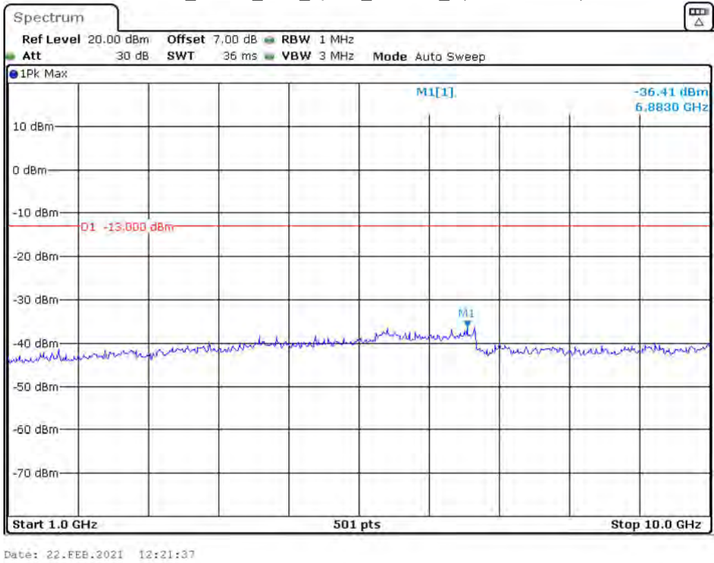
Band 5_3 MHz_Low_QPSK_RB15#0_2(1GHz-10GHz)
