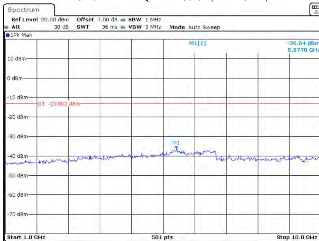
Band 5 10 MHz Low QPSK RB50#0 2(1GHz-10GHz)
