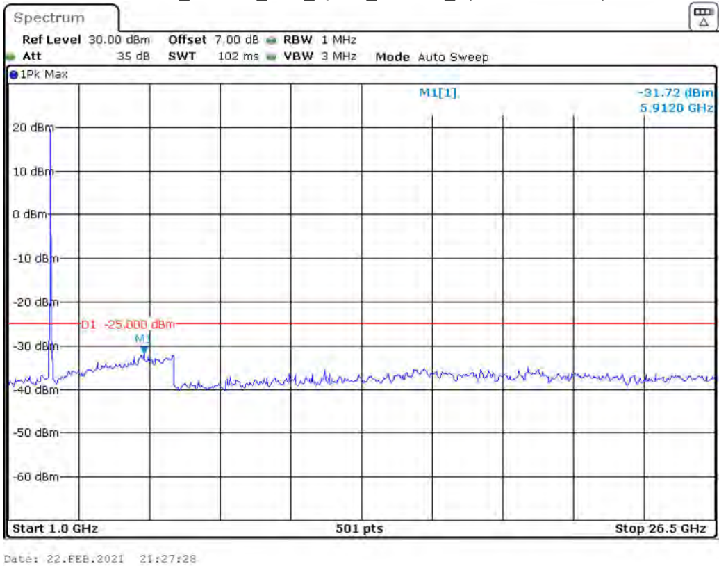
Band 41_15 MHz_Low_QPSK_RB75#0_2(1GHz-26.5GHz)
