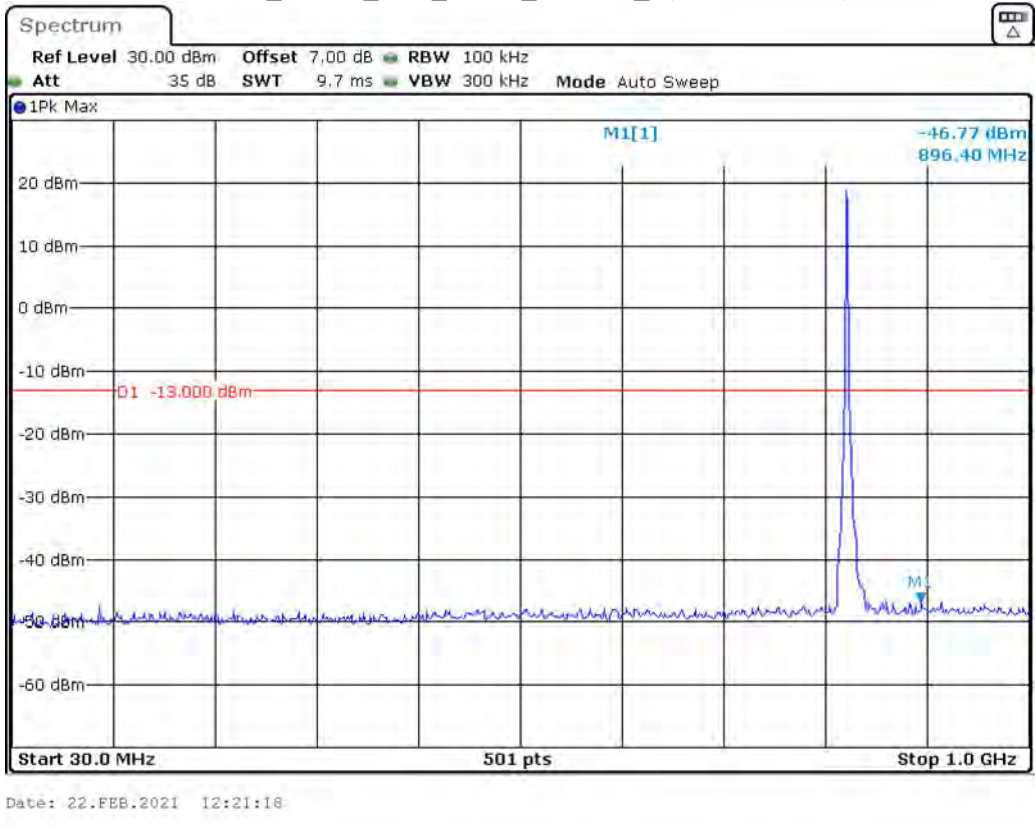
Band 5_3 MHz_Low_QPSK_RB15#0_1(30MHz-1GHz)
