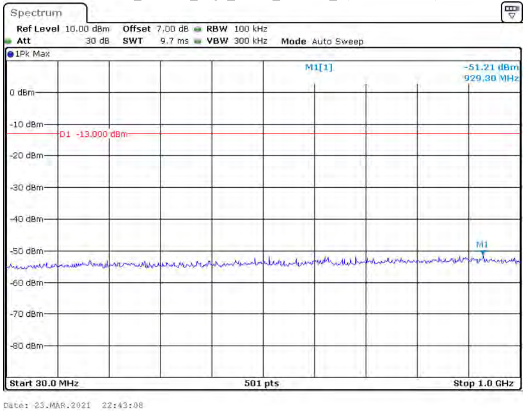
Band 66_15 MHz_High_QPSK_RB75#0_1(30MHz-1GHz)
