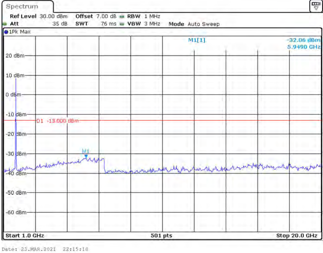
Band 4_20 MHz_Middle_QPSK_RB100#0_2(1GHz-20GHz)
