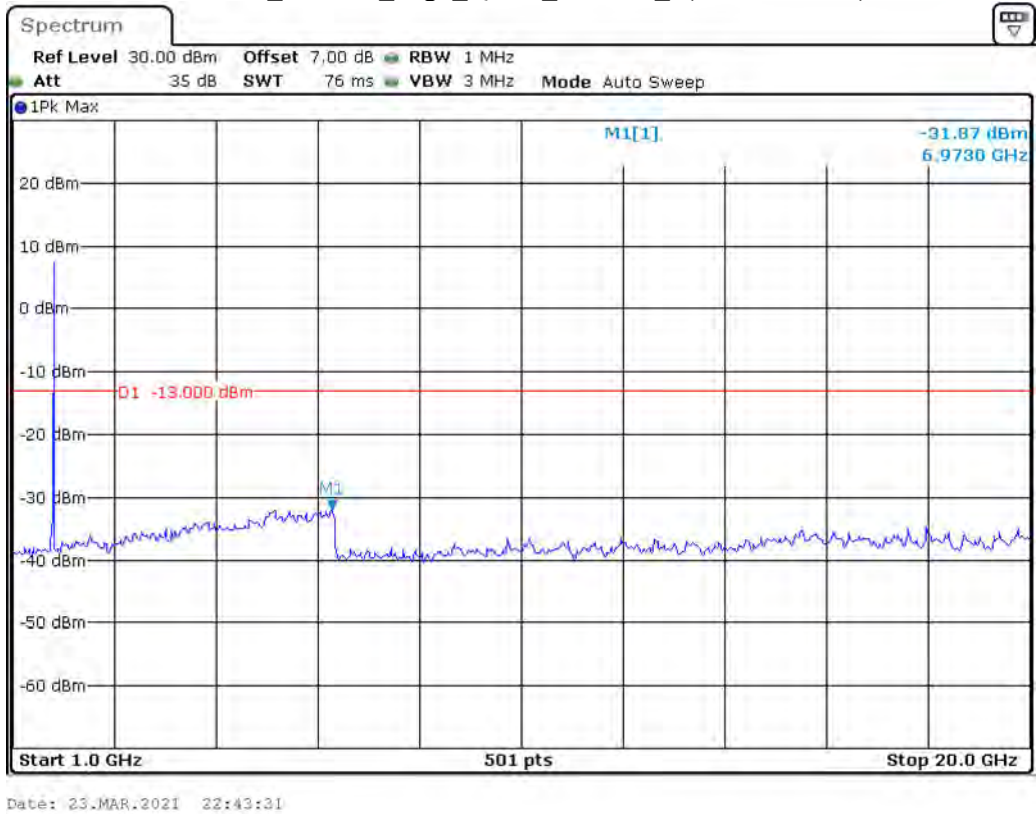
Band 66_15 MHz_High_QPSK_RB75#0_2(1GHz-20GHz)
