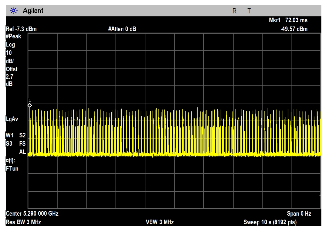
7.7 Channel Loading_801.11VHT80_8192pt_MCS9
