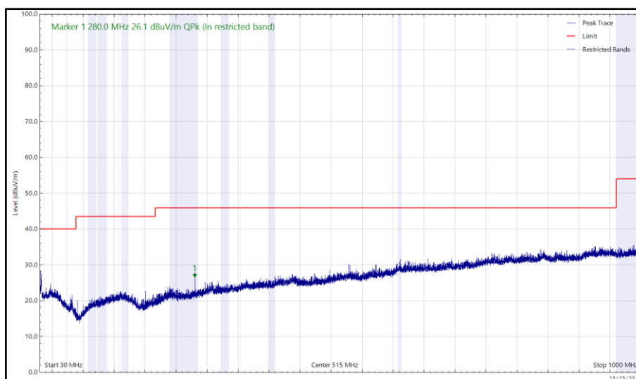
Figure 26 - U-NII-5 - 5955 MHz (CH1), HE20, SU, CDD, Core 0 + Core 1 and 2480 MHz MHz (CH78), 2-DH5, ePA, Core 0 + Core 1, 30 MHz to 1 GHz, Horizontal (Peak)
