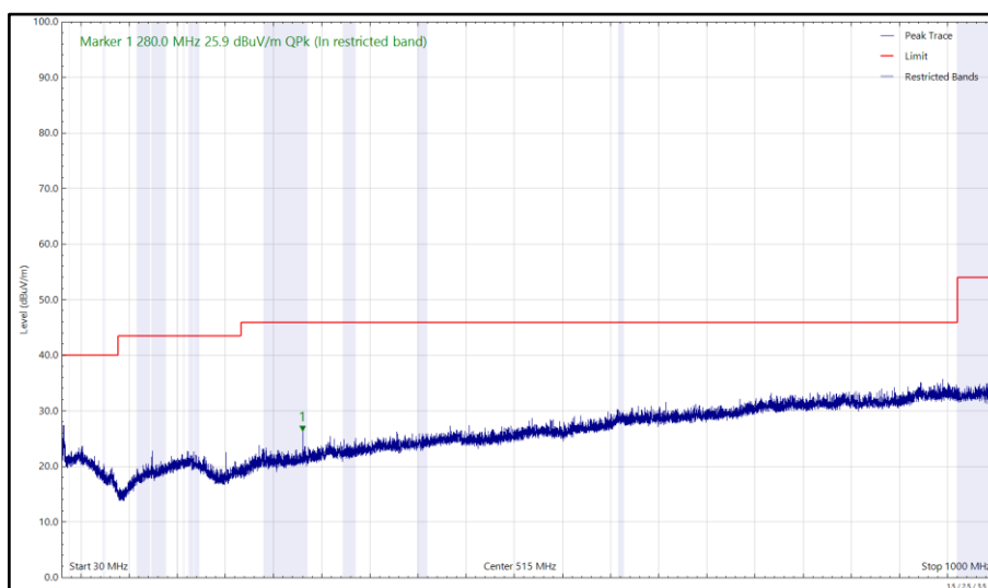
Figure 34 - 2412 MHz z (CH1), HT20, Core 0 and 5162 MHz, HDR4, ePA, Core 1, 30 MHz to 1 GHz, Horizontal (Peak)
