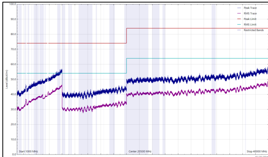
Figure 59 - 2412 MHz (CH1), HT20, Core 1 and 5844 MHz, HDR4, ePA, Core 0, 1 GHz to 40 GHz, Horizontal
