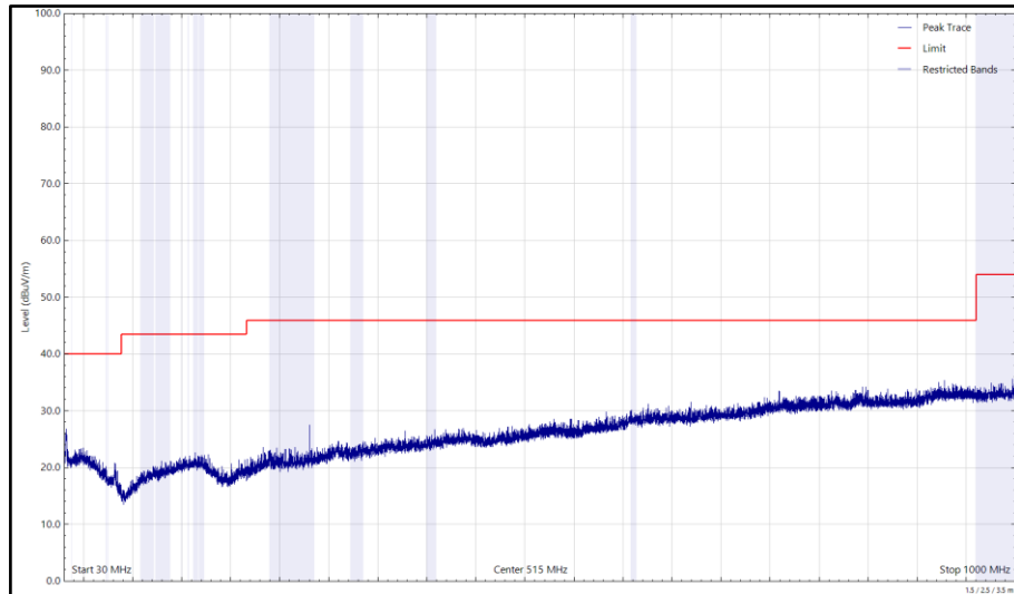
Figure 58 - 2412 MHz (CH1), HT20, Core 1 and 5844 MHz, HDR4, ePA, Core 0, 30 MHz to 1 GHz, Horizontal (Peak)
