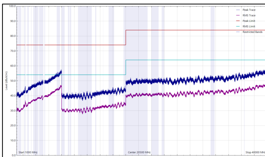
Figure 35 - 2412 MHz (CH1), HT20, Core 0 and 5162 MHz, HDR4, ePA, Core 1, 1 GHz to 40 GHz, Horizontal
