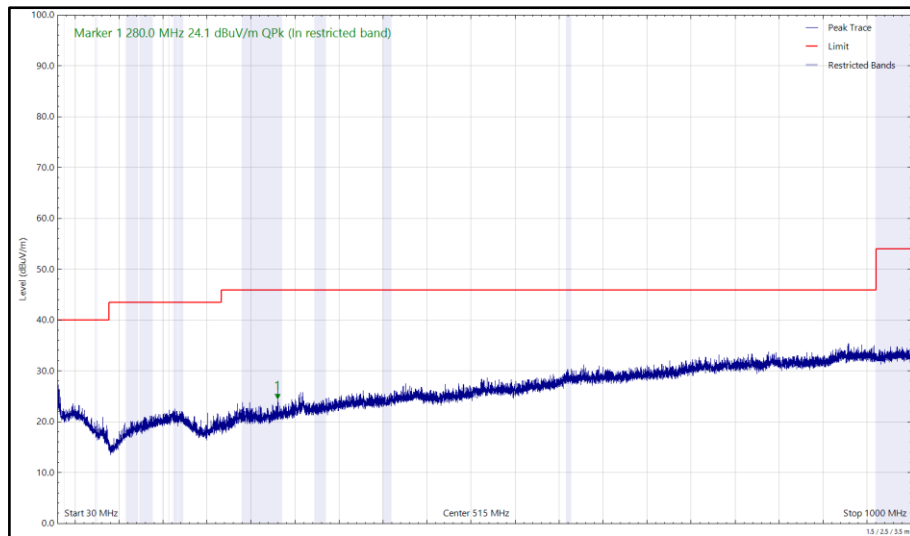
Figure 38 - 2472 MHz (CH13), HT20, Core 0 and 5162 MHz, HDR4, ePA, Core 1, 30 MHz to 1 GHz, Horizontal (Peak)
