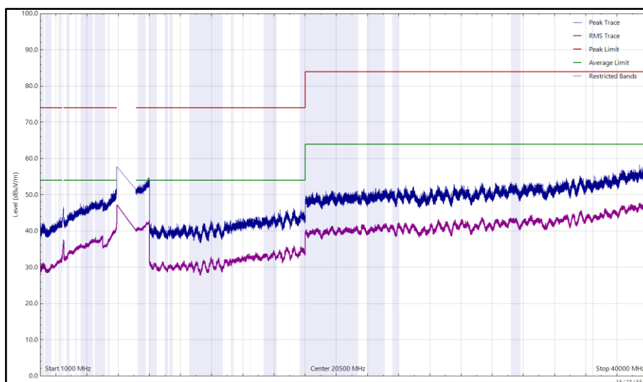
Figure 27 - U-NII-5 - 5955 MHz (CH1), HE20, SU, CDD, Core 0 + Core 1 and 2480 MHz MHz (CH78), 2-DH5, ePA, Core 0 + Core 1, 1 GHz to 40 GHz, Horizontal
