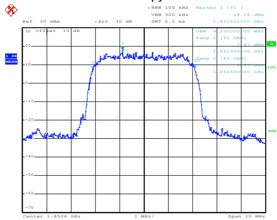
99% Occupy bandwidth
