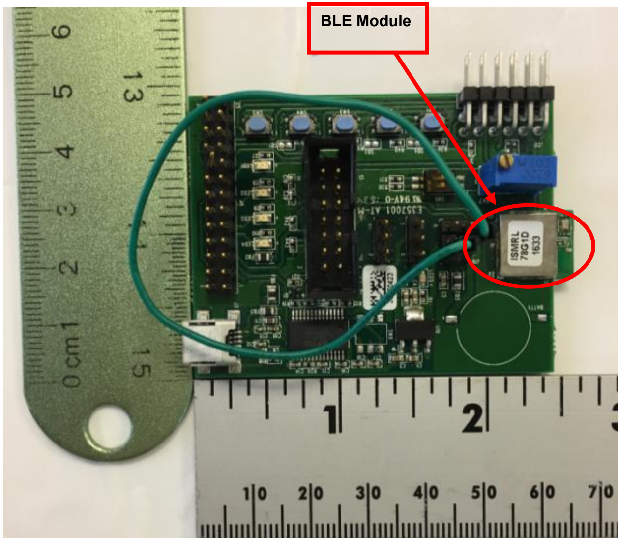
Figure 1. Placement of Module on Evaluation Board
