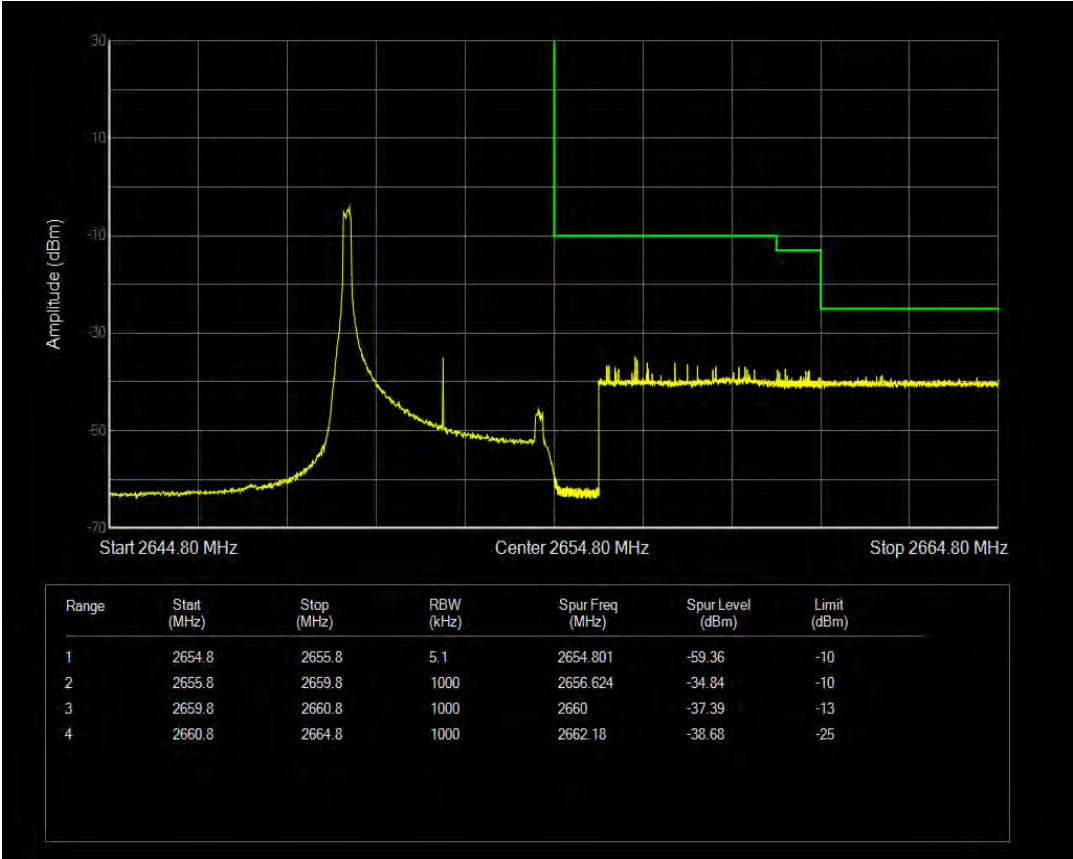
Band41 QAM16 BW=5MHz Channel=41213 RB Size=1 Position=#0
