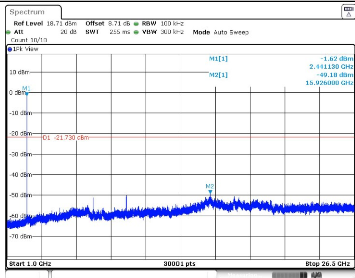
2DH5_Ant1_2441_1000~26500
