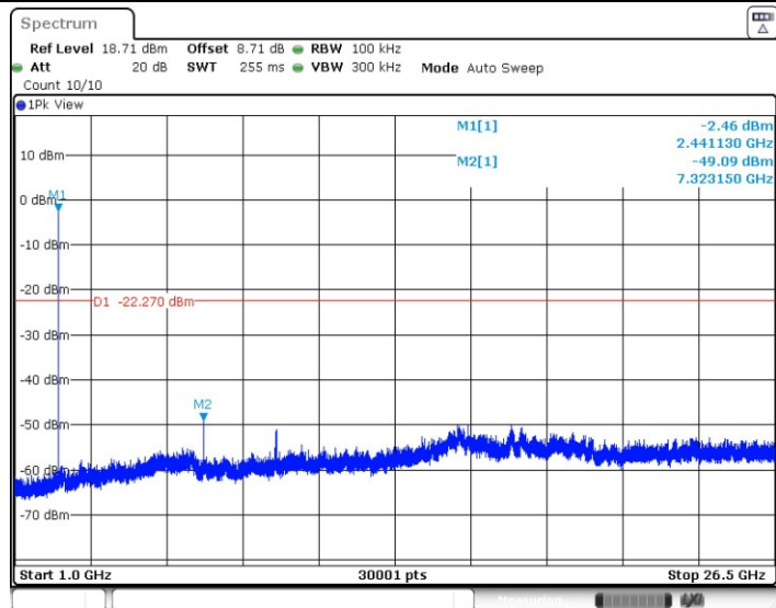
3DH5_Ant1_2441_1000~26500
