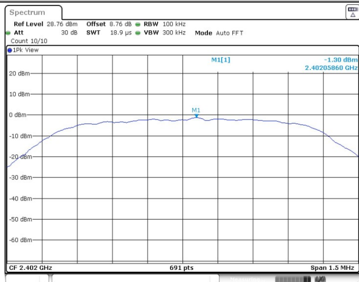
2DH5_Ant1_2402_0~Reference
