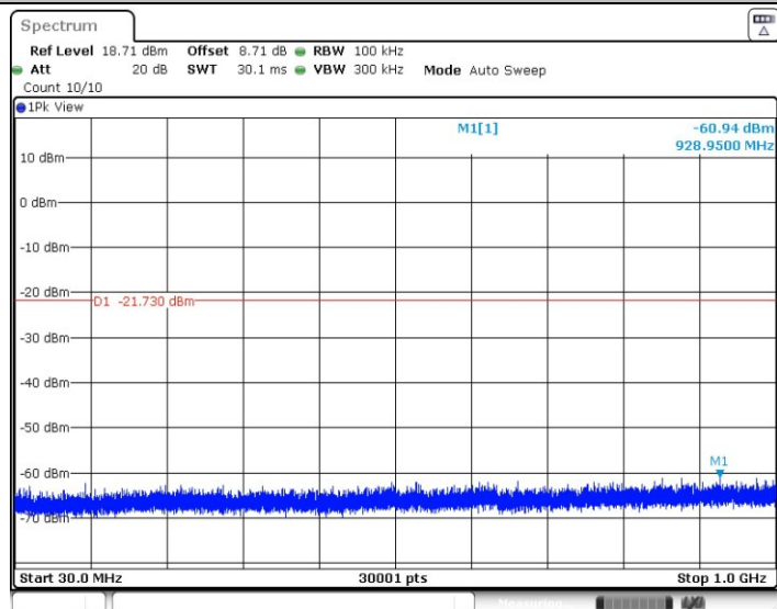
2DH5_Ant1_2441_30~1000
