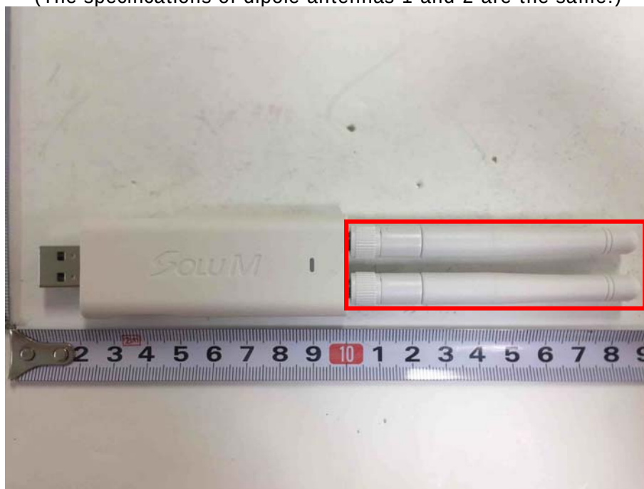
Dipole Antenna 3 & 4 (The specifications of dipole antennas 3 and 4 are the same.)
