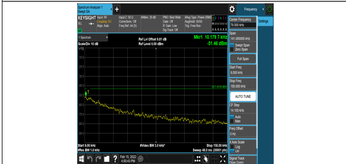
Band25-20MHz-QPSK-26140-1-0-Low-0.009-0.15--51.46-PASS
