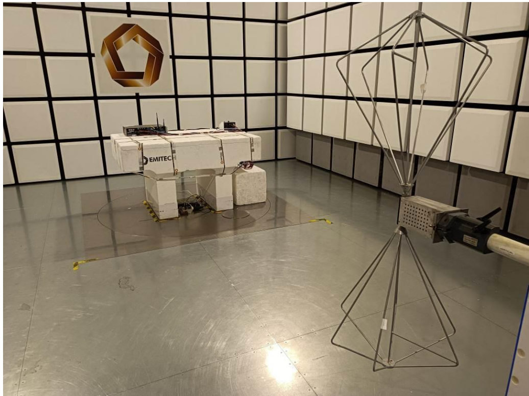
TEST SETUP PHOTO(S) – SETUP FOR FREQ < 200MHZ
