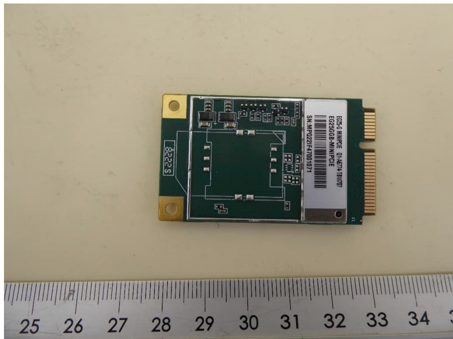
Cellular module bottom view
