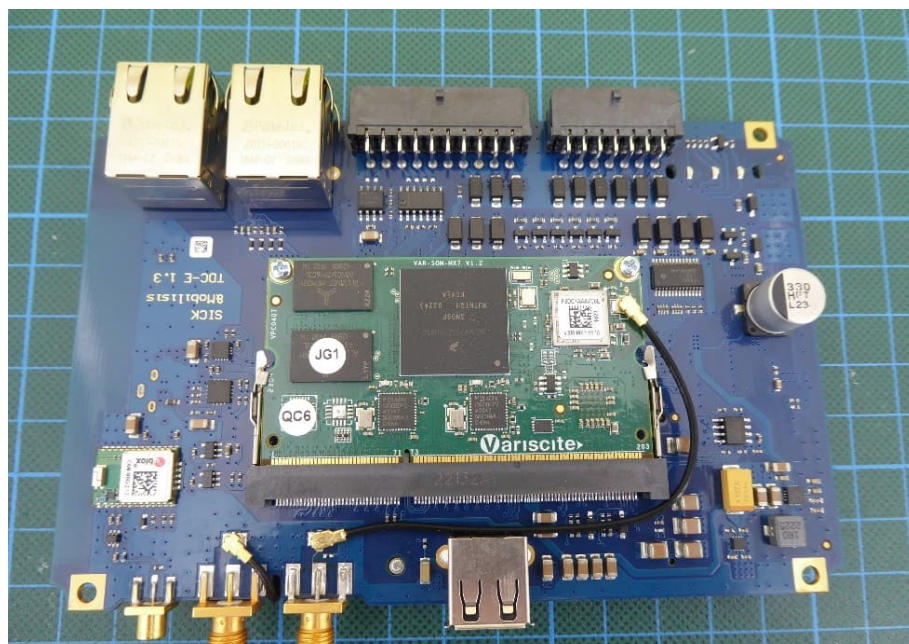
EUT internal view 3
