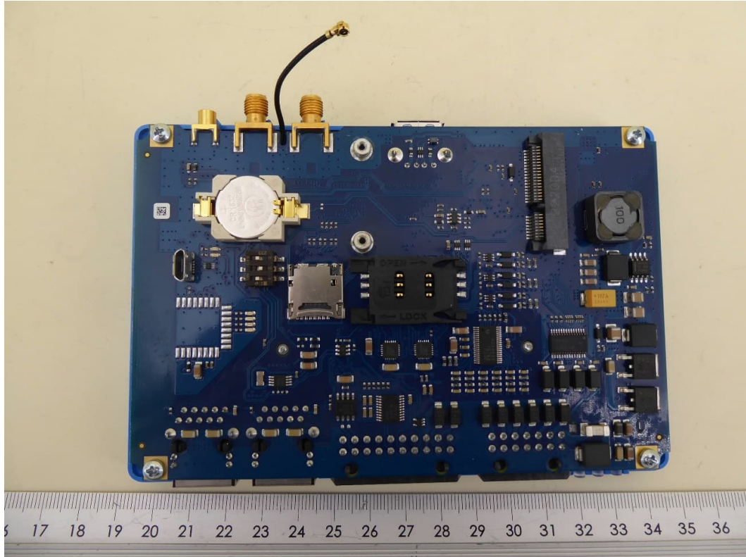
EUT Internal view 4 with depopulated module
