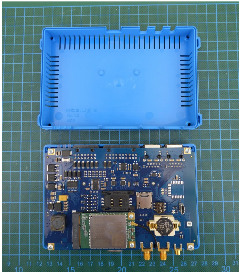
EUT internal view 1
