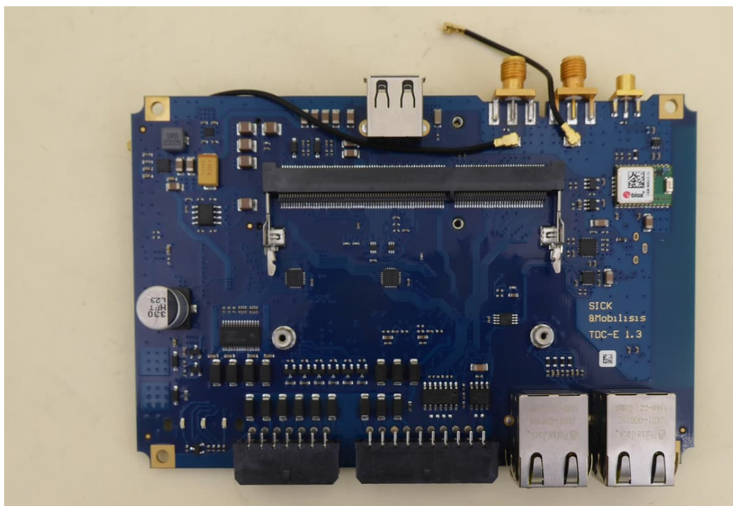
EUT Internal view 5 with depopulated module
