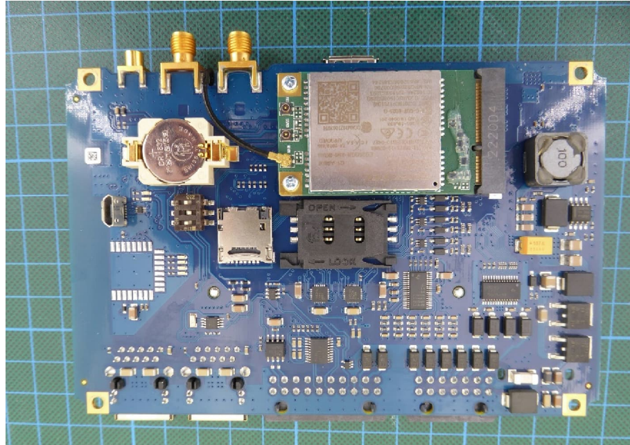
EUT internal view 2
