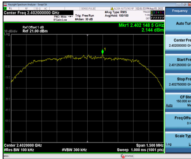
2DH5_Ant2_2402_0~Reference
