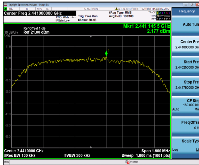
3DH5_Ant2_2441_0~Reference
