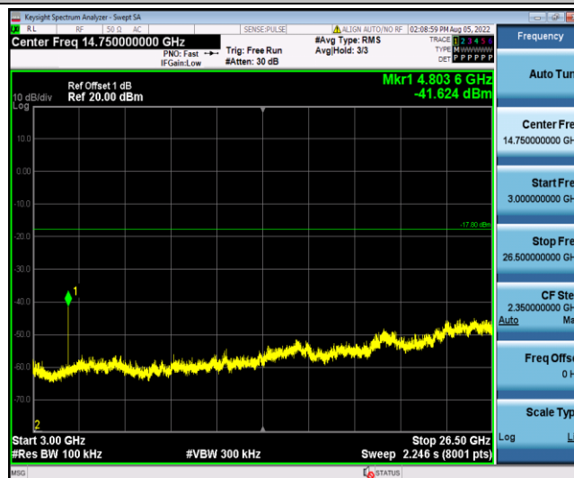
3DH5_Ant2_2402_3000~26500
