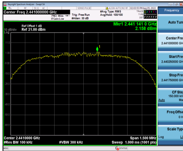
2DH5_Ant2_2441_0~Reference
