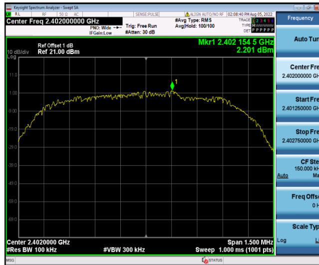
3DH5_Ant2_2402_0~Reference
