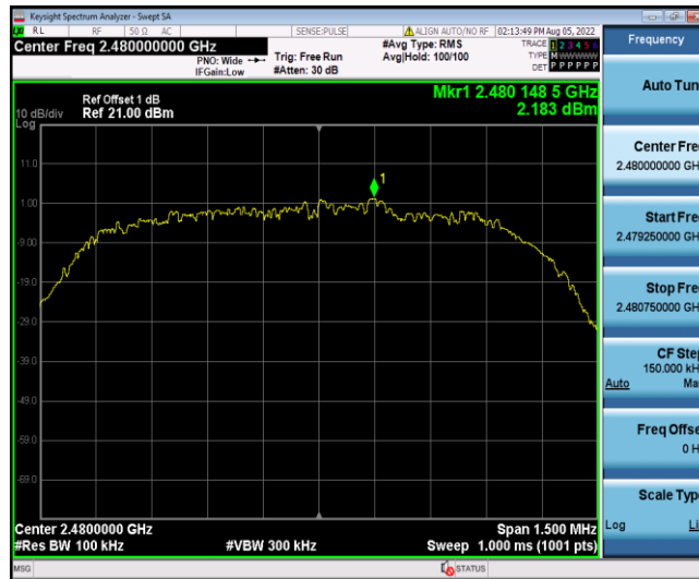
3DH5_Ant2_2480_0~Reference
