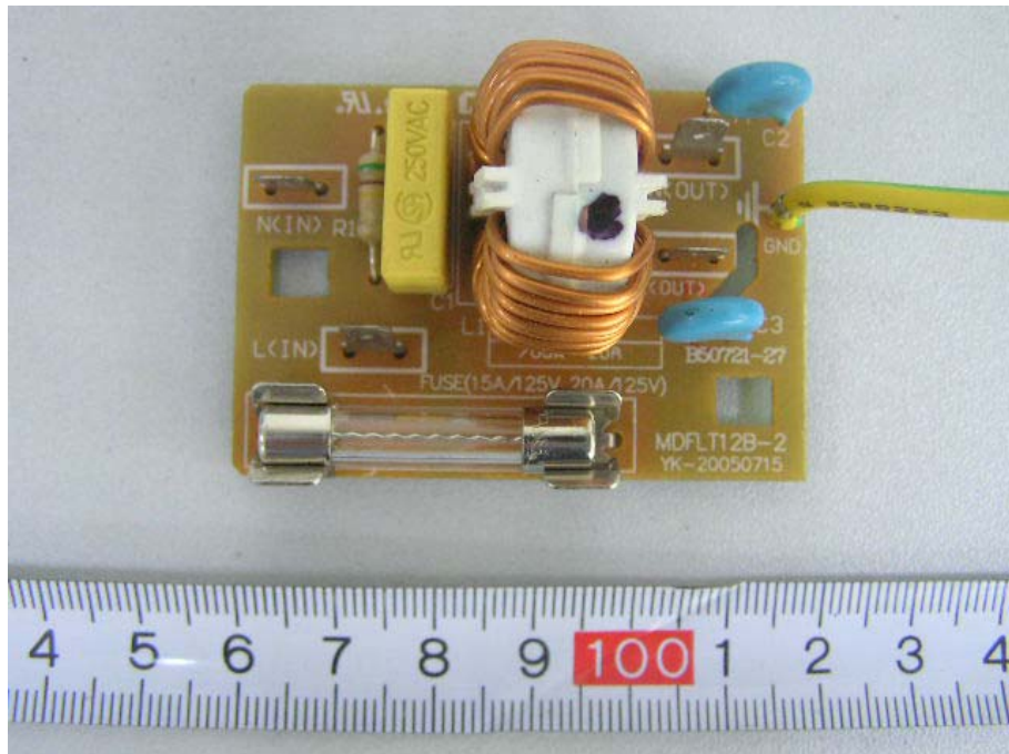
EUT – Power PCB Front View
