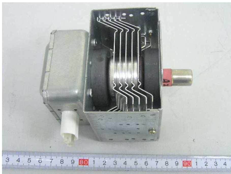
EUT- Magnetron View (2)
