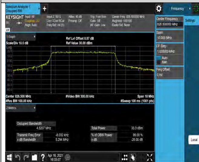
Band5-5MHz-QPSK-20625-25RB#0
