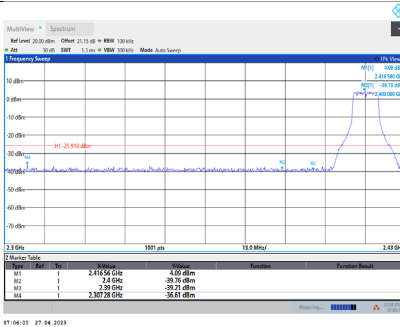
11G_Ant2_Low_2417
