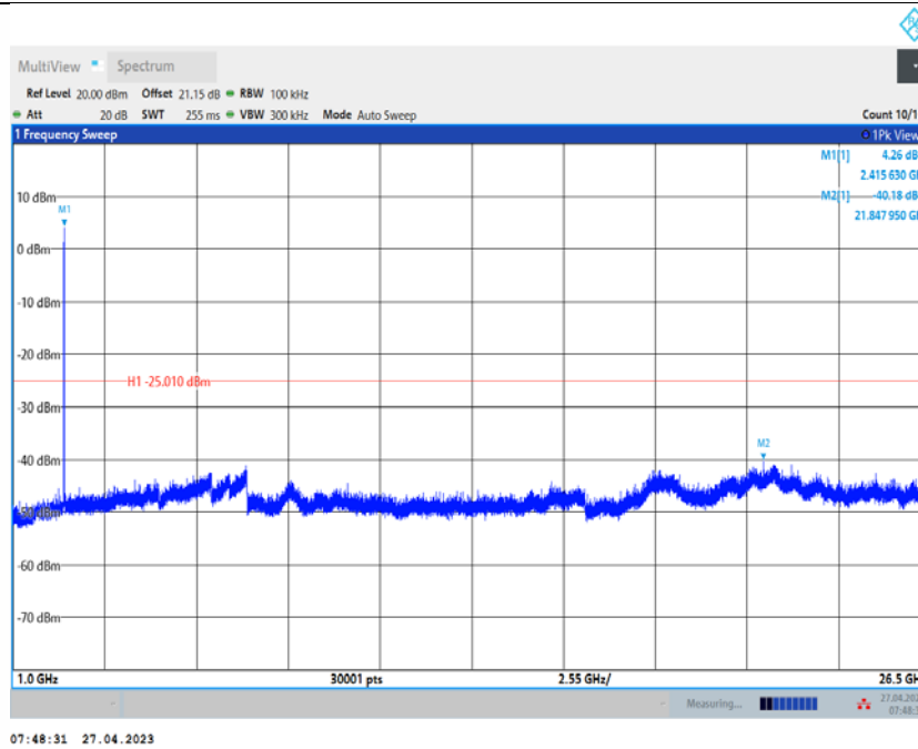
11N20SISO_Ant2_2417_0-Reference
