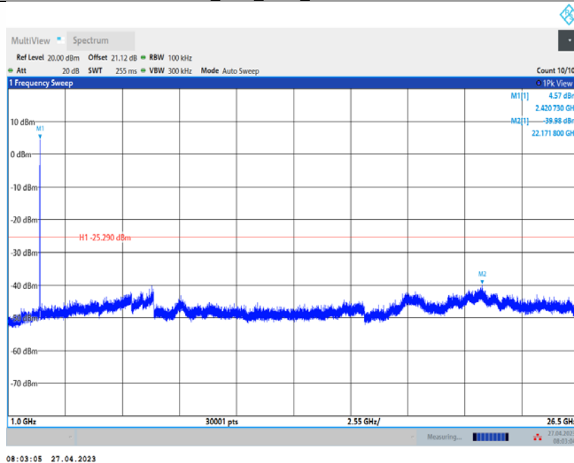
11N20SISO_Ant1_2417_0-Reference
