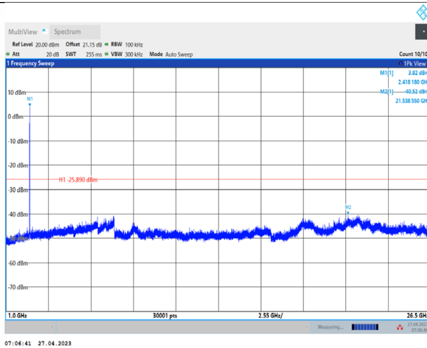
11G_Ant2_2417_0~Reference
