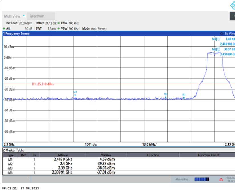
11N20SISO_Ant1_Low_2417
