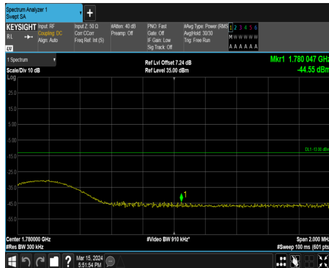
Band66-15MHz-16QAM-132597-1RB#74
