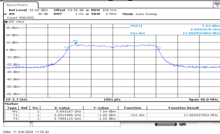
11A-CDD_Ant4_5700
