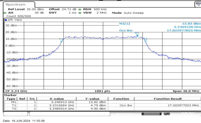
11A-CDD_Ant3_5240
