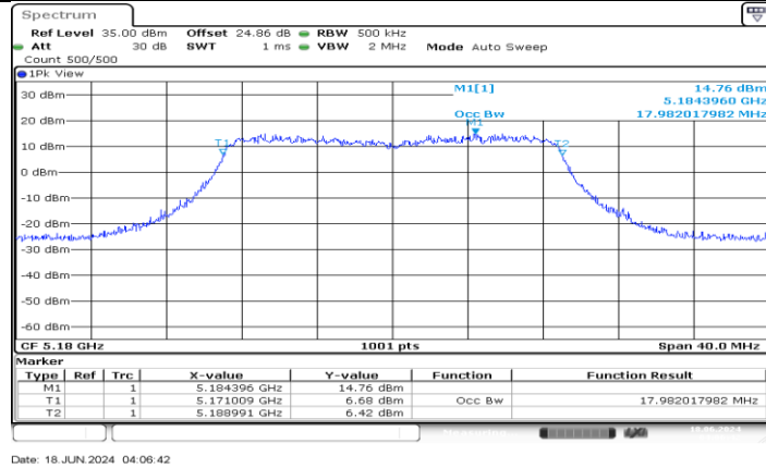
11AC20MIMO_Ant4_5180
