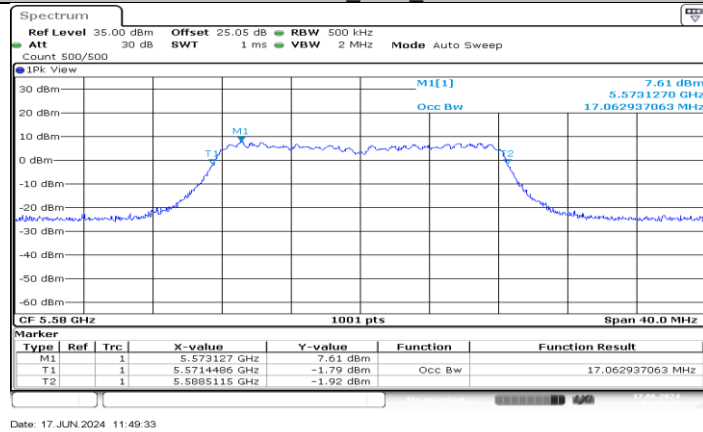
11A-CDD_Ant4_5580
