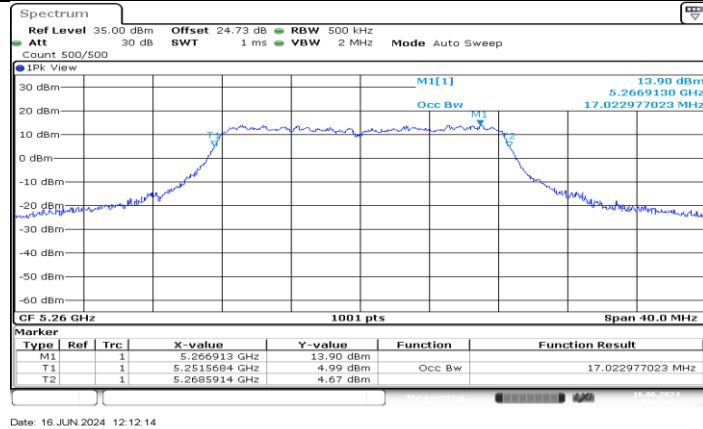
11A-CDD_Ant3_5260
