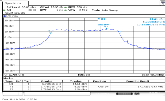
11A-CDD_Ant2_5785
