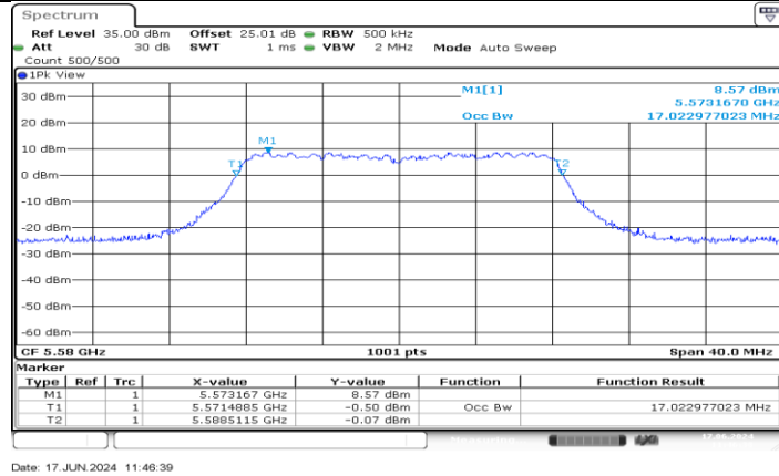
11A-CDD_Ant3_5580
