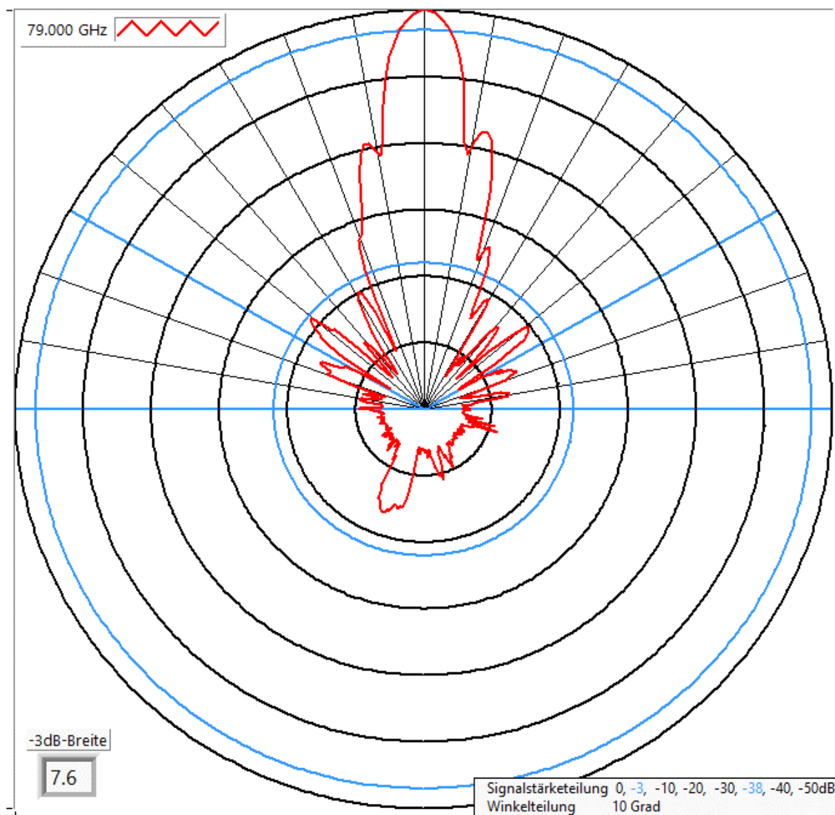
Antenna diagram as provided by the applicant in the H-plane
