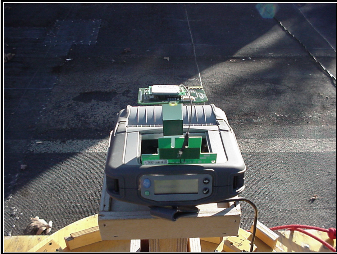
Photograph 1: Radiated Emissions - Front View of CQ17718-G1 Antenna Testing
