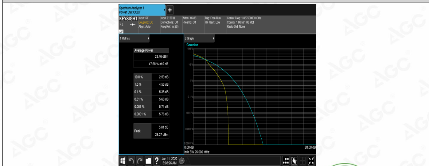
Band2-15MHz-16QAM-18675-1RB#0
