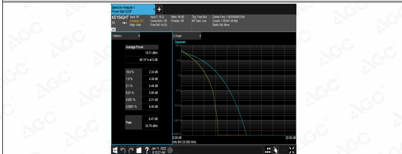
Band2-15MHz-16QAM-18675-1RB#0
