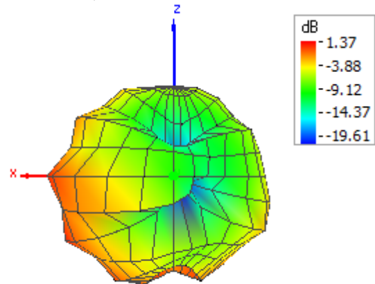
Theta = 90, Phi = 90
