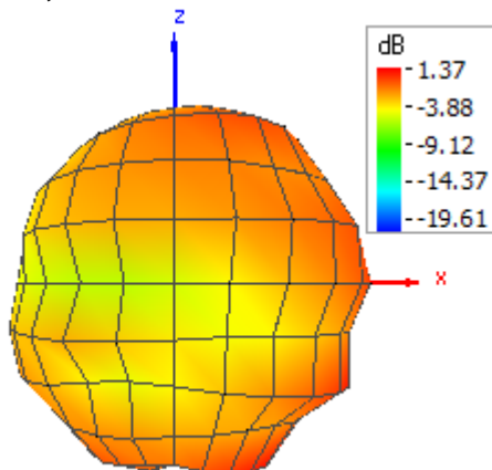
Theta = 90, Phi = 270
