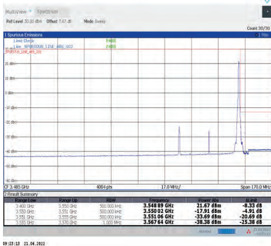
1-N78-3450-3550--30-40-H-5-CP-QPSK-Edge_1RB_Right-1@105-Ant1-PASS-see graph
