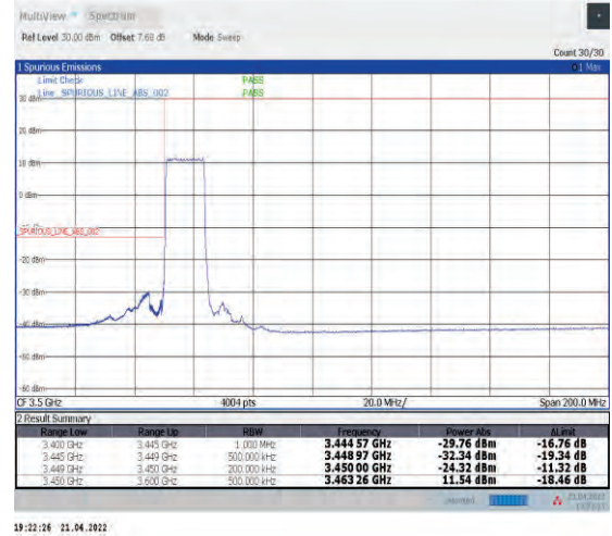
1-N78-3450-3550--30-15-L-3-DFT-PI2BPSK-Outer _Full-36@0-Ant1-PASS-see graph
