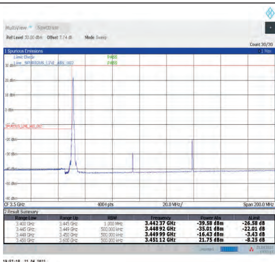
1-N78-3450-3550--30-90-L-1-DFT-PI2BPSK-Edge_1R_B_Left-1@0-Ant1-PASS-see graph
