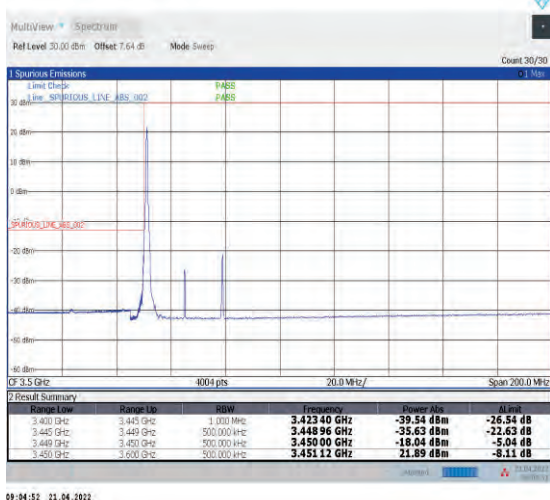
1-N78-3450-3550--30-30-L-4-CP-QPSK-Edge_1RB_L_eff-1@0-Ant1-PASS-see graph
