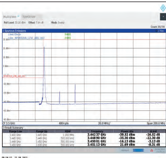
1-N78-3450-3550--30-40-L-1-DFT-PI2BPSK-Edge_1R_B_Left-1@0-Ant1-PASS-see graph
