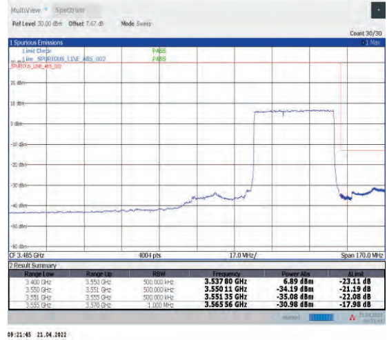
1-N78-3450-3550--30-40-H-3-DFT-PI2BPSK-Outer_Full-100@0-Ant1-PASS-see graph
