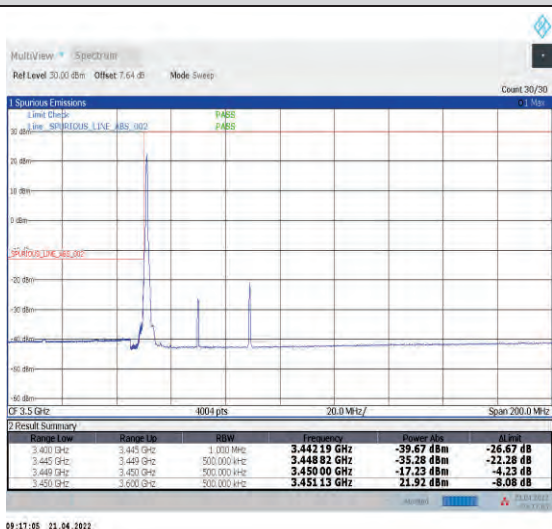
1-N78-3450-3550--30-40-L-4-CP-QPSK-Edge_1RB_L_eff-1@0-Ant1-PASS-see graph
