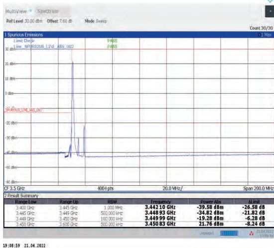
1-N78-3450-3550--30-10-L-1-DFT-PI2BPSK-Edge_1R B_Left-1@0-Ant1-PASS-see graph
