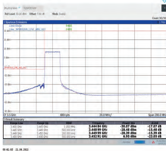
1-N78-3450-3550--30-20-L-6-CP-QPSK-Outer_Ful l-51@0-Ant1-PASS-see graph
