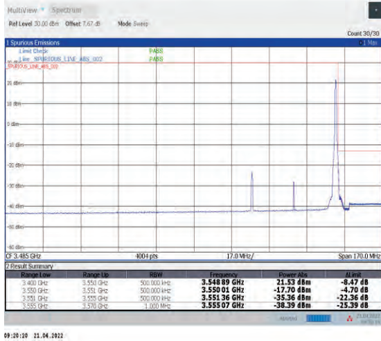
1-N78-3450-3550--30-40-H-2-DFT-PI2BPSK-Edge_1R_B_Right-1@105-Ant1-PASS-see graph
