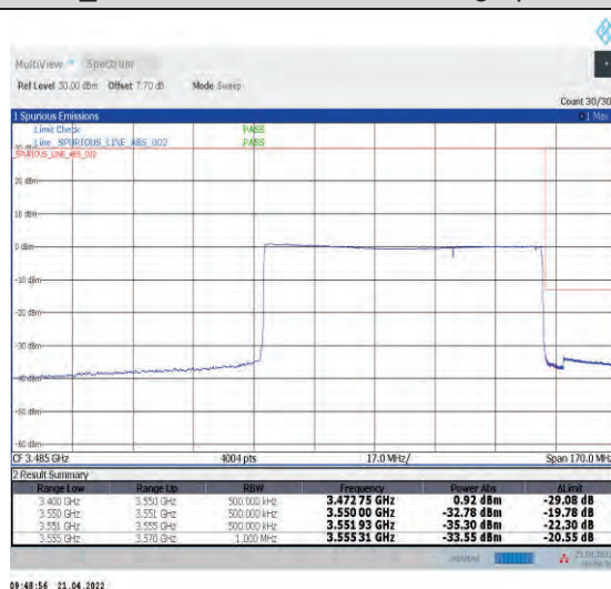
1-N78-3450-3550--30-80-H-6-CP-QPSK-Outer_Fu ll-217@0-Ant1-PASS-see graph
