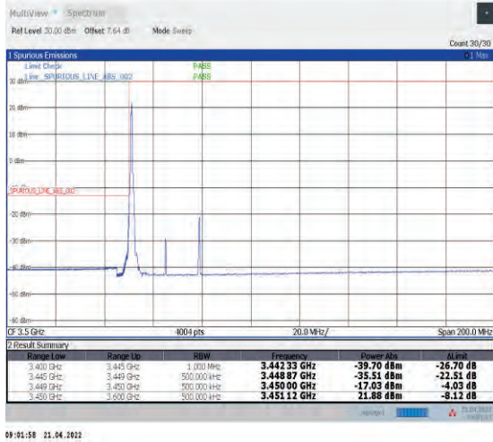
1-N78-3450-3550--30-30-L-1-DFT-PI2BPSK-Edge_1R_B_Left-1@0-Ant1-PASS-see graph
