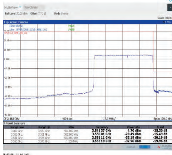
1-N78-3450-3550--30-60-H-3-DFT-PI2BPSK-Outer_Full-162@0-Ant1-PASS-see graph
