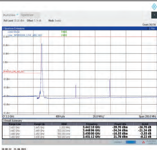
1-N78-3450-3550--30-90-L-4-CP-QPSK-Edge_1RB_L_eff-1@0-Ant1-PASS-see graph
