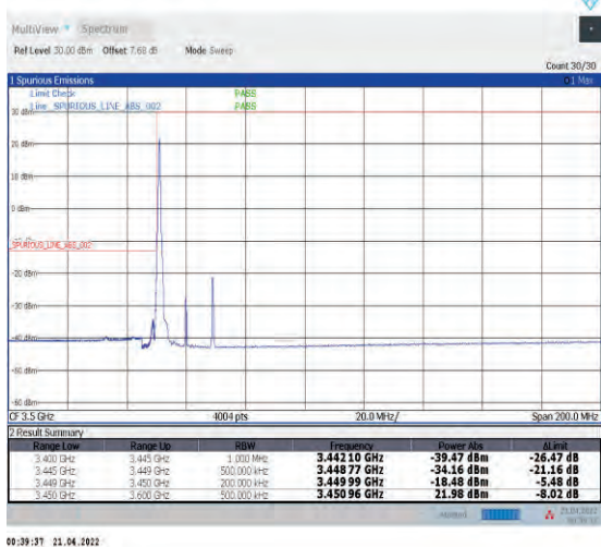
1-N78-3450-3550--30-20-L-4-CP-QPSK-Edge_1RB_L eft-1@0-Ant1-PASS-see graph
