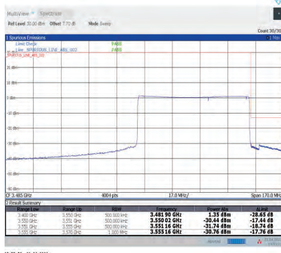
1-N78-3450-3550--30-70-H-6-CP-QPSK-Outer_Full-189@0-Ant1-PASS-see graph
