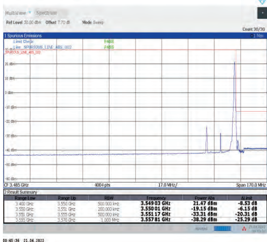
1-N78-3450-3550--30-20-H-5-CP-QPSK-Edge_1RB_R ight-1@50-Ant1-PASS-see graph
