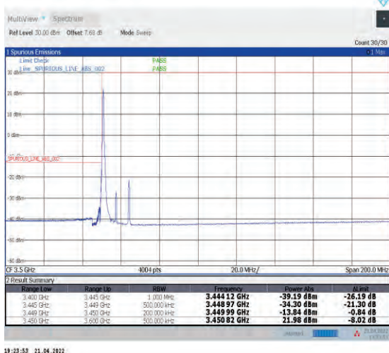
1-N78-3450-3550--30-15-L-4-CP-QPSK-Edge_1RB_L eft-1@0-Ant1-PASS-see graph
