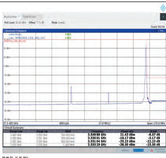
1-N78-3450-3550--30-80-H-2-DFT-PI2BPSK-Edge_1R B_Right-1@216-Ant1-PASS-see graph
