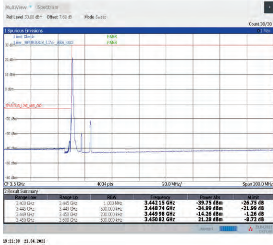
1-N78-3450-3550--30-15-L-1-DFT-PI2BPSK-Edge_1R B_Left-1@0-Ant1-PASS-see graph
