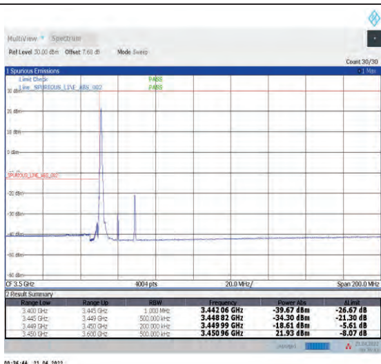
1-N78-3450-3550--30-20-L-1-DFT-PI2BPSK-Edge_1R B_Left-1@0-Ant1-PASS-see graph
