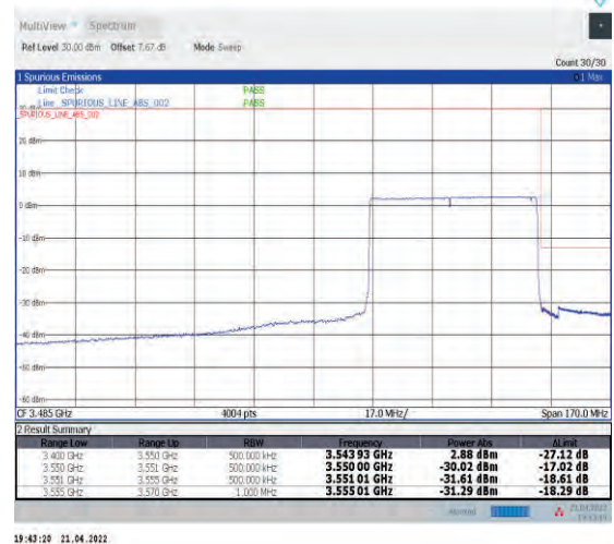
1-N78-3450-3550--30-50-H-6-CP-QPSK-Outer_Full-133@0-Ant1-PASS-see graph
