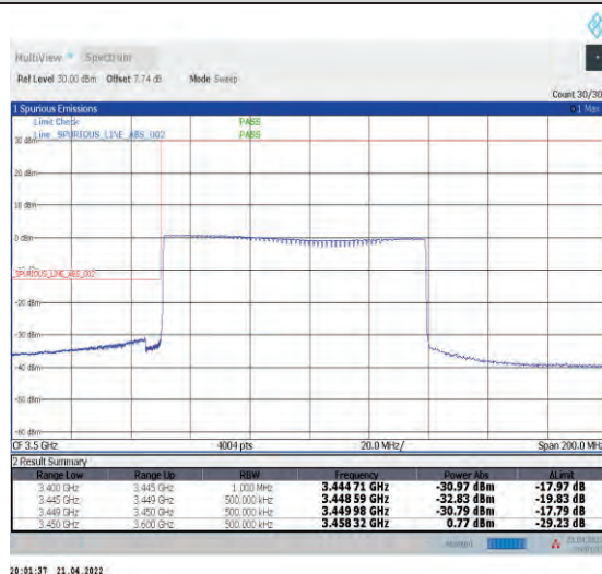
1-N78-3450-3550--30-90-L-6-CP-QPSK-Outer_Ful_I-245@0-Ant1-PASS-see graph
