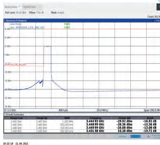
1-N78-3450-3550--30-10-L-6-CP-QPSK-Outer_Ful l-24@0-Ant1-PASS-see graph
