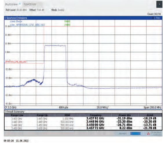
1-N78-3450-3550--30-30-L-3-DFT-PI2BPSK-Outer_Full-75@0-Ant1-PASS-see graph
