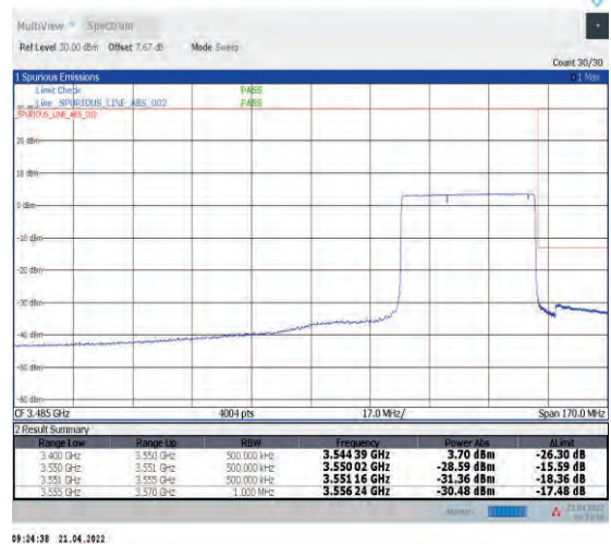
1-N78-3450-3550--30-40-H-6-CP-QPSK-Outer_Full-106@0-Ant1-PASS-see graph
