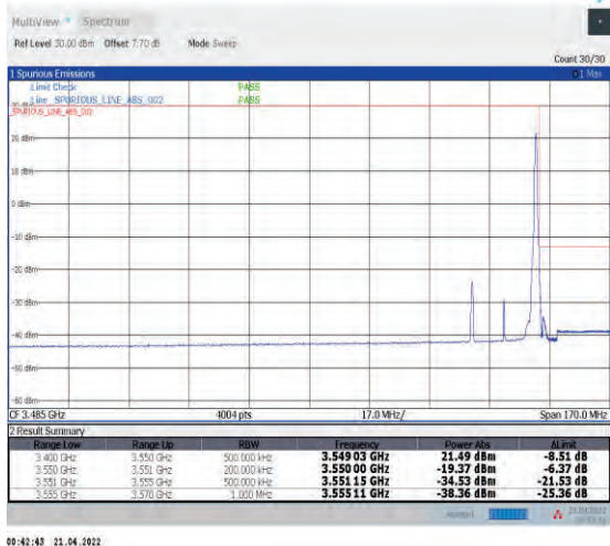
1-N78-3450-3550--30-20-H-2-DFT-PI2BPSK-Edge_1R B_Right-1@50-Ant1-PASS-see graph
