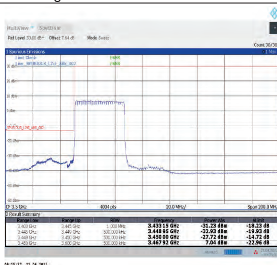
1-N78-3450-3550--30-40-L-3-DFT-PI2BPSK-Outer_Full-100@0-Ant1-PASS-see graph
