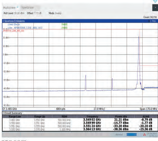
1-N78-3450-3550--30-60-H-5-CP-QPSK-Edge_1RB_Right-1@161-Ant1-PASS-see graph
