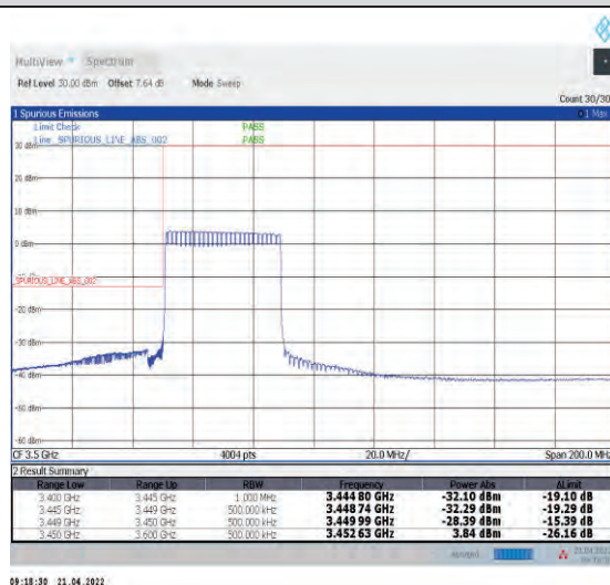
1-N78-3450-3550--30-40-L-6-CP-QPSK-Outer_Ful_I-106@0-Ant1-PASS-see graph
