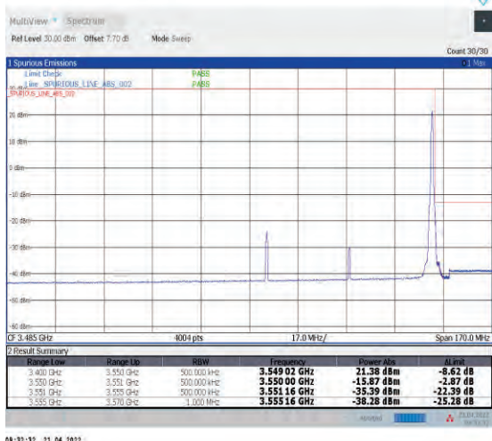
1-N78-3450-3550--30-60-H-2-DFT-PI2BPSK-Edge_1R_B_Right-1@161-Ant1-PASS-see graph
