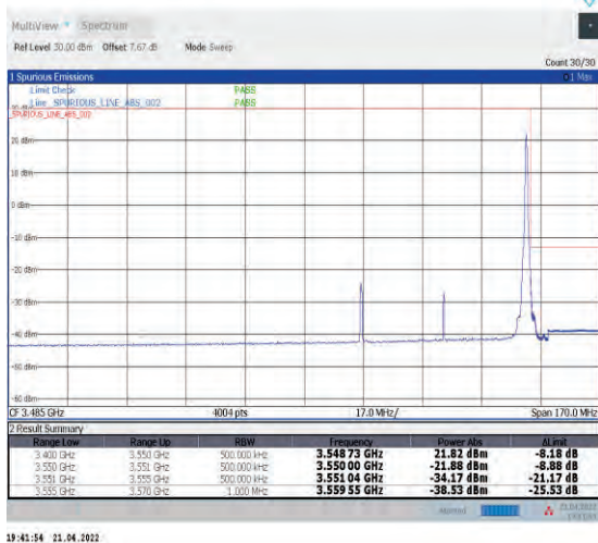
1-N78-3450-3550--30-50-H-5-CP-QPSK-Edge_1RB_Right-1@132-Ant1-PASS-see graph
