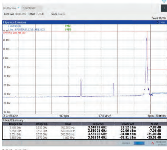
1-N78-3450-3550--30-70-H-5-CP-QPSK-Edge_1RB_Right-1@188-Ant1-PASS-see graph
