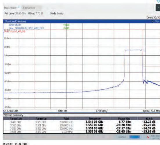
1-N78-3450-3550--30-20-H-6-CP-QPSK-Outer_Fu ll-51@0-Ant1-PASS-see graph
