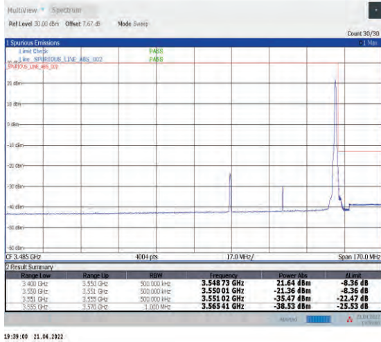
1-N78-3450-3550--30-50-H-2-DFT-PI2BPSK-Edge_1R_B_Right-1@132-Ant1-PASS-see graph
