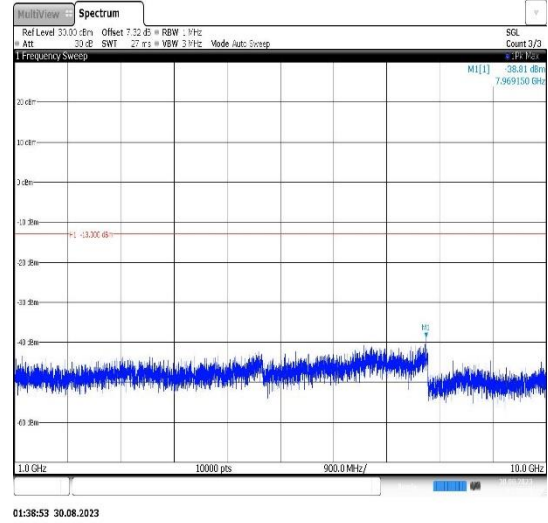
Band5-5MHz-16QAM-20525-1RB#0- Range2:1000~10000MHz
