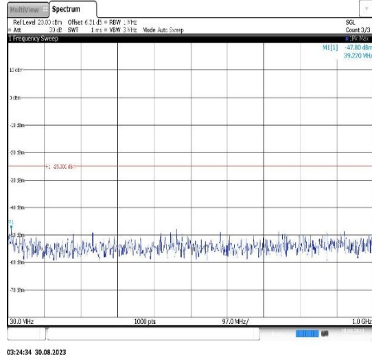
Band7-20MHz-16QAM-21100-1RB#0- Range1:30~1000MHz
