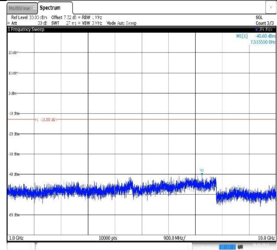
Band12-5MHz-16QAM-23035-1RB#0- Range2:1000~10000MHz
