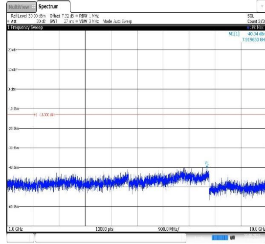
Band5-10MHz-16QAM-20450-1RB#0- Range2:1000~10000MHz
