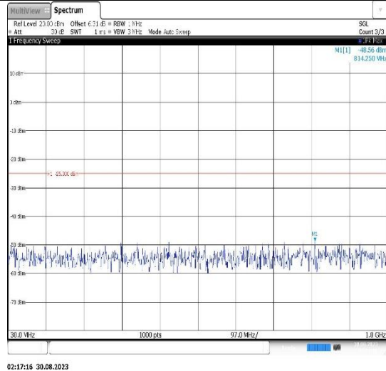
Band7-5MHz-QPSK-21425-1RB#0- Range1:30~1000MHz
