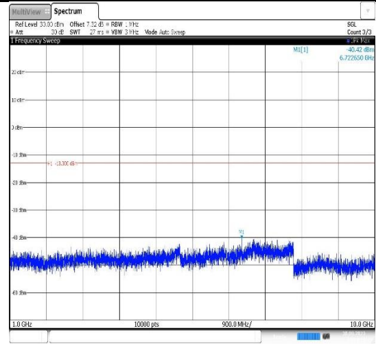
Band12-3MHz-16QAM-23025-1RB#0- Range2:1000~10000MHz
