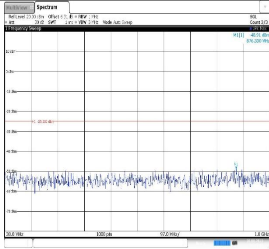
Band7-5MHz-16QAM-21100-1RB#0- Range1:30~1000MHz
