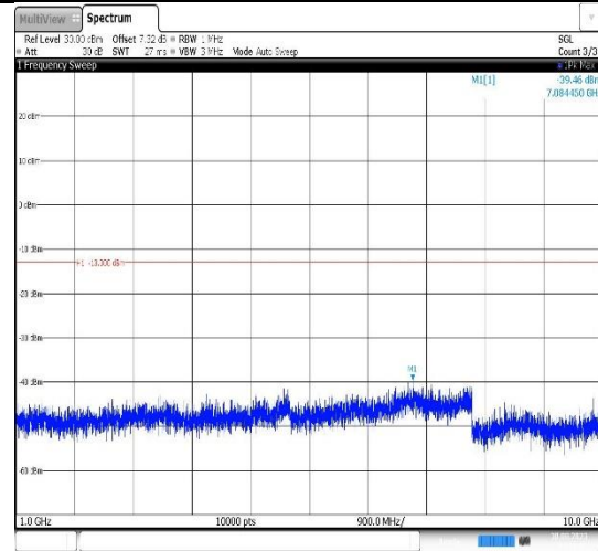
Band12-1.4MHz-16QAM-23017-1RB#0- Range2:1000~10000MHz
