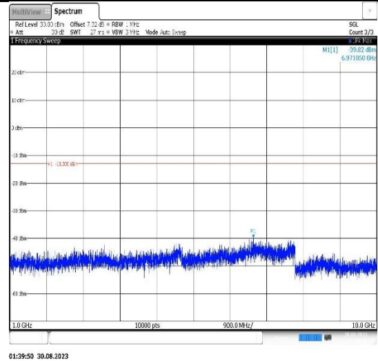
Band5-5MHz-16QAM-20425-1RB#0- Range2:1000~10000MHz
