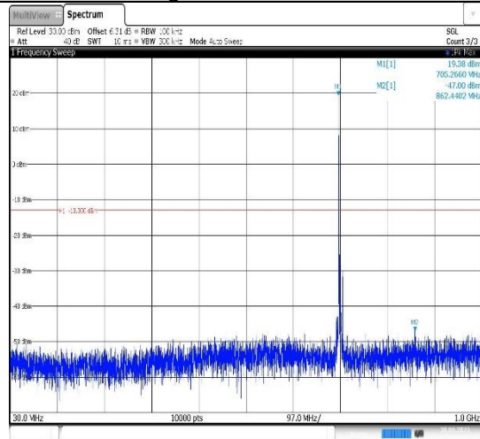
Band12-5MHz-16QAM-23095-1RB#0- Range1:30~1000MHz
