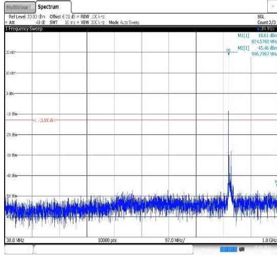
Band5-10MHz-16QAM-20450-1RB#0- Range1:30~1000MHz
