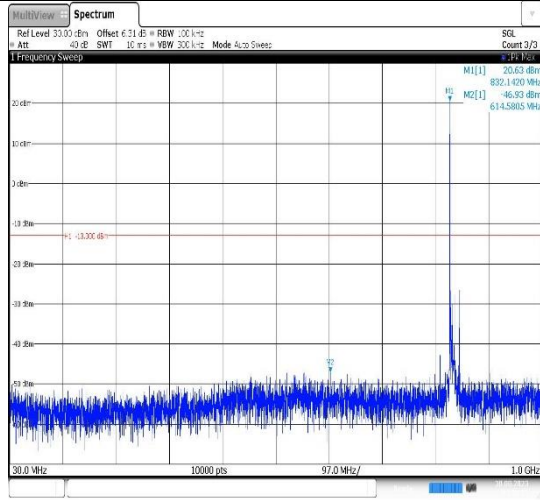
Band5-10MHz-16QAM-20600-1RB#0- Range1:30~1000MHz
