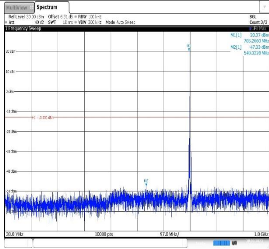
Band12-5MHz-QPSK-23095-1RB#0- Range1:30~1000MHz
