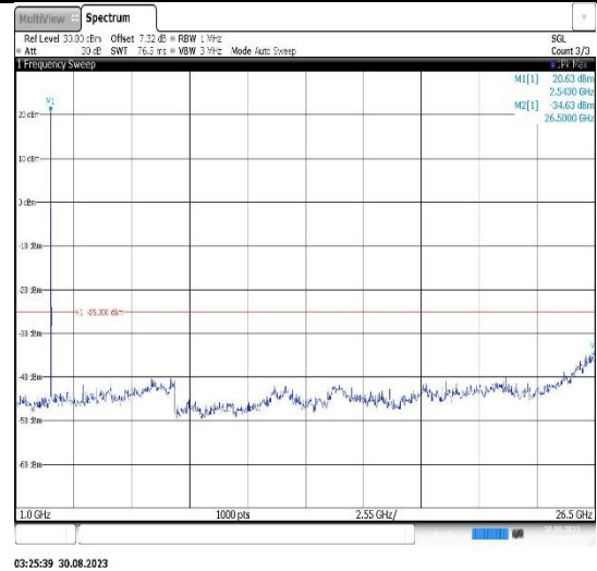
Band7-20MHz-16QAM-20850-1RB#0- Range2:1000~26500MHz
