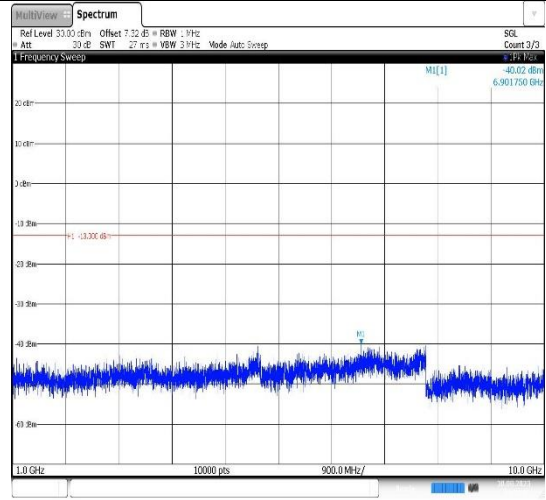
Band12-5MHz-QPSK-23095-1RB#0- Range2:1000~10000MHz
