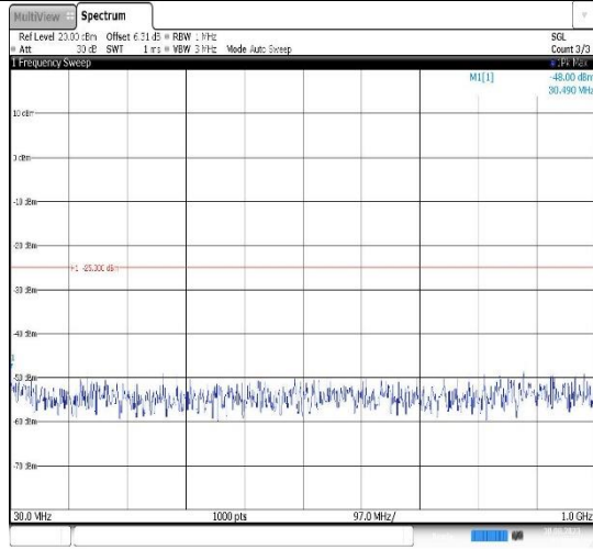
Band7-10MHz-16QAM-21100-1RB#0- Range1:30~1000MHz
