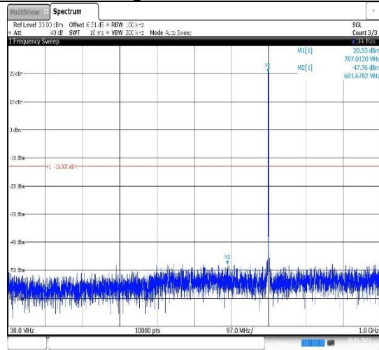
Band12-1.4MHz-16QAM-23095-1RB#0- Range1:30~1000MHz
