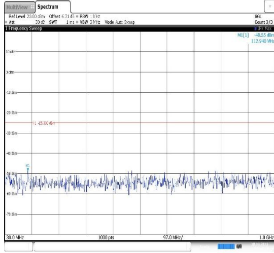
Band7-5MHz-16QAM-20775-1RB#0- Range1:30~1000MHz
