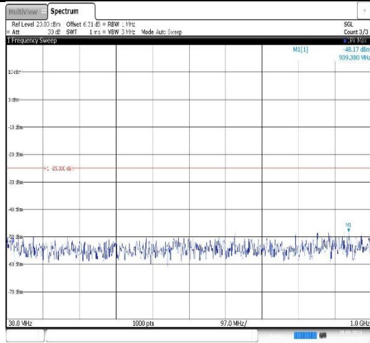
Band7-10MHz-16QAM-20800-1RB#0- Range1:30~1000MHz
