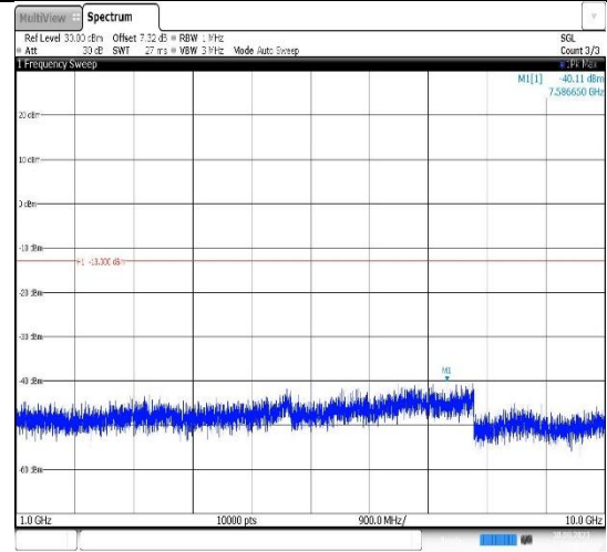
Band12-3MHz-QPSK-23025-1RB#0- Range2:1000~10000MHz
