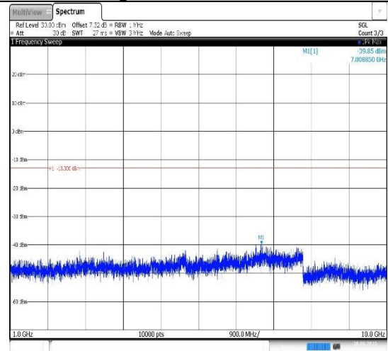
Band12-5MHz-16QAM-23095-1RB#0- Range2:1000~10000MHz
