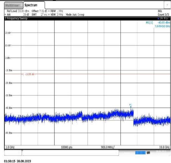
Band5-10MHz-QPSK-20600-1RB#0- Range2:1000~10000MHz
