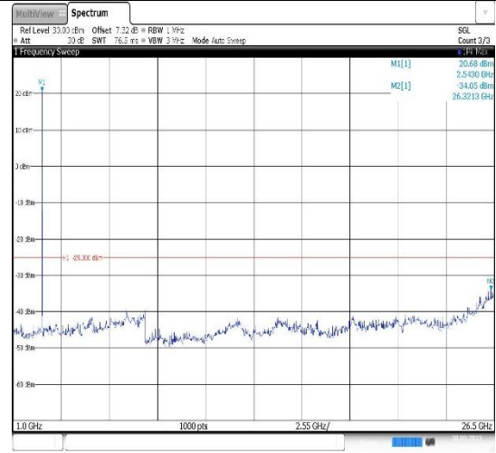
Band7-5MHz-16QAM-21100-1RB#0- Range2:1000~26500MHz
