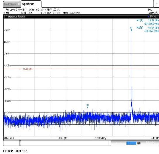
Band5-5MHz-16QAM-20525-1RB#0- Range1:30~1000MHz
