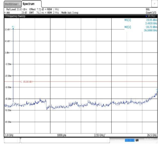
Band7-15MHz-16QAM-20825-1RB#0- Range2:1000~26500MHz
