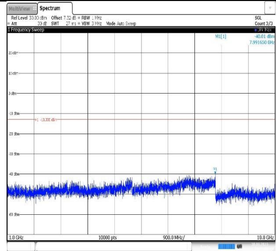
Band12-5MHz-16QAM-23035-1RB#0- Range2:1000~10000MHz
