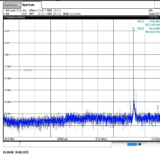
Band5-10MHz-QPSK-20600-1RB#0- Range1:30~1000MHz
