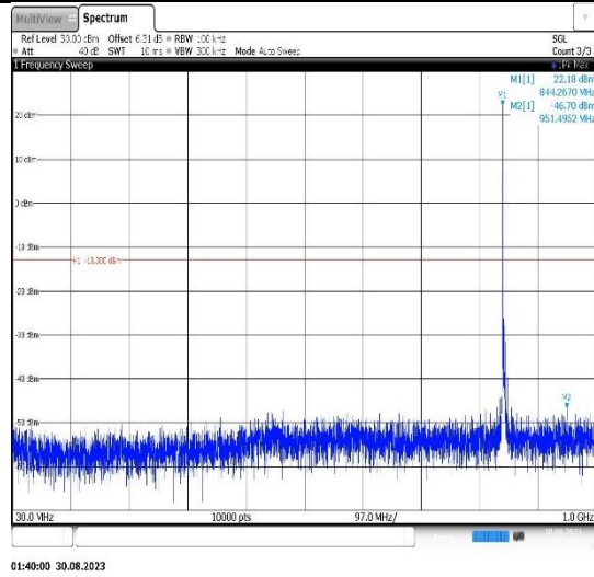
Band5-10MHz-QPSK-20450-1RB#0- Range1:30~1000MHz
