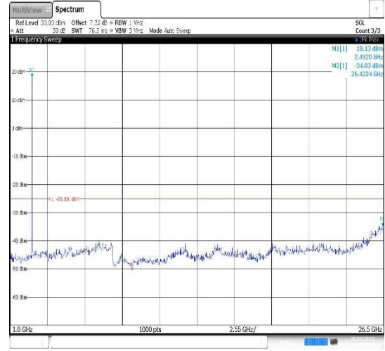
Band7-5MHz-16QAM-20775-1RB#0- Range2:1000~26500MHz
