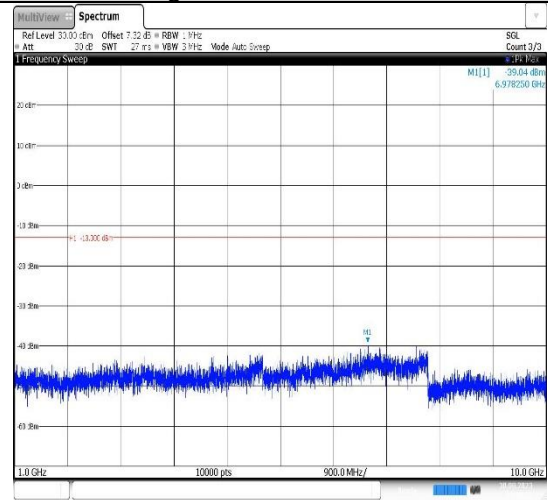
Band12-3MHz-QPSK-23095-1RB#0- Range2:1000~10000MHz
