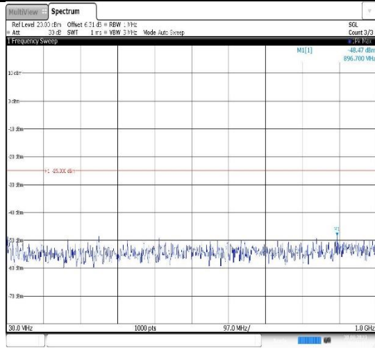
Band7-15MHz-16QAM-20825-1RB#0- Range1:30~1000MHz
