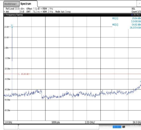
Band7-10MHz-16QAM-21100-1RB#0- Range2:1000~26500MHz
