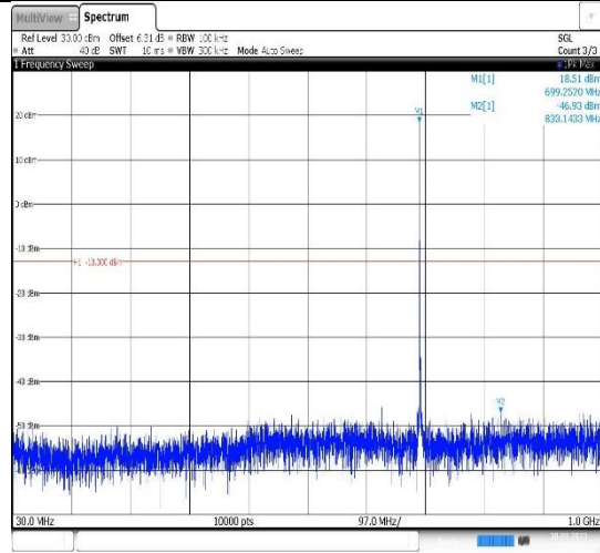
Band12-1.4MHz-16QAM-23017-1RB#0- Range1:30~1000MHz
