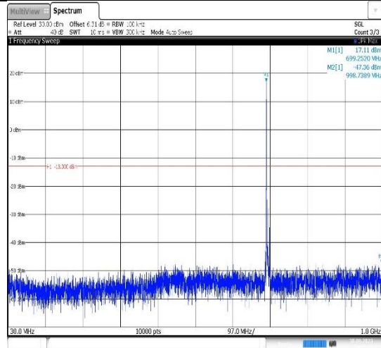
Band12-5MHz-16QAM-23035-1RB#0- Range1:30~1000MHz
