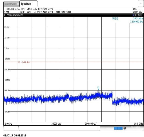
Band12-1.4MHz-QPSK-23173-1RB#0- Range2:1000~10000MHz
