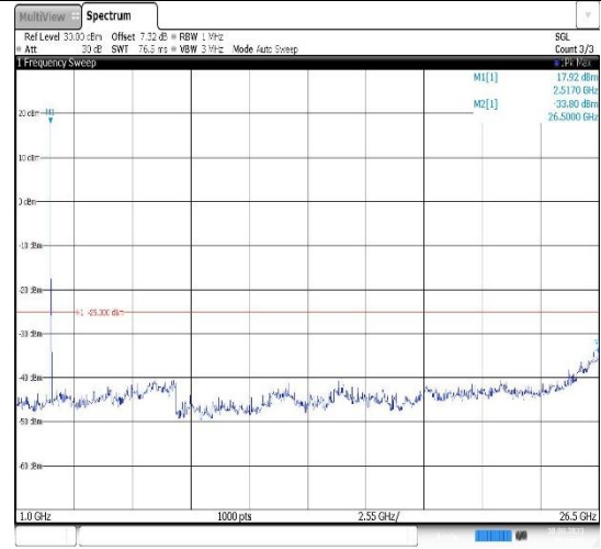
Band7-15MHz-16QAM-21100-1RB#0- Range2:1000~26500MHz
