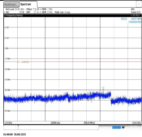
Band5-10MHz-QPSK-20450-1RB#0- Range2:1000~10000MHz
