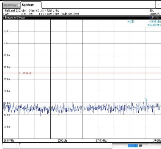
Band7-15MHz-QPSK-20825-1RB#0- Range1:30~1000MHz
