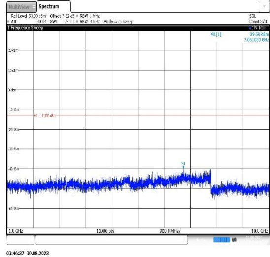
Band12-1.4MHz-QPSK-23095-1RB#0- Range2:1000~10000MHz
