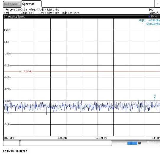
Band7-5MHz-QPSK-21100-1RB#0- Range1:30~1000MHz
