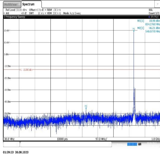
Band5-5MHz-16QAM-20625-1RB#0- Range1:30~1000MHz
