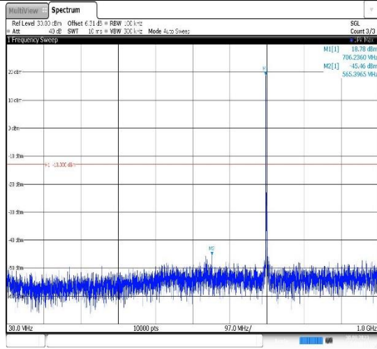
Band12-3MHz-16QAM-23095-1RB#0- Range1:30~1000MHz
