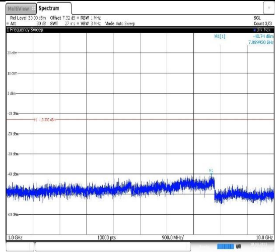
Band12-5MHz-QPSK-23035-1RB#0- Range2:1000~10000MHz
