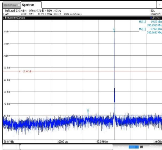
Band12-3MHz-QPSK-23095-1RB#0- Range1:30~1000MHz
