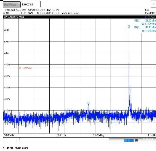
Band5-10MHz-QPSK-20525-1RB#0- Range1:30~1000MHz
