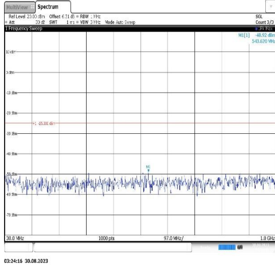
Band7-20MHz-QPSK-21100-1RB#0- Range1:30~1000MHz
