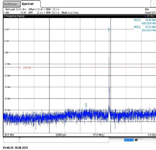
Band12-1.4MHz-QPSK-23095-1RB#0- Range1:30~1000MHz
