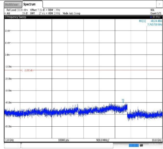
Band12-3MHz-16QAM-23095-1RB#0- Range2:1000~10000MHz
