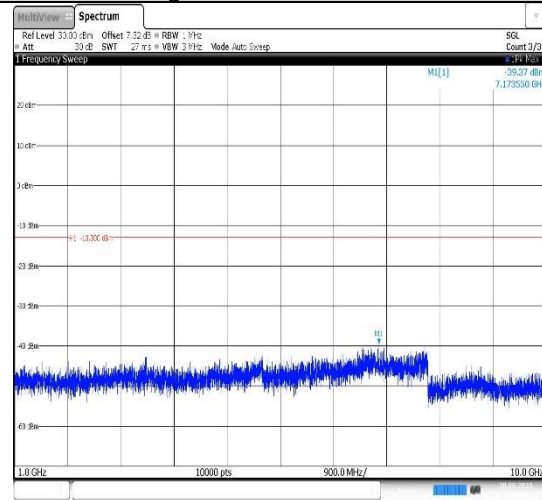
Band12-1.4MHz-16QAM-23095-1RB#0- Range2:1000~10000MHz
