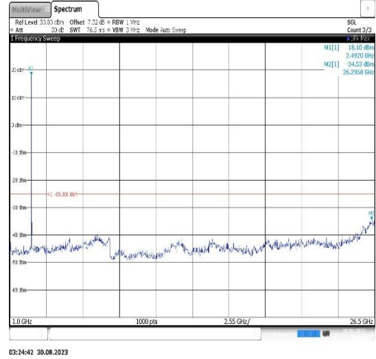
Band7-20MHz-16QAM-21100-1RB#0- Range2:1000~26500MHz
