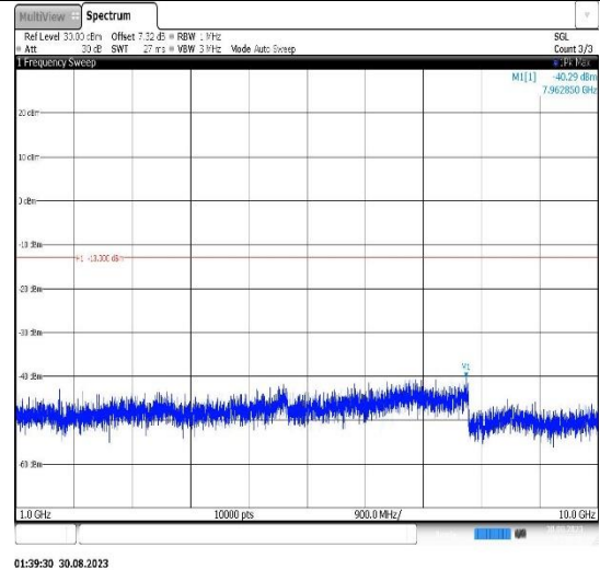
Band5-5MHz-16QAM-20625-1RB#0- Range2:1000~10000MHz
