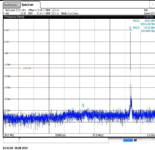
Band7-5MHz-QPSK-20775-1RB#0- Range1:30~1000MHz
