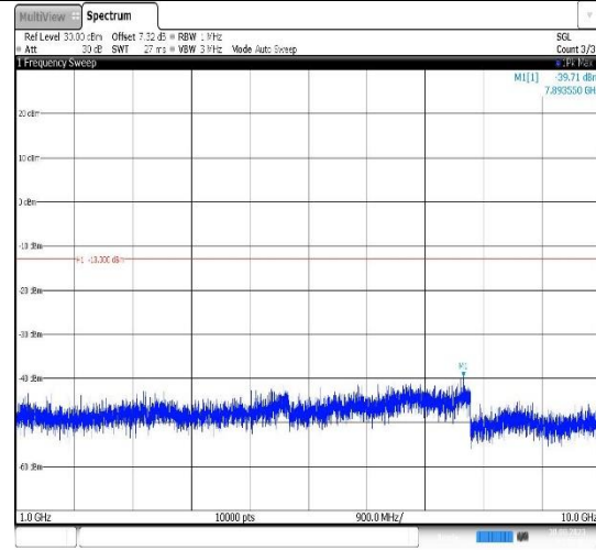
Band5-10MHz-16QAM-20600-1RB#0- Range2:1000~10000MHz
