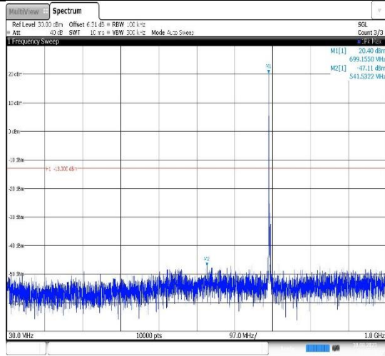
Band12-3MHz-QPSK-23025-1RB#0- Range1:30~1000MHz
