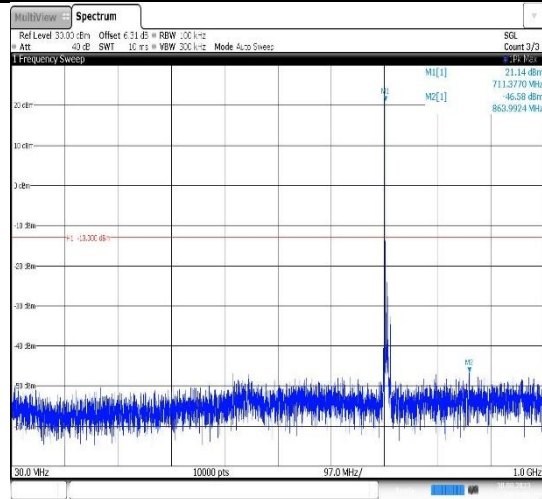
Band12-5MHz-16QAM-23035-1RB#0- Range1:30~1000MHz
