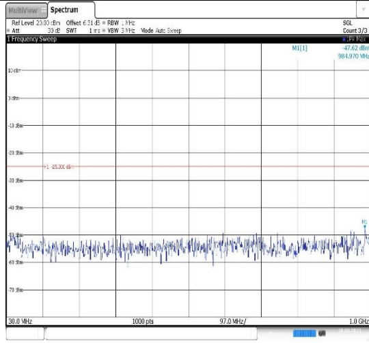
Band7-10MHz-QPSK-21100-1RB#0- Range1:30~1000MHz
