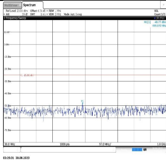
Band7-20MHz-16QAM-20850-1RB#0- Range1:30~1000MHz
