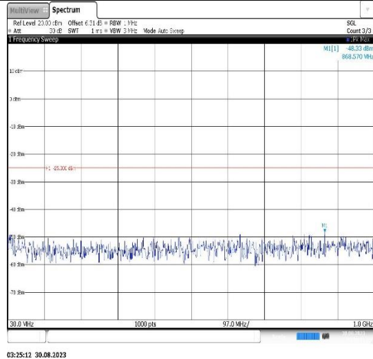
Band7-20MHz-16QAM-21350-1RB#0- Range1:30~1000MHz
