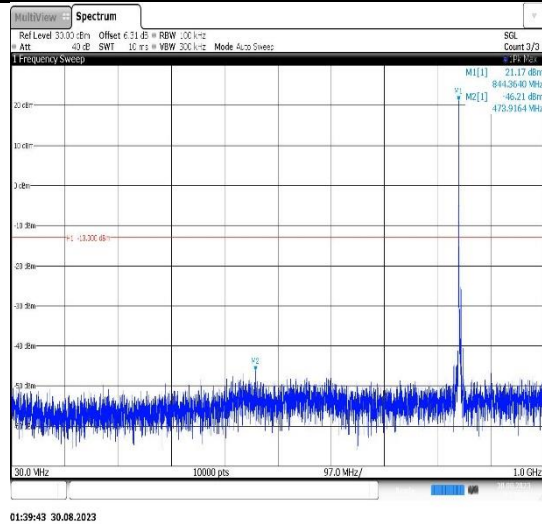
Band5-5MHz-16QAM-20425-1RB#0- Range1:30~1000MHz
