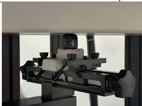
Left Side of EUT with 0cm Gap
