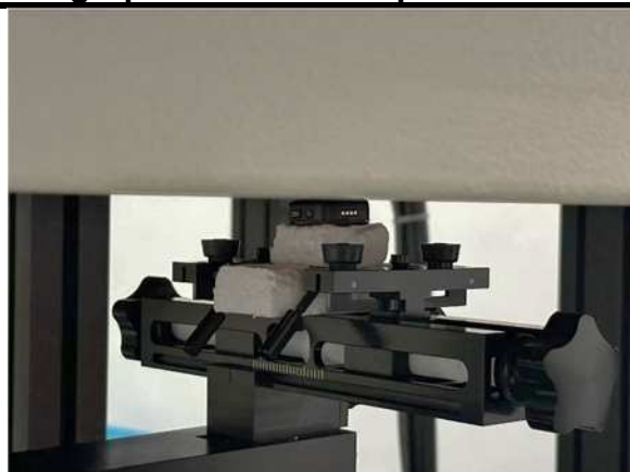
Front Face of EUT with 0cm Gap
