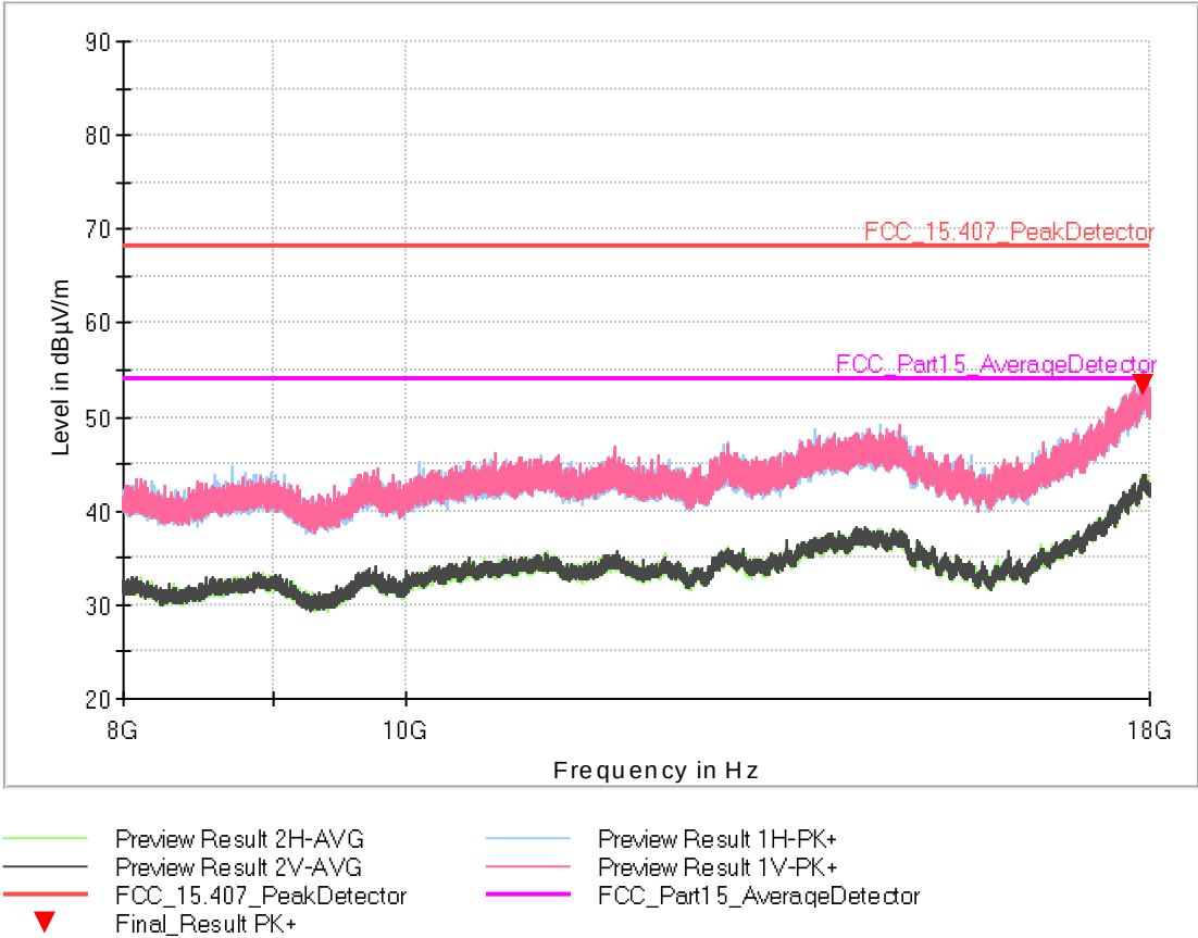
Fig. 361: Low Channel. Frequency range: 8 GHz – 18 GHz
