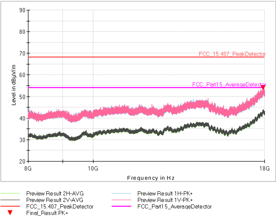
Fig. 362: High Channel. Frequency range: 8 GHz – 18 GHz
