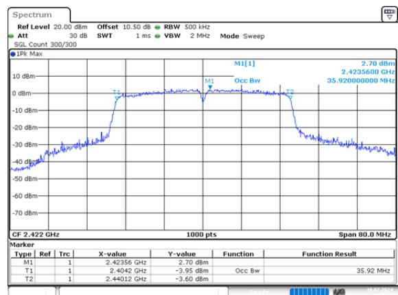
n40_2422MHz_Chain 0 35.920MHz
