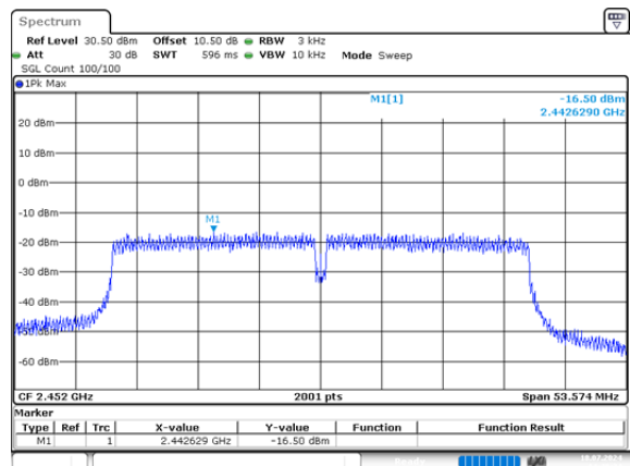
n40_2452MHz_Chain 0 -16.50dBm/3kHz
