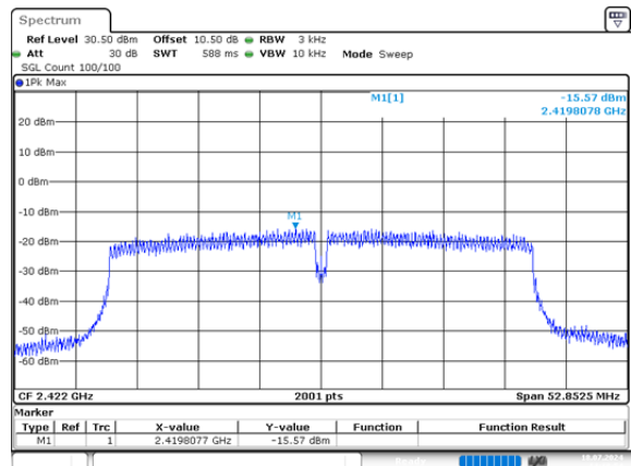
n40_2422MHz_Chain 0 -15.57dBm/3kHz
