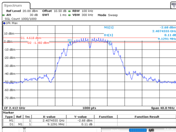
b_2412MHz_Chain 0 9.129MHz
