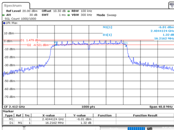
n20_2412MHz_Chain 0 16.216MHz
