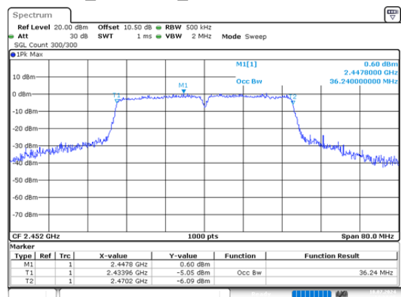
n40_2452MHz_Chain 0 36.240MHz
