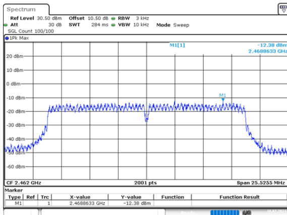
n20_2462MHz_Chain 0 -12.38dBm/3kHz
