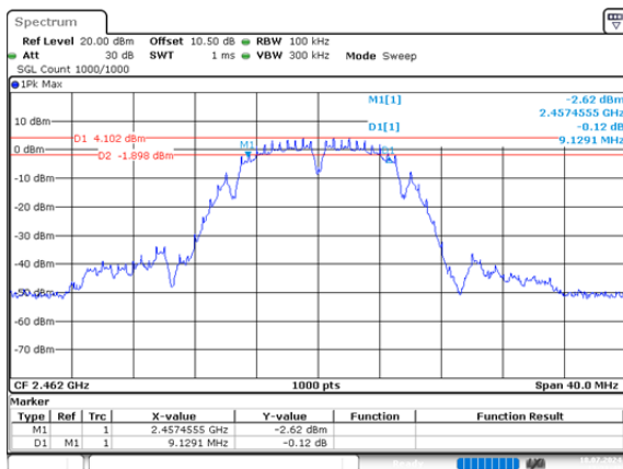
b_2462MHz_Chain 0 9.129MHz
