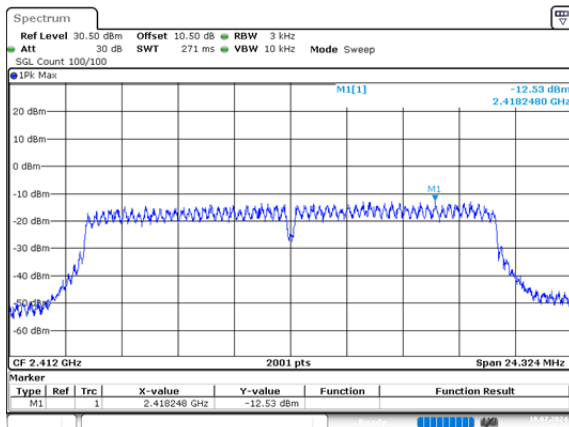
n20_2412MHz_Chain 0 -12.53dBm/3kHz
