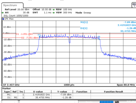
n40_2437MHz_Chain 0 35.475MHz
