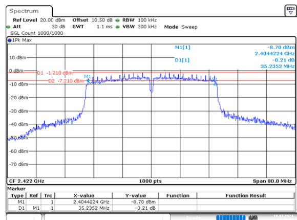
n40_2422MHz_Chain 0 35.235MHz
