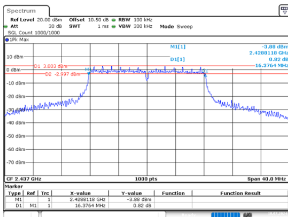
g_2437MHz_Chain 0 16.376MHz
