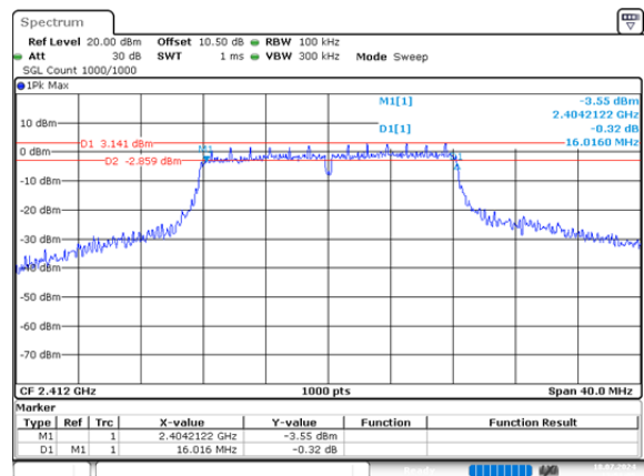
g_2412MHz_Chain 0 16.016MHz
