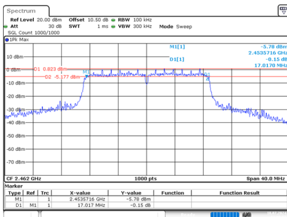
n20_2462MHz_Chain 0 17.017MHz
