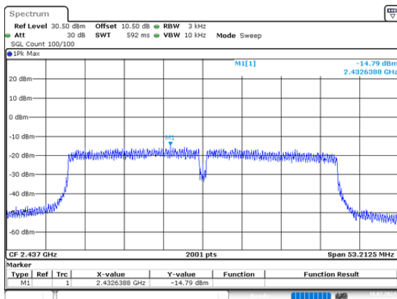
n40_2437MHz_Chain 0 -14.79dBm/3kHz
