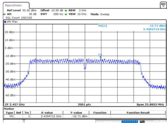
n20_2437MHz_Chain 0 -12.71dBm/3kHz
