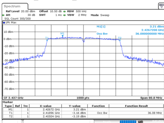
n40_2437MHz_Chain 0 36.080MHz
