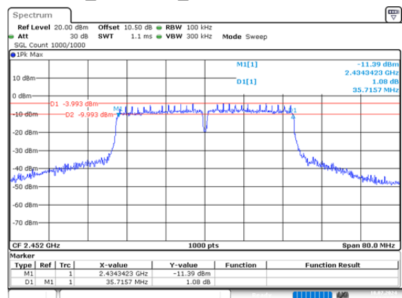
n40_2452MHz_Chain 0 35.716MHz
