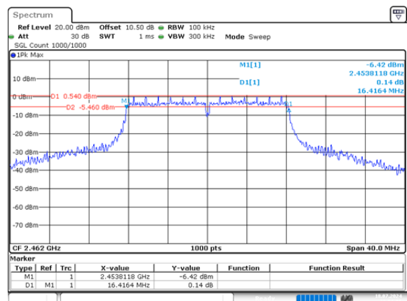
g_2462MHz_Chain 0 16.416MHz
