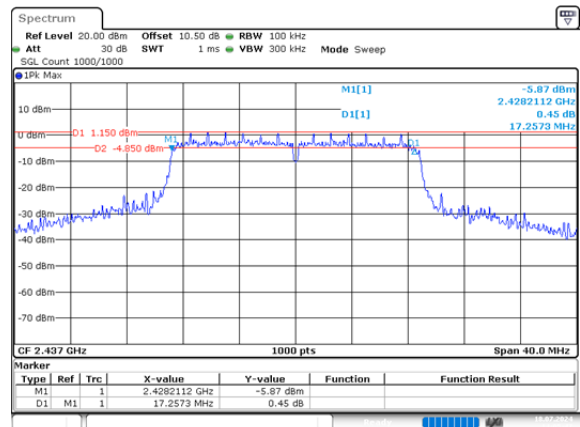
n20_2437MHz_Chain 0 17.257MHz
