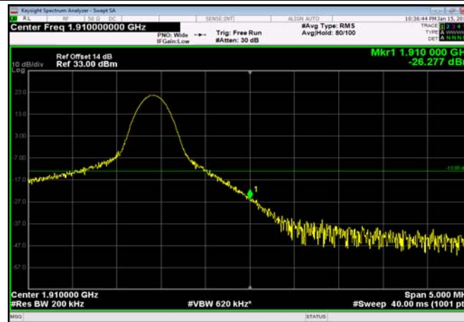
HighRange_FDD02_20MHz_1900_fullRB _High_QPSK
