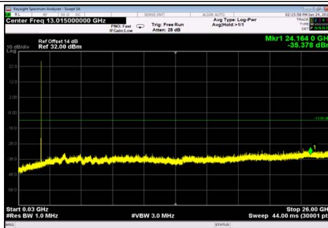
FDD02_MidRange_1.4MHz_30MHz~26GHz
