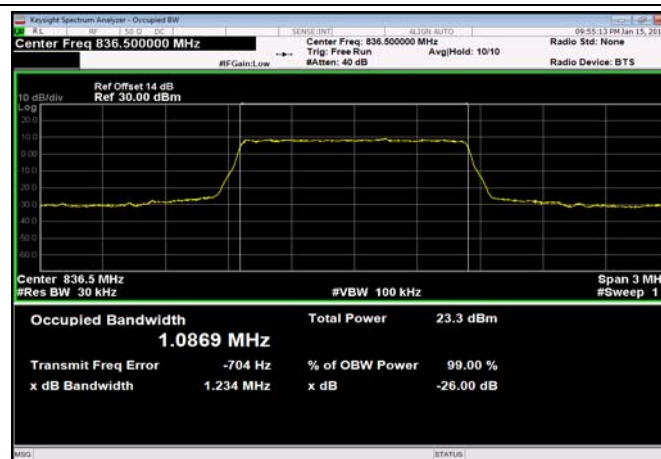
FDD05_MidRange_1.4MHz_836.5MHz _QPSK
