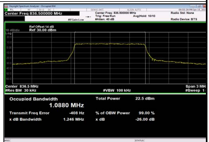
FDD05_MidRange_1.4MHz_836.5MHz _Q16
