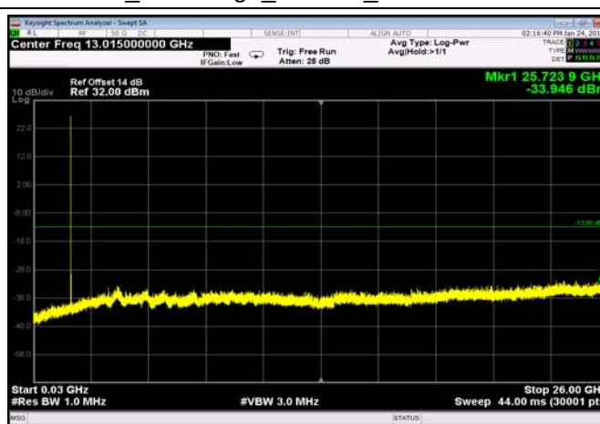
FDD04_LowRange_1.4MHz_30MHz~26GHz
