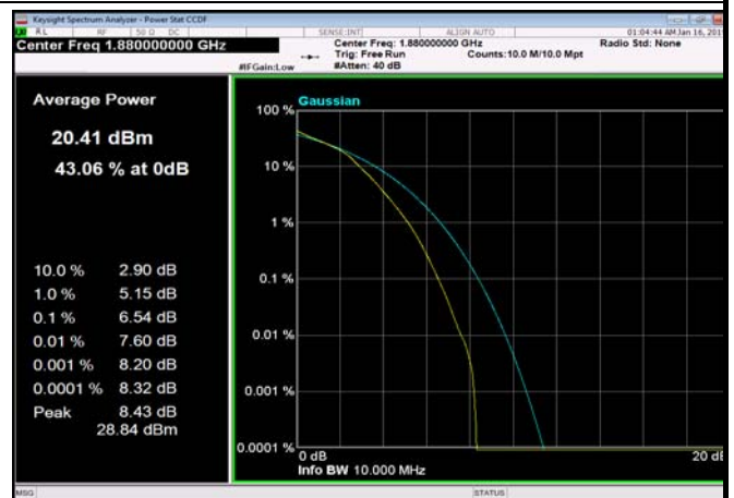
FDD02_10MHz_1880_fullRB_Q16
