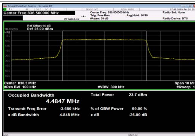
FDD05_MidRange_5_836.5_QPSK
