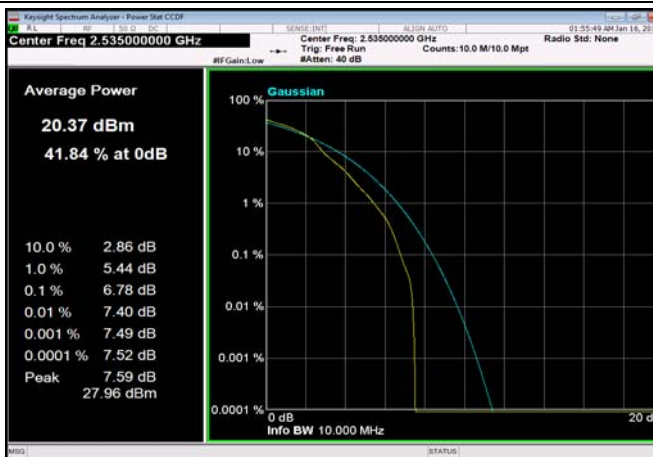
FDD07_10MHz_2560_OneRB_high_Q16
