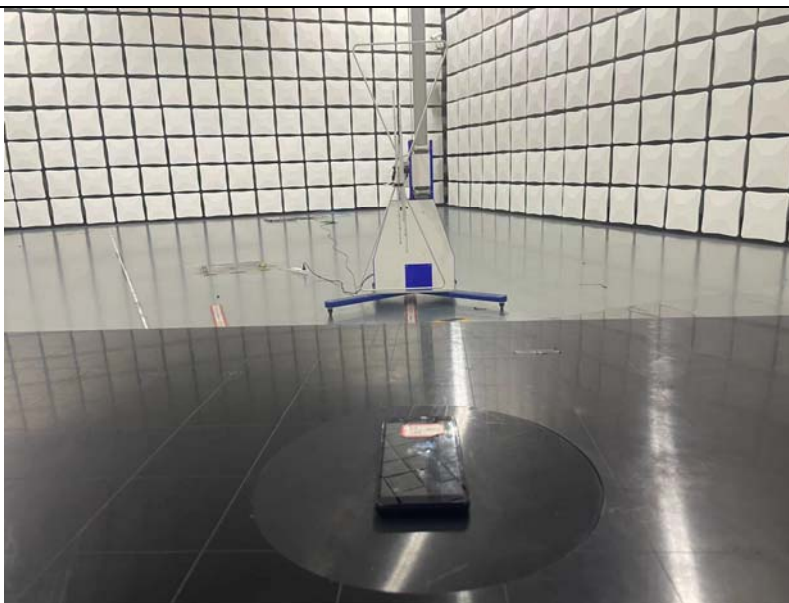
30MHz~1GHz
