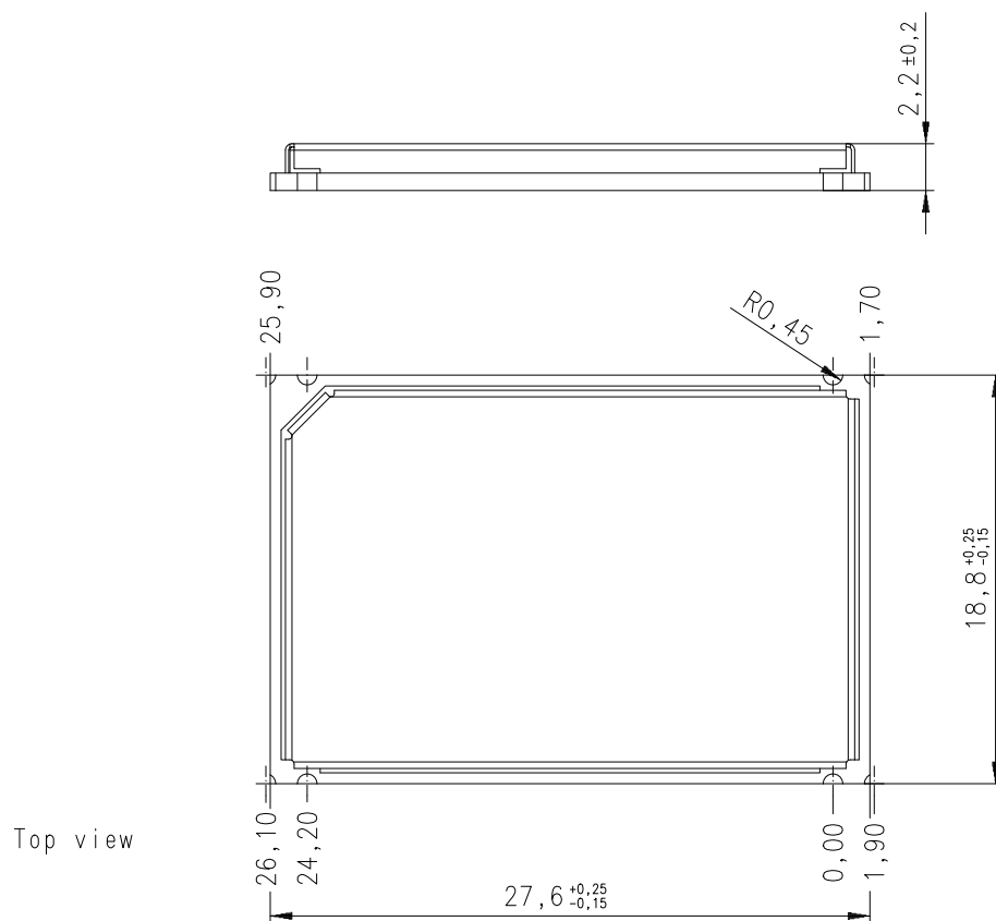
Figure 8: Dimensions of ELS31-V / ELS51-V (all dimensions in mm)
