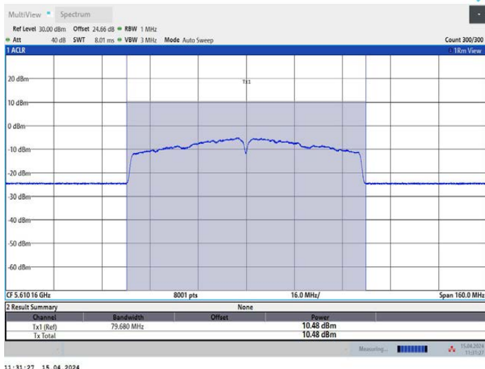
11AC80MIMO Ant2_5610
