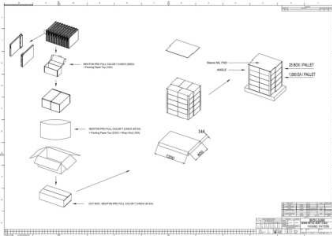
Figure 11. 7.3" Packing-Diagram (1,200 X 800)
