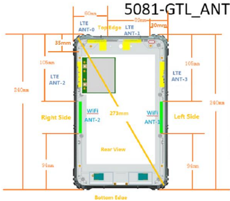
Figure: The location of the antennas
