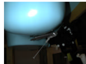
Figure 18. Right Head SAR Test Setup -- Check / Touch Position --
