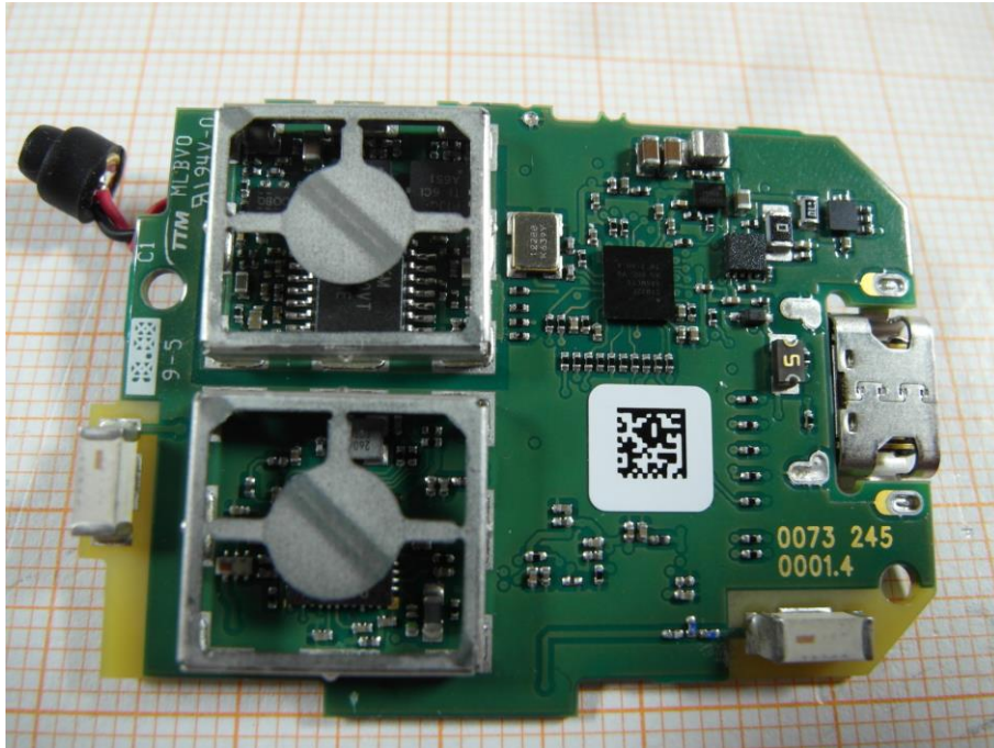
Photo 3: PCB of the EUT (rear view)
