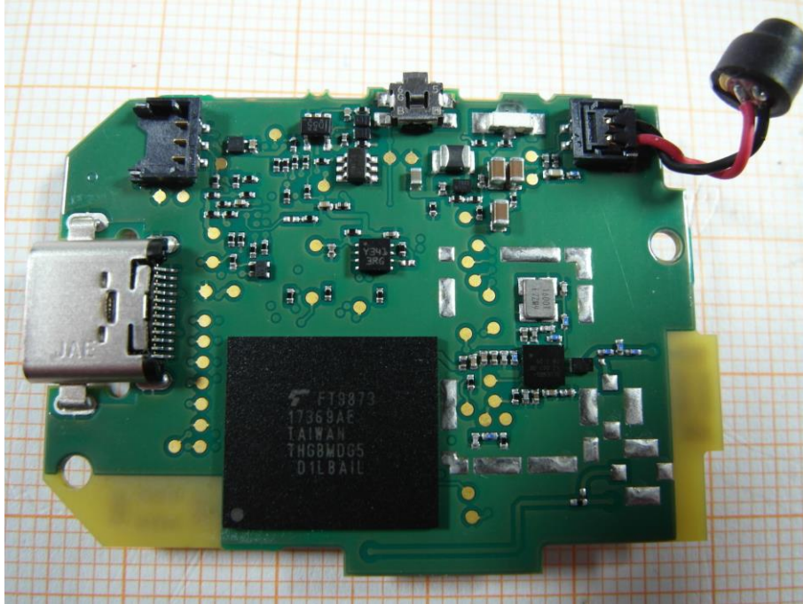
Photo 5: PCB of the EUT (front view)
