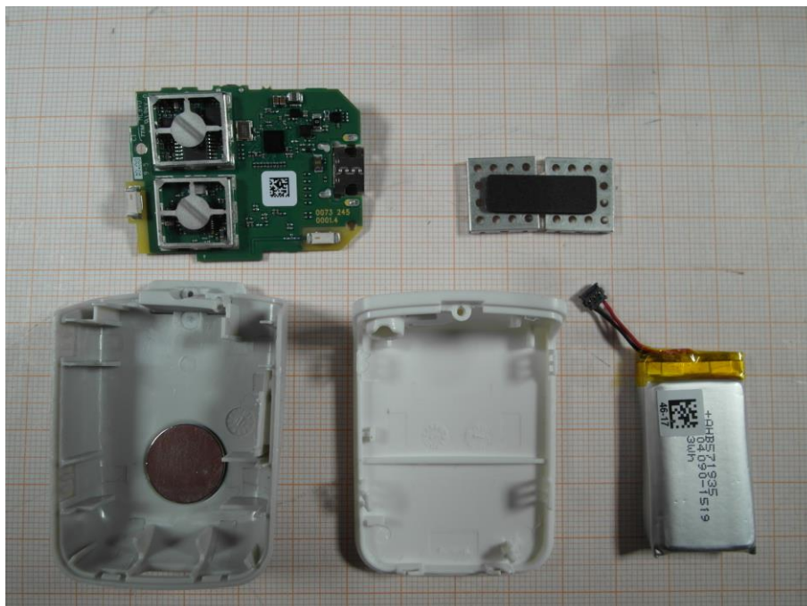
Photo 2: EUT disassembled with battery pack (rear view)
