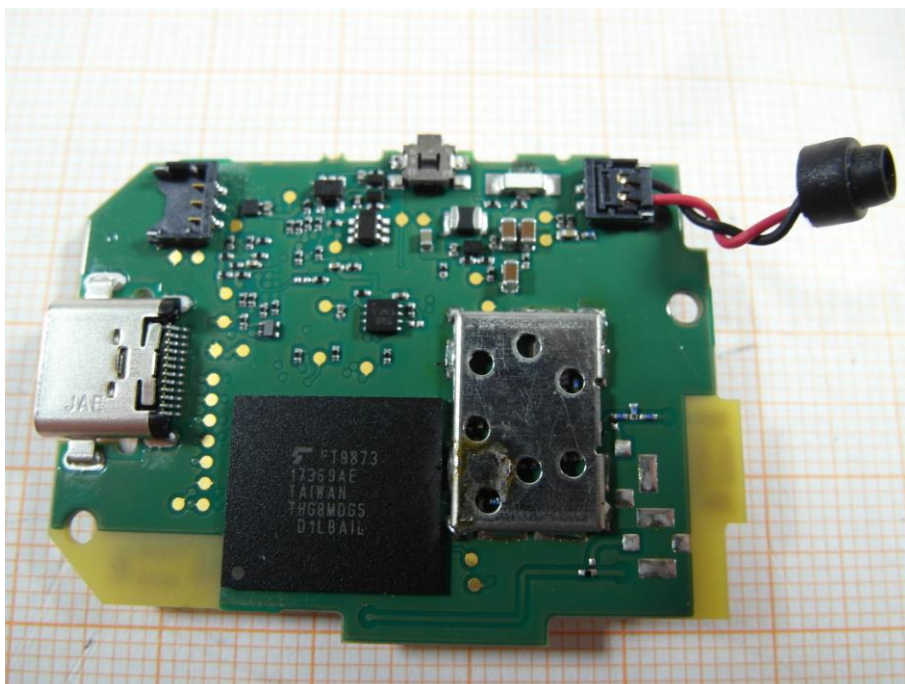
Photo 6: PCB of the EUT (front view)
