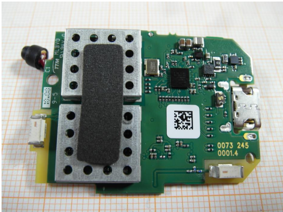
Photo 4: PCB of the EUT (rear view)
