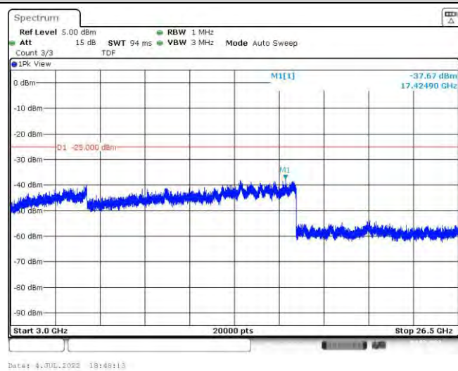
Band41-20MHz-16QAM-41140-100RB#0-Range3:3000~26500MHz
