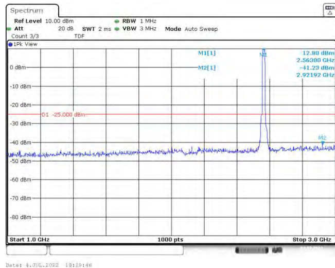
Band41-15MHz-QPSK-40315-75RB#0-Range3:3000~26500MHz
